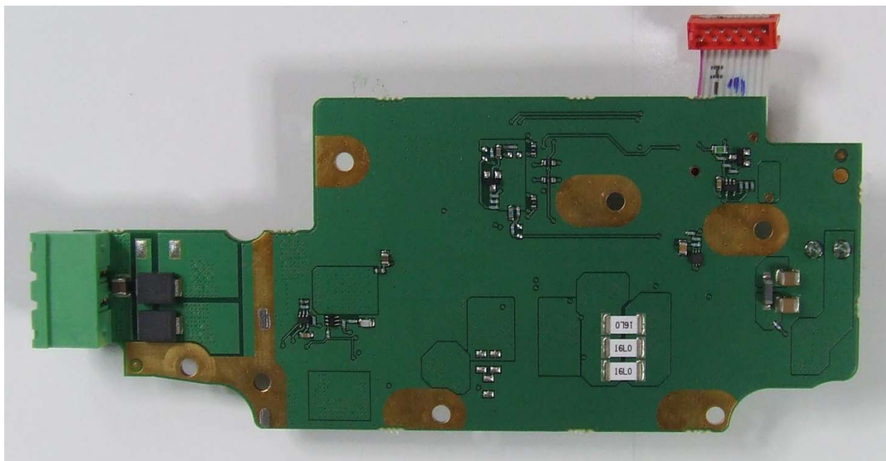
Photograph 09: DC-DC PCB bottom
