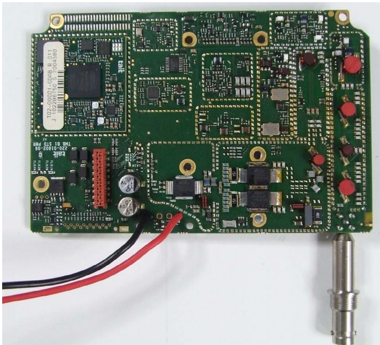
Photograph 05: RF PCB top without shields
