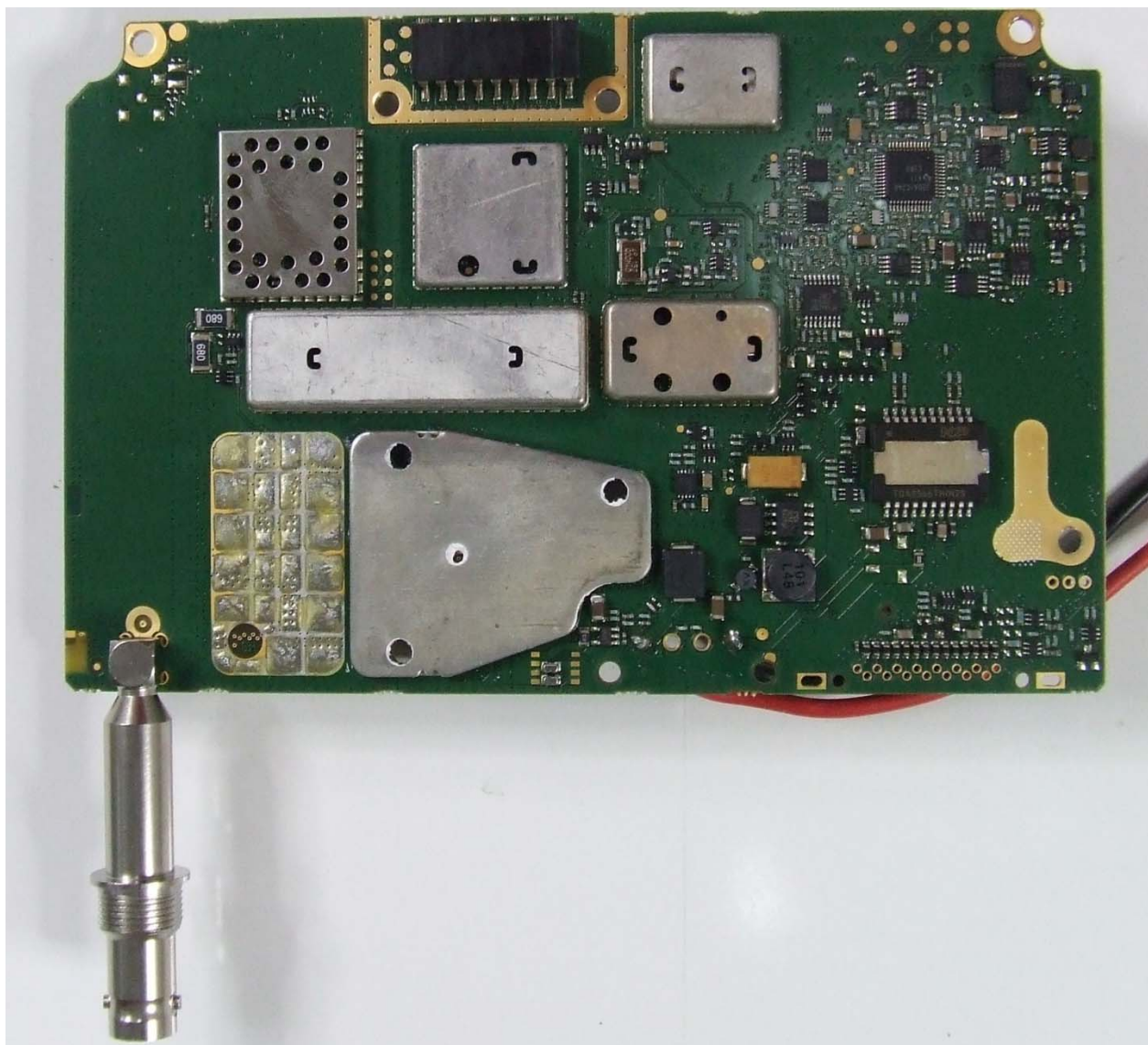
Photograph 06: RF PCB bottom with shields
