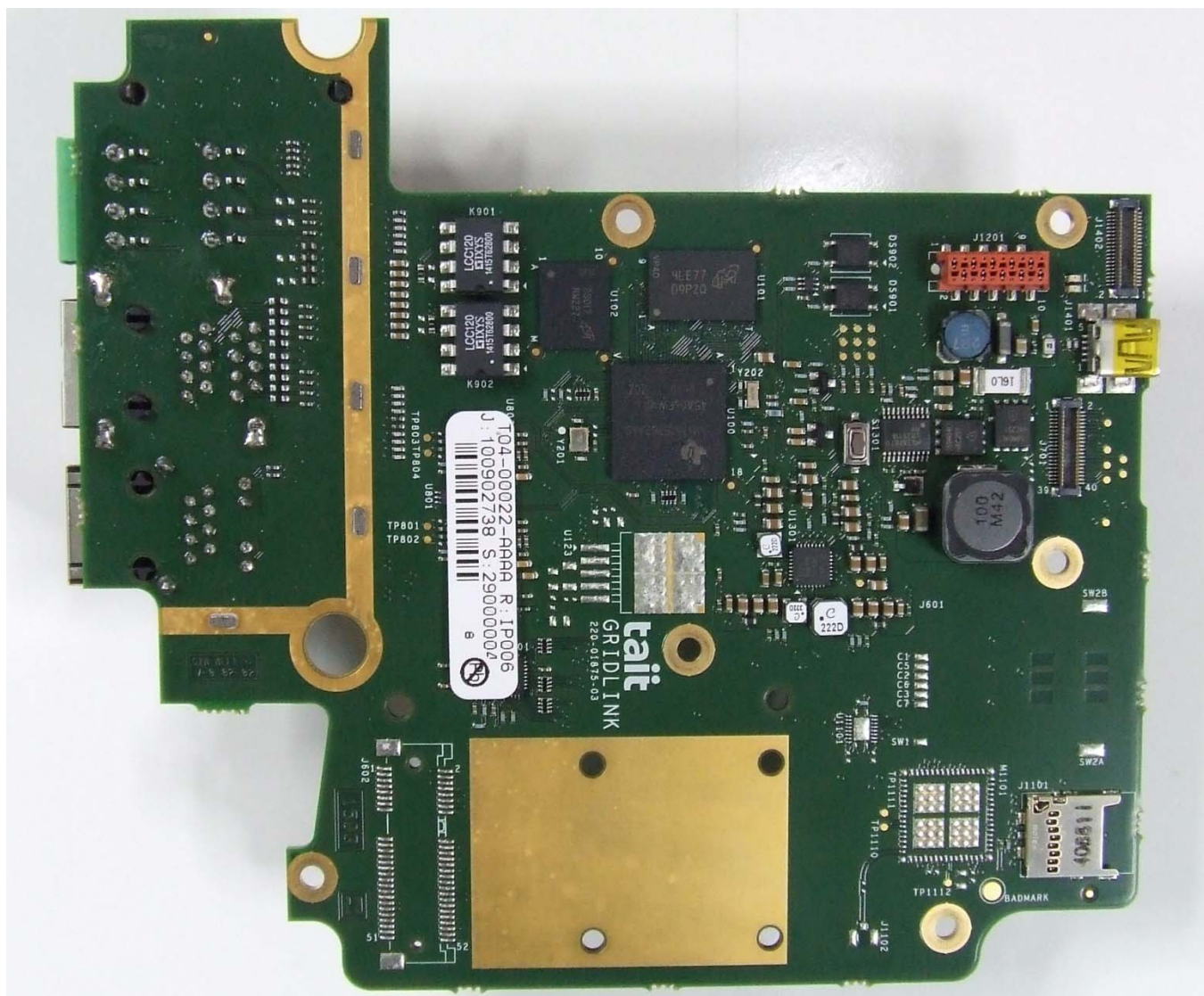
Photograph 02: Main PCB top
