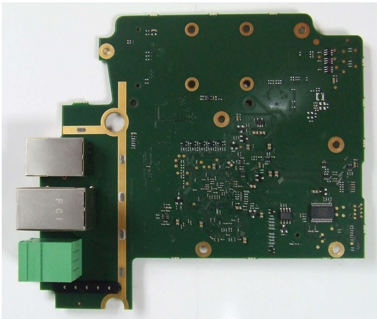
Photograph 03: Main PCB bottom
