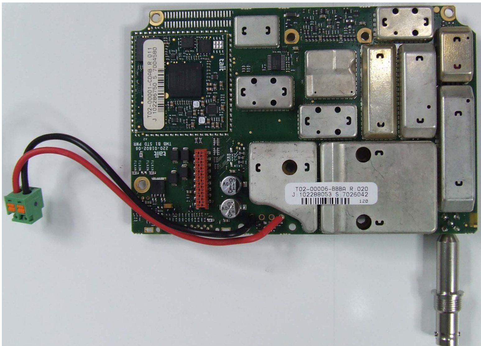
Photograph 04: RF PCB top with shields
