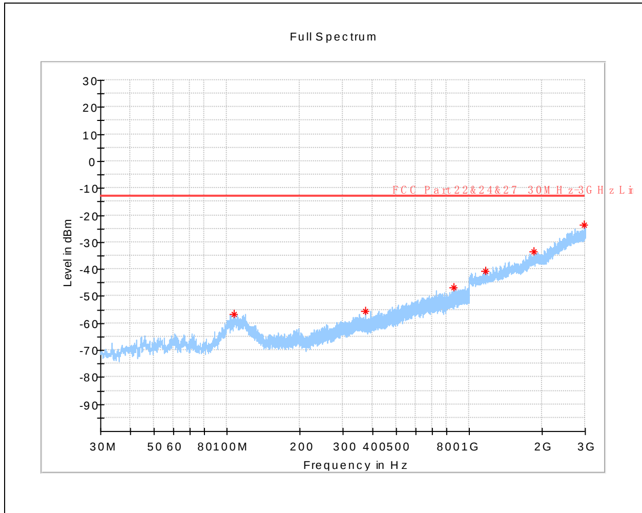
(WCDMA Band II _ Middle Channel _ 30MHz to 3GHz _ Vertical)
