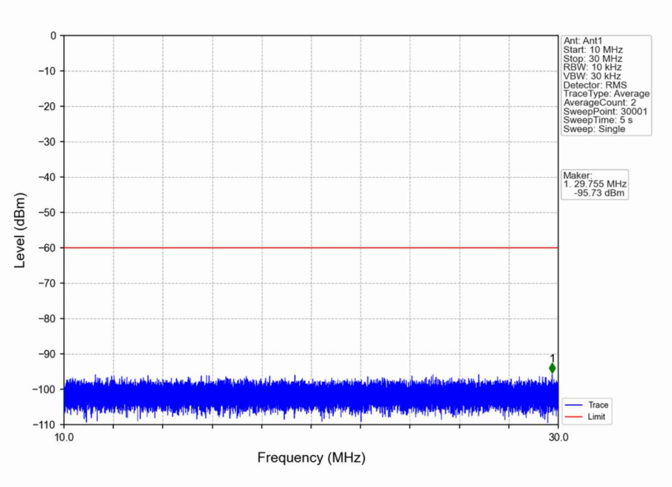
n48_30kHz_SISO_NTNV_40MHz_DFT-s-OFDM QPSK_3570MHz_Outer_Full
