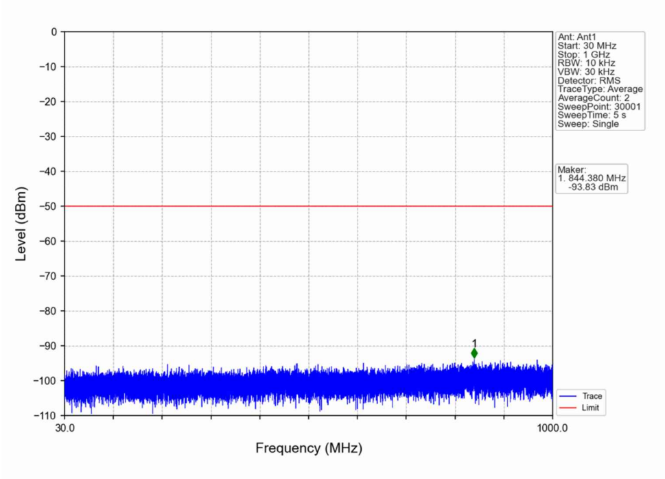
n48_30kHz_SISO_NTNV_40MHz_DFT-s-OFDM QPSK_3679.98MHz_Outer_Full
