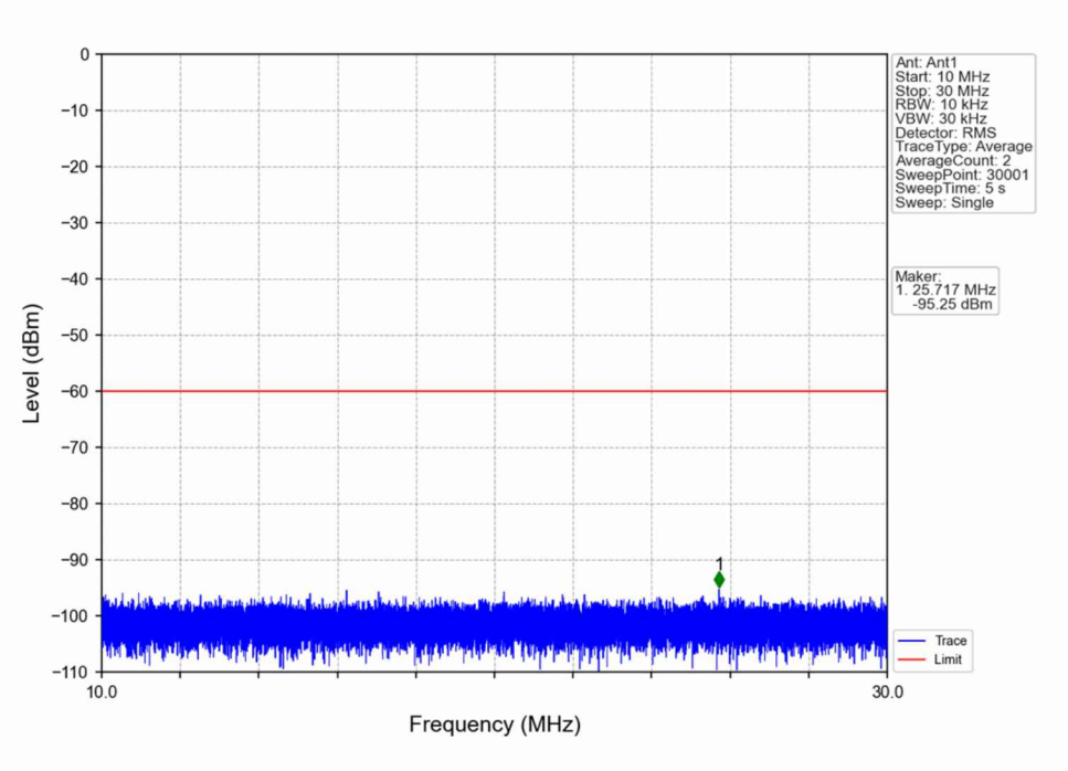
n48_30kHz_SISO_NTNV_20MHz_CP-OFDM QPSK_3690MHz_Outer_Full
