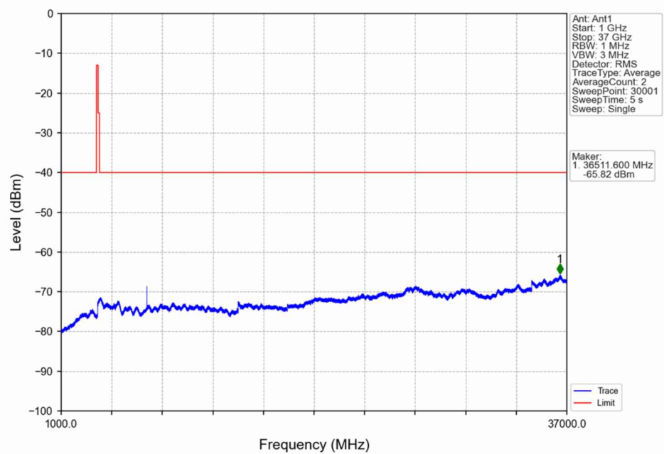
n48_30kHz_SISO_NTNV_40MHz_DFT-s-OFDM QPSK_3570MHz_Edge_1RB_Left
