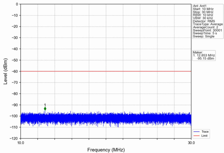
n48_30kHz_SISO_NTNV_40MHz_DFT-s-OFDM QPSK_3679.98MHz_Edge_1RB_Right
