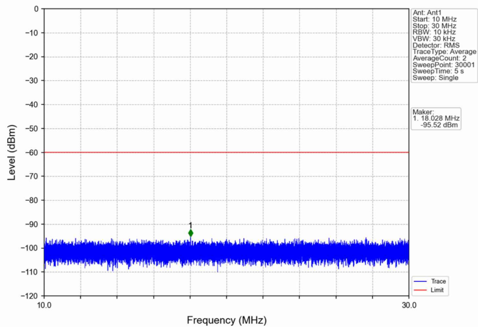
n48_30kHz_SISO_NTNV_40MHz_DFT-s-OFDM QPSK_3679.98MHz_Inner_1RB_Right
