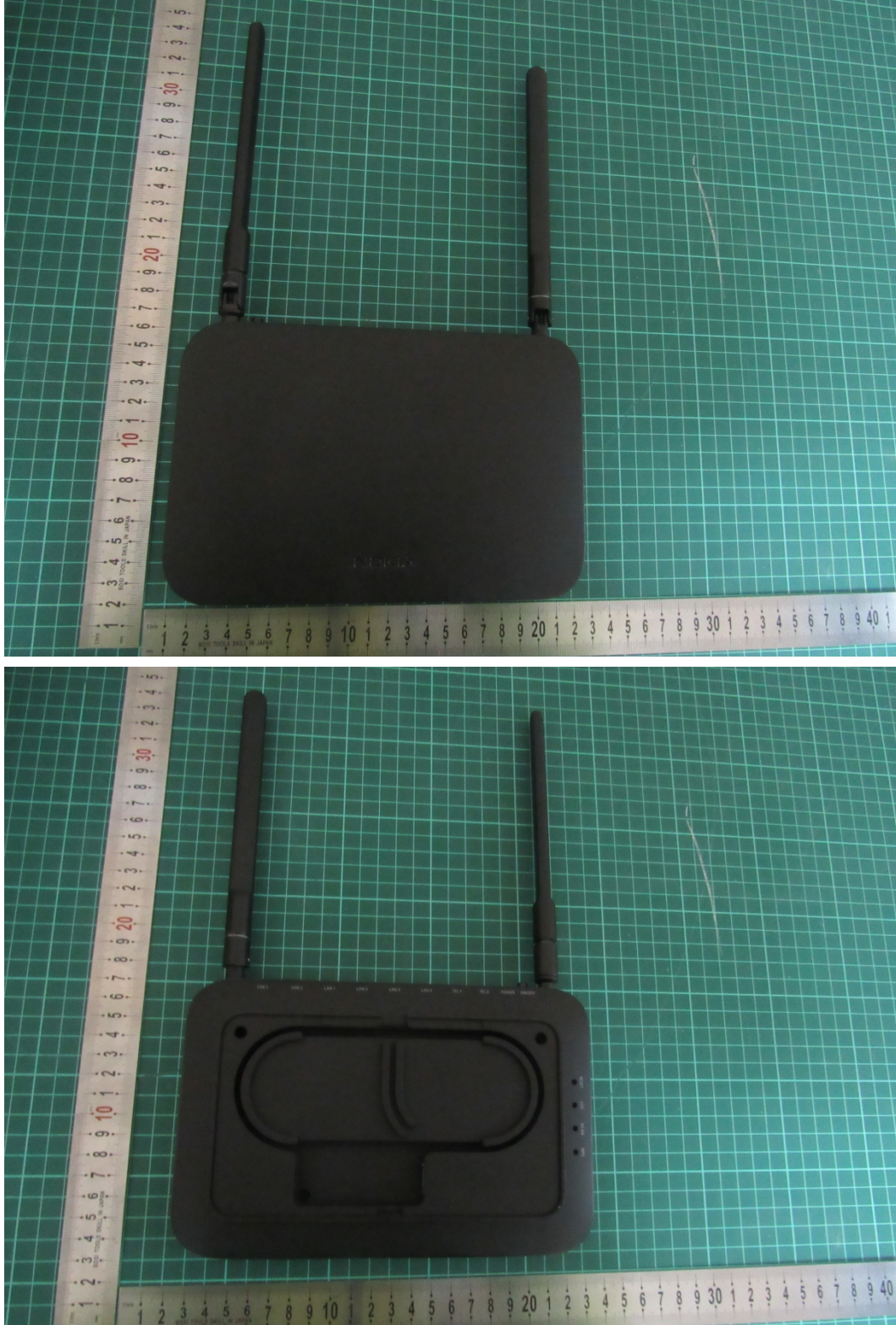
Picture 1-1: EUT
