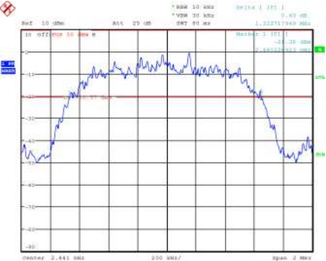
Figure 5-5: 20 dB Bandwidth Single freq., Static PBRS, 2-DH5
