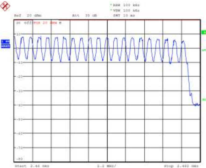
Figure 5-16: Number of Hopping Frequencies Static PBRs, DH5
