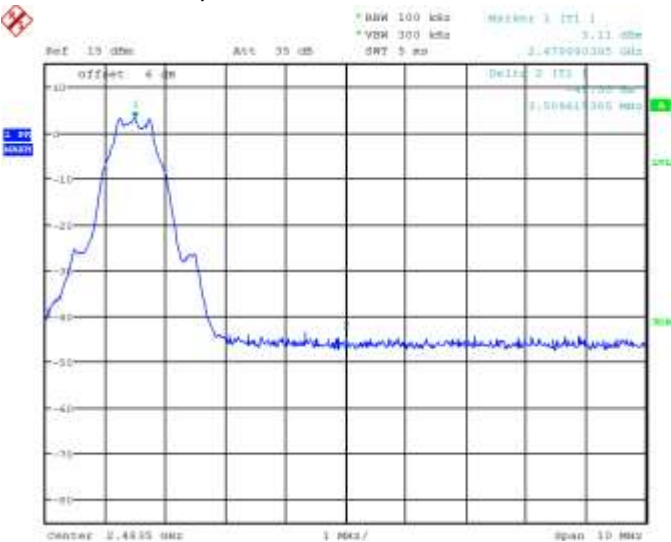
Figure 5-54: Band Edge Compliance LE, Channel 39
