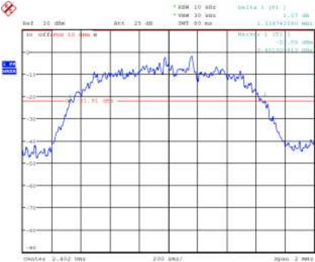
Figure 5-7: 20 dB Bandwidth Single freq., Static PBRs, 3-DH5
