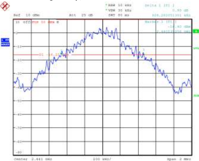
Figure 5-2: 20 dB Bandwidth Single freq., Static PBRS, DH5
