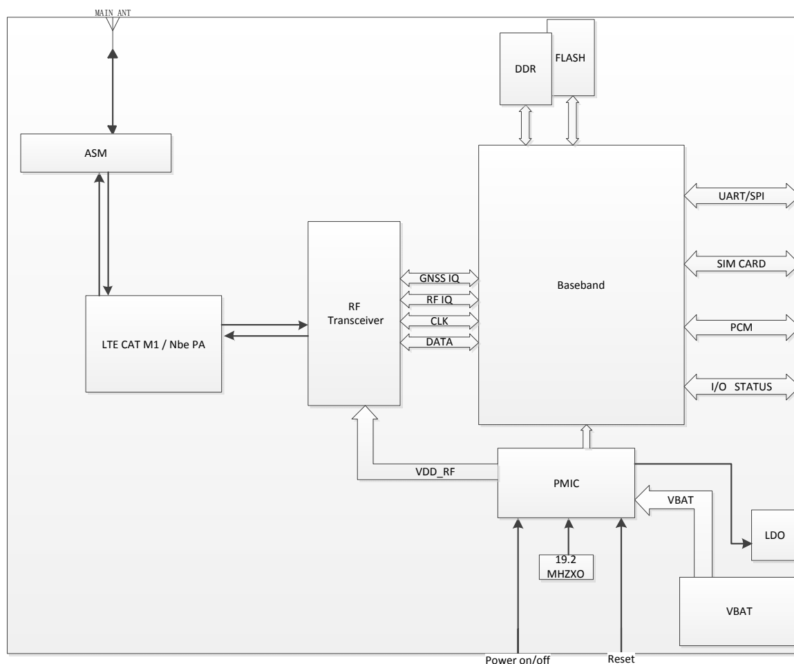
Figure 2-3 L600 System Functional Architecture
