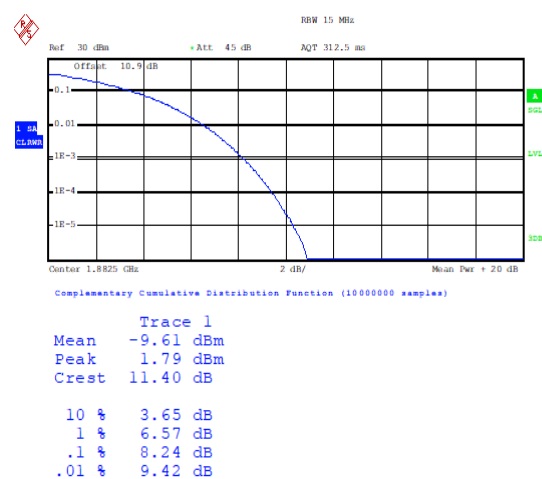
Band25-15MHz-QPSK-26365-1RB#0-PASS
