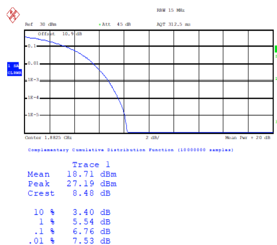
Band25-15MHz-QPSK-26365-75RB#0-PASS
