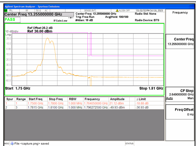
66C / 15+15MHz / High CH / QPSK / 1#74-1#0
