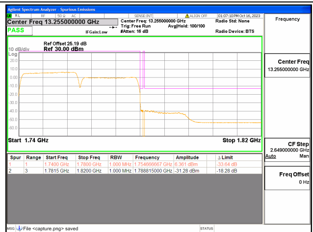
66C / 20+20MHz / High CH / QPSK / 100#0-100#0
