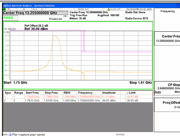
66C / 20+10MHz / High CH / QPSK / 1#99-1#0
