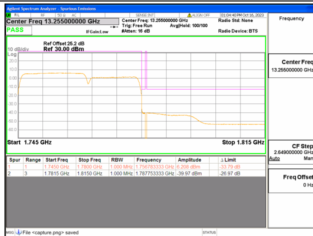
66C / 20+15MHz / High CH / QPSK / 100#0-75#0
