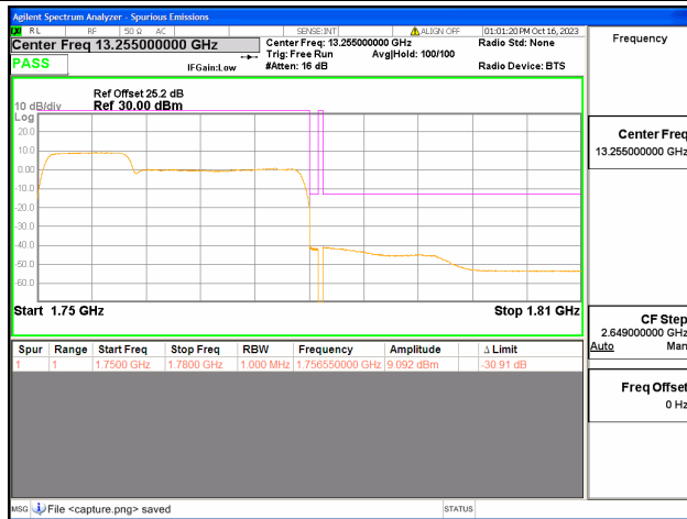
66C / 10+20MHz / High CH / QPSK / 50#0-100#0
