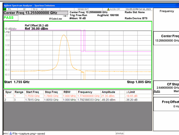
66C / 20+5MHz / High CH / QPSK / 1#99-1#0
