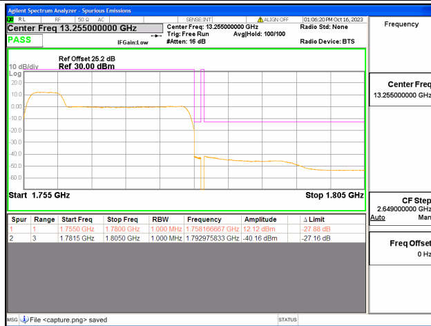
66C / 5+20MHz / High CH / QPSK / 25#0-100#0
