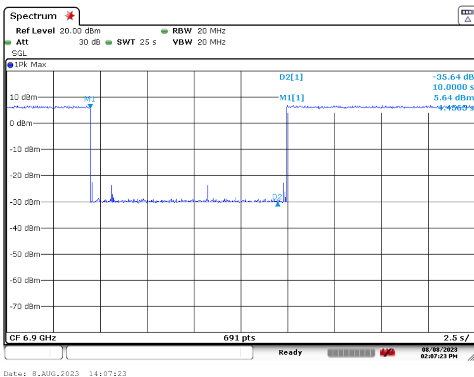
Plot 7-109. Contention Based Protocol Timing Plot (160MHz (UNII Band 7) – Ch. 175 High)
