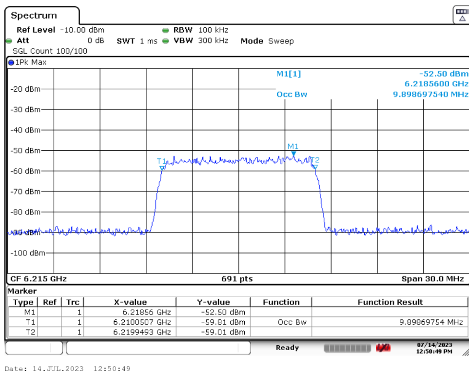
Plot 7-97. AWGN Signal (Demonstration)
