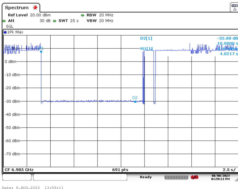
Plot 7-112. Contention Based Protocol Timing Plot (160MHz (UNII Band 8) – Ch. 207 Mid)
