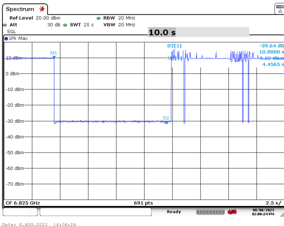
Plot 7-108. Contention Based Protocol Timing Plot (160MHz (UNII Band 7) – Ch. 175 Mid)
