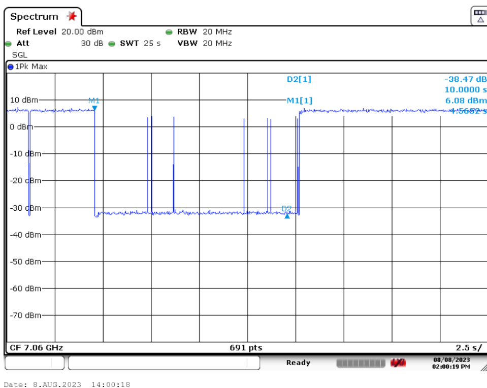
Plot 7-113. Contention Based Protocol Timing Plot (160MHz (UNII Band 8) – Ch. 207 High)
