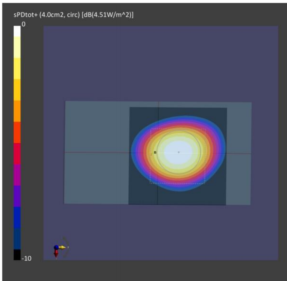
Figure 8-4: 4cm2-averaged power density distribution measured at input.power.limit of 4.51dBm on the back surface for n261 beam 40
