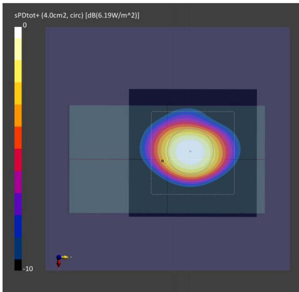
Figure 8-2: 4cm 2 -averaged power density distribution measured at input.power.limit of 6.19 dBm on the Right Side surface for n260 beam 30
