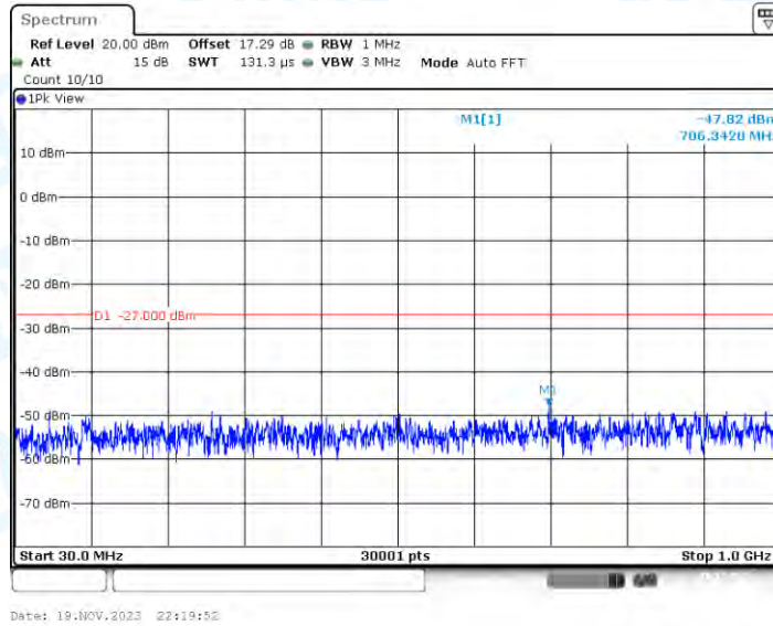
11N40-CDD_Ant2_5755_1000~40000
