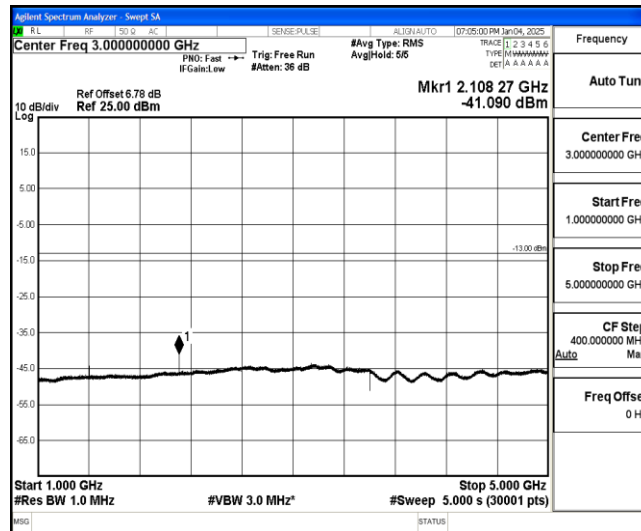
Band85-10MHz-QPSK-134092-1-0-Low-1000-5000--41.09-PASS
