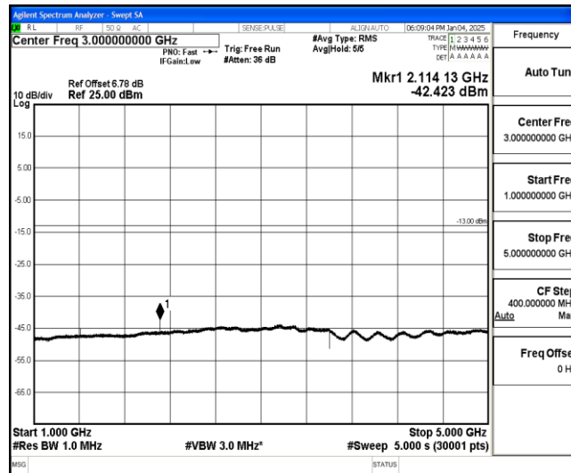
Band85-5MHz-16QAM-134092-1-0-Low-1000-5000--42.42-PASS
