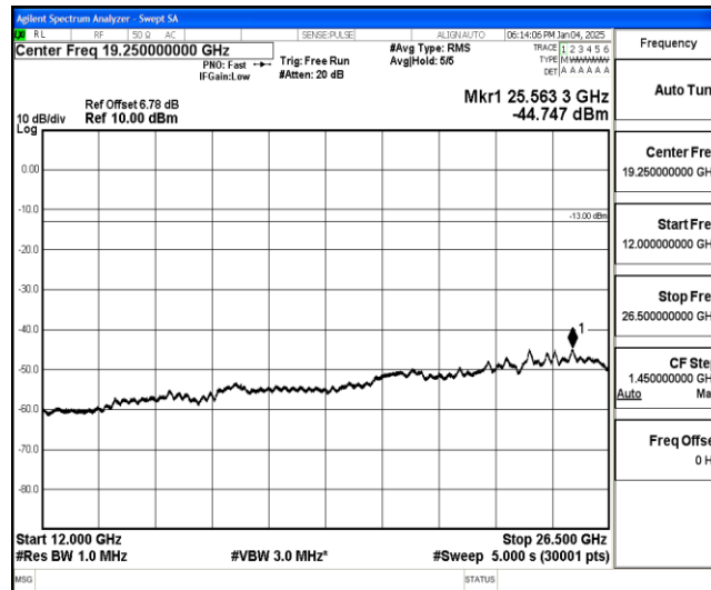
Band85-5MHz-16QAM-134157-1-0-High-12000-26500--44.75-PASS
