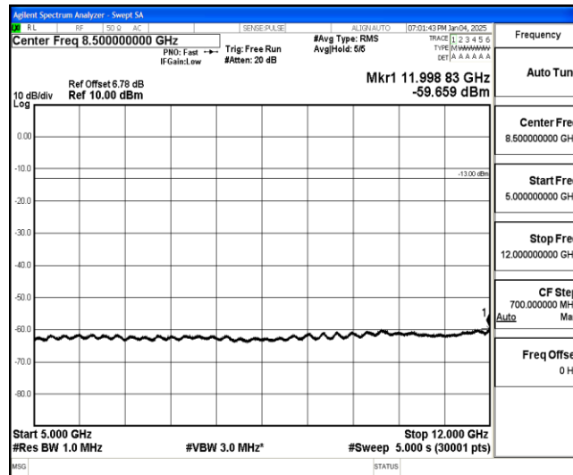
Band85-10MHz-QPSK-134052-1-0-Low-5000-12000--59.66-PASS
