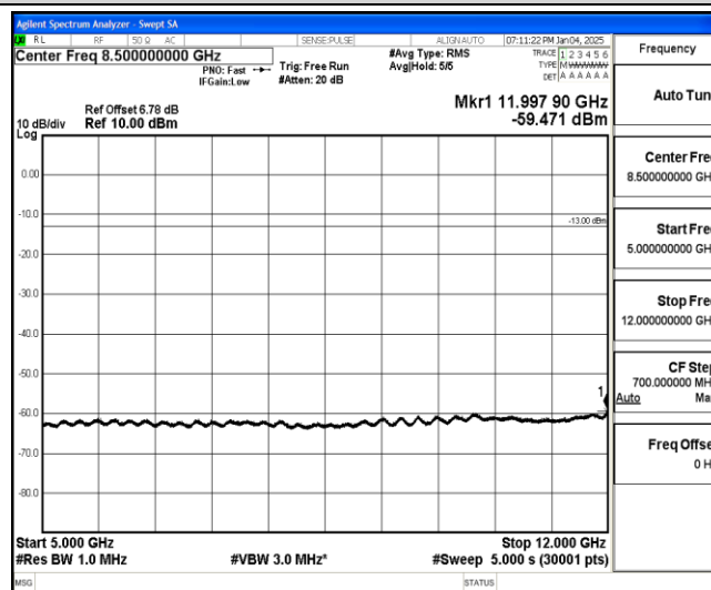
Band85-10MHz-16QAM-134132-1-0-High-5000-12000--59.47-PASS
