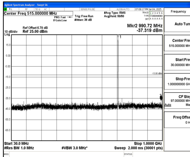
Band85-10MHz-QPSK-134132-1-0-High-30-1000--37.32-PASS
