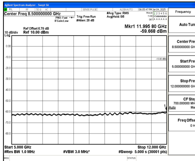
Band85-5MHz-16QAM-134027-1-0-Low-5000-12000--59.67-PASS
