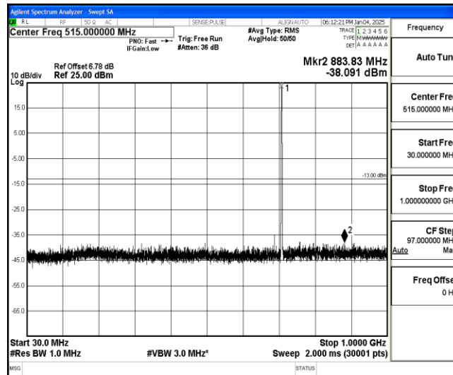
Band85-5MHz-16QAM-134157-1-0-High-30-1000--38.09-PASS
