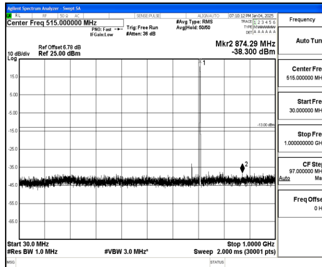
Band85-10MHz-16QAM-134132-1-0-High-30-1000--38.3-PASS
