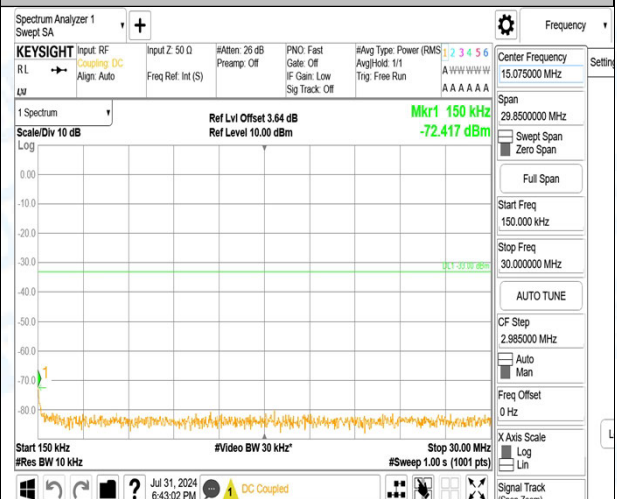
Band2_10MHz_QPSK_18650_50RB#0_1000~3000_1000~3000
