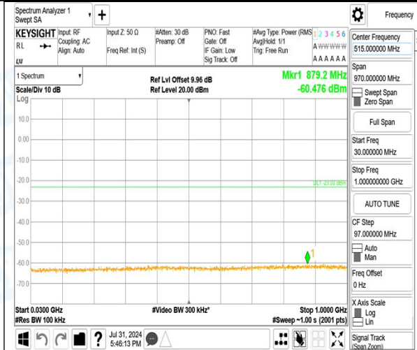
Band2_5MHz_16QAM_18900_25RB#0_3000~20000_3000~2000
