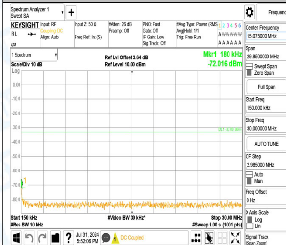
Band2_5MHz_16QAM_19175_25RB#0_0.15~30_0.15~30
