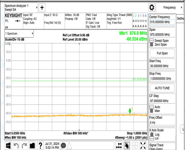
Band2_5MHz_16QAM_19175_25RB#0_30~1000_30~1000
