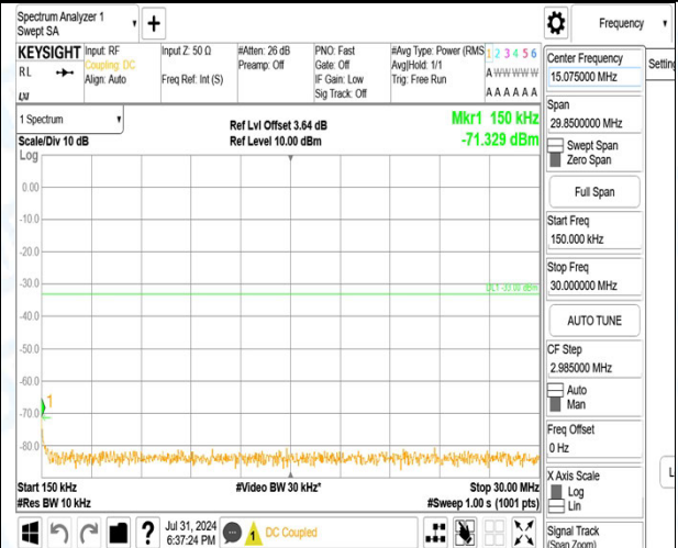
Band2_10MHz_QPSK_19150_1RB#0_1000~3000_1000~3000
