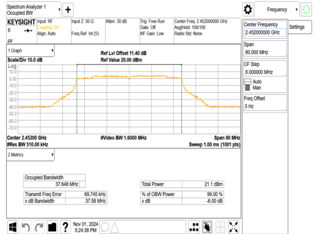
802.11ax_40MHz_ChainA_2452MHz_RU242_62
