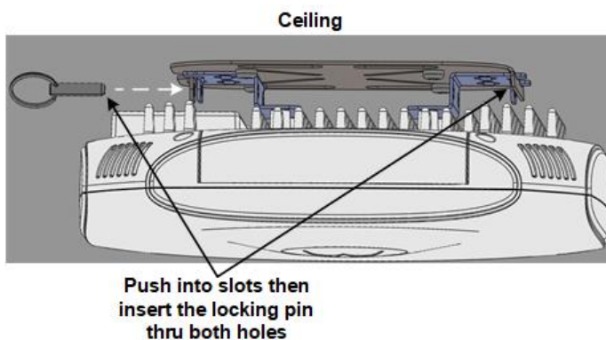
Figure 13: Insert &amp; Secure Locking Pin
