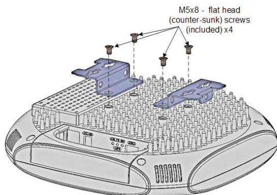
Figure 14: Assemble Rail Brackets to the Unit
