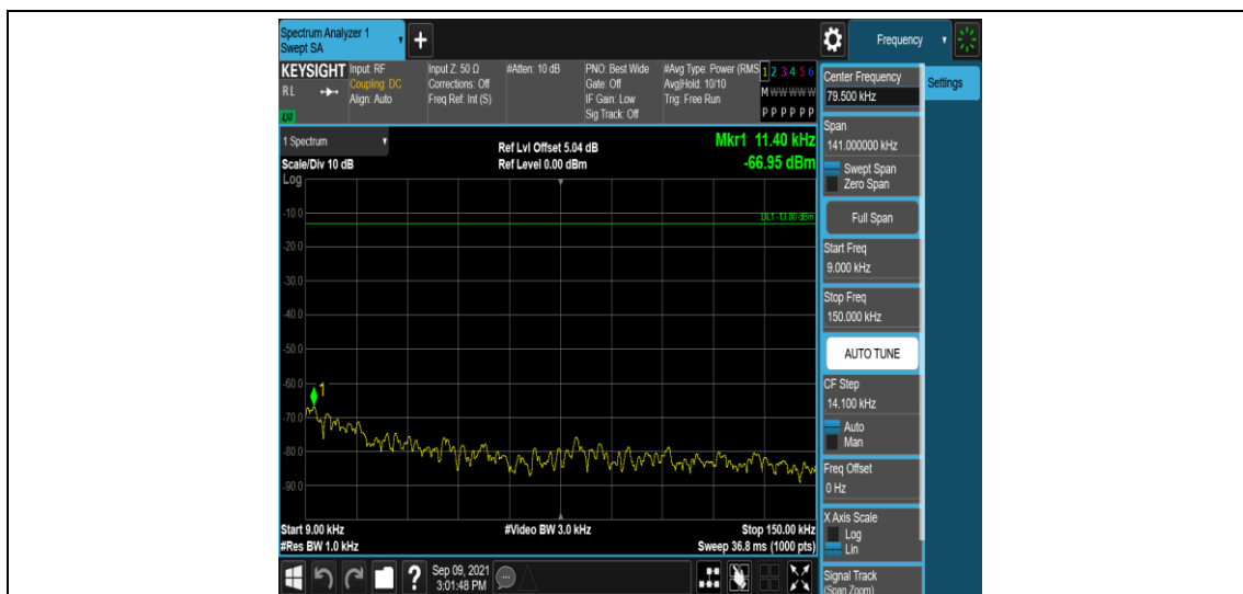
Band4-15MHz-QPSK-20325-1RB#0-Range1:0.009~0.15MHz
