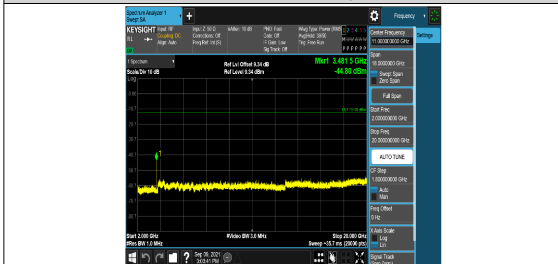
Band4-15MHz-16QAM-20325-1RB#0-Range5:2000~20000MHz
