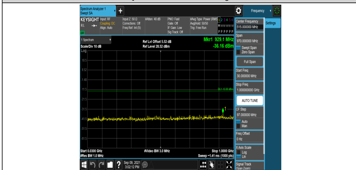
Band4-15MHz-QPSK-20325-1RB#0-Range3:30~1000MHz
