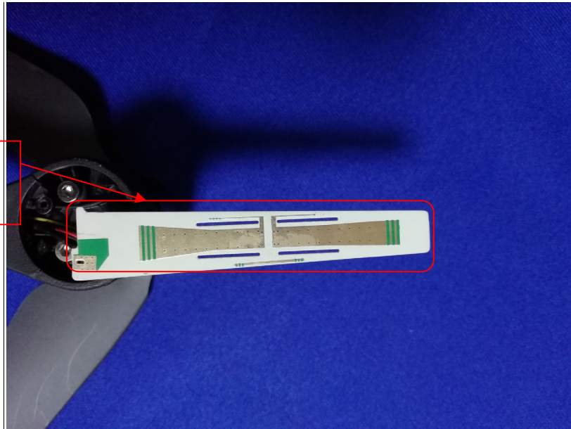
Front view of Optional antenna 2
