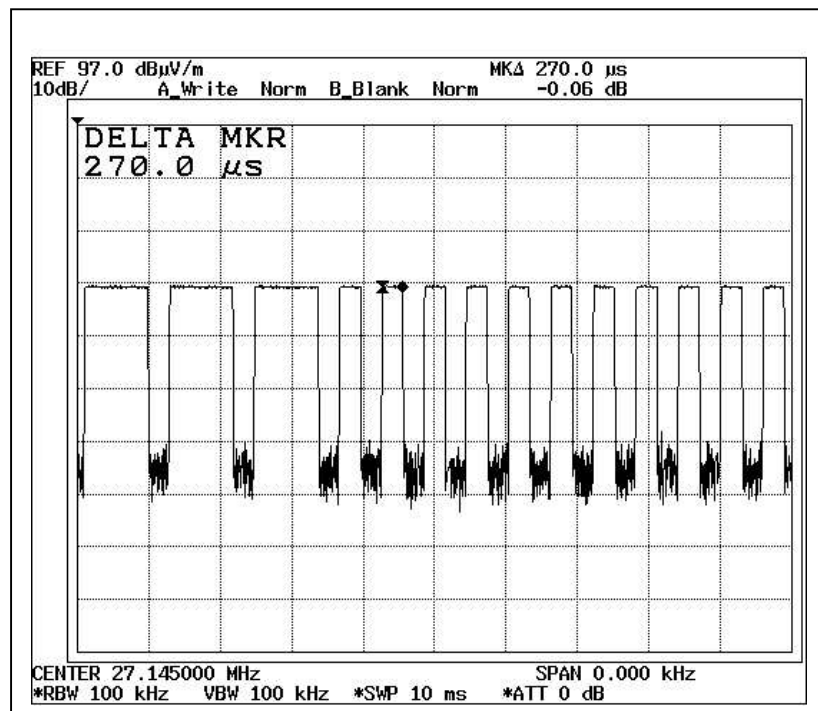
Duty Cycle 3
