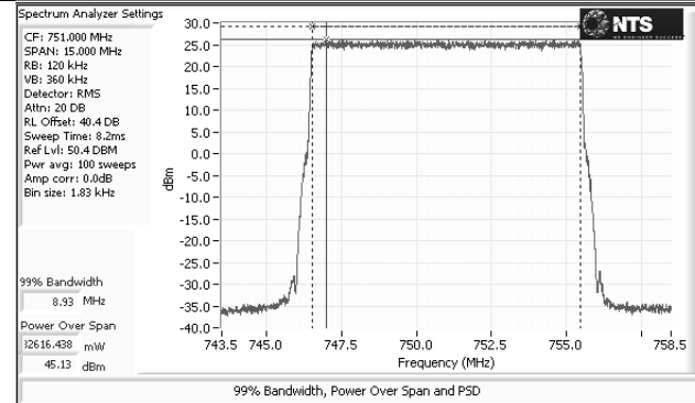
Port 2 – LTE – 16QAM – 10M – Center Channel – Average
