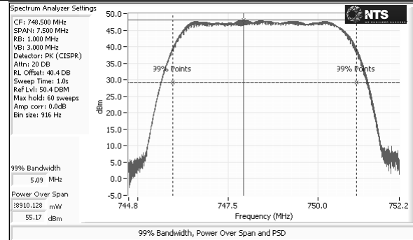
Port 2 – LTE – 64QAM – 5M – Low Channel – Peak
