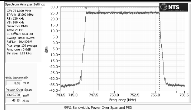
Port 2 – LTE – 64QAM – 10M – Center Channel – Average
