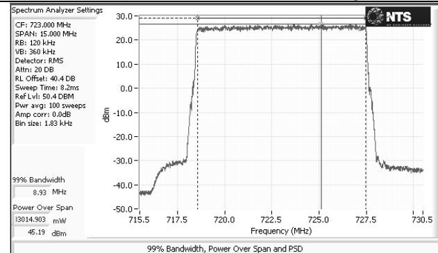
Port 3 – LTE – 64QAM – 10M – Center Channel – Average
