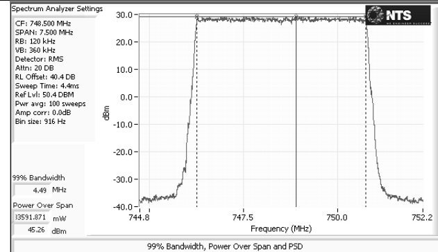
Port 2 – LTE – 64QAM – 5M – Low Channel – Average
