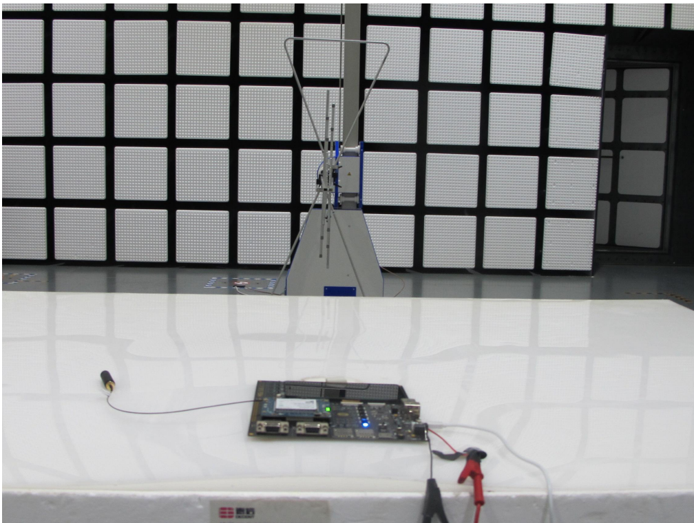
Pic1-2. Radiated emissions (30MHz-1GHz)
