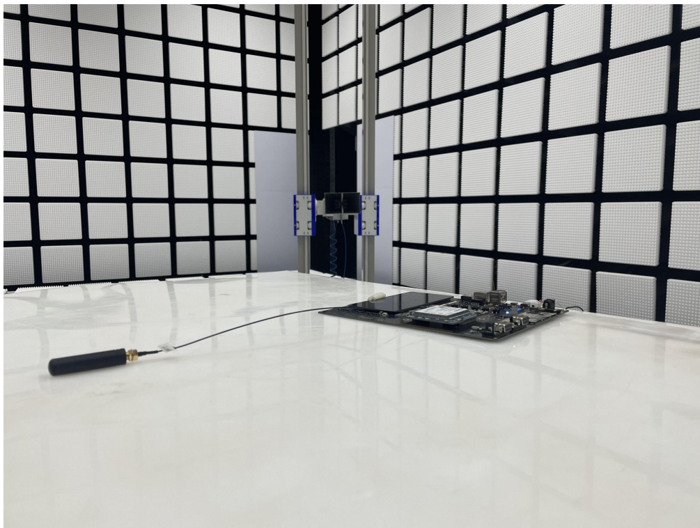
Pic3-4.Radiated emissions (1GHz-18GHz)
