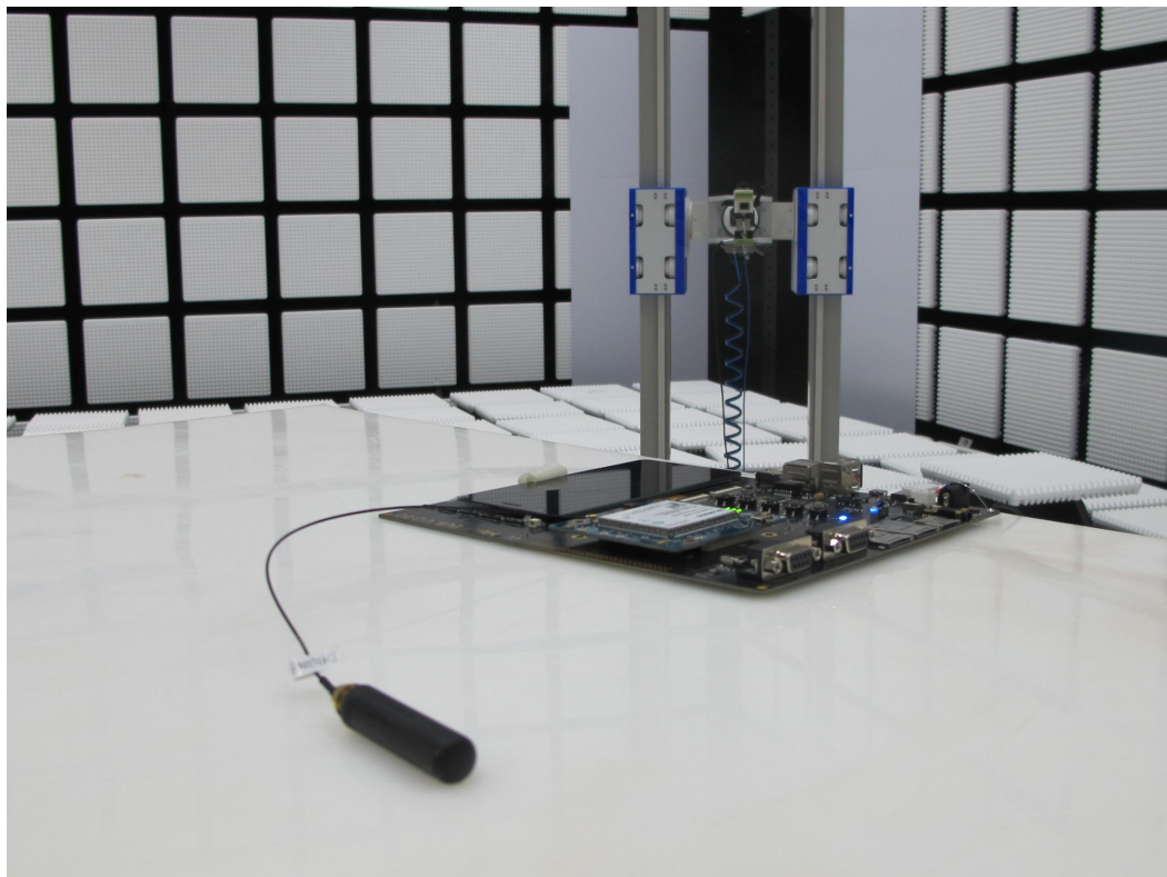
Pic4. Radiated emissions (26.5GHz-40GHz)
