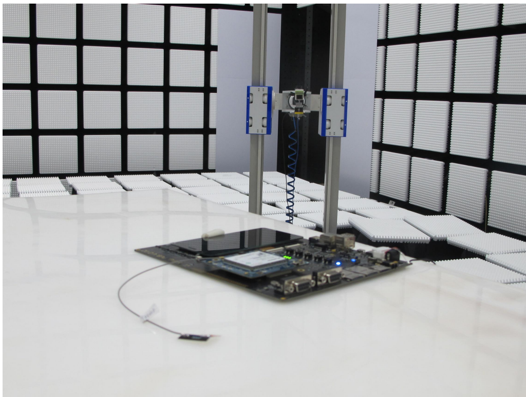
Pic5-6. Radiated emissions (18GHz-26.5GHz)
