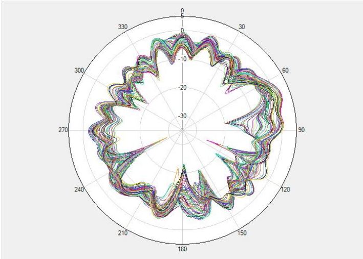
Phi 0 Etotal dB
