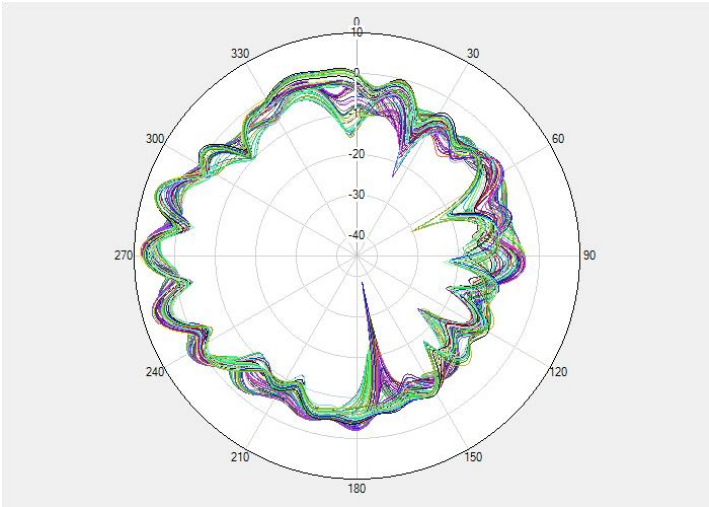
Theta 90 Etotal dB
