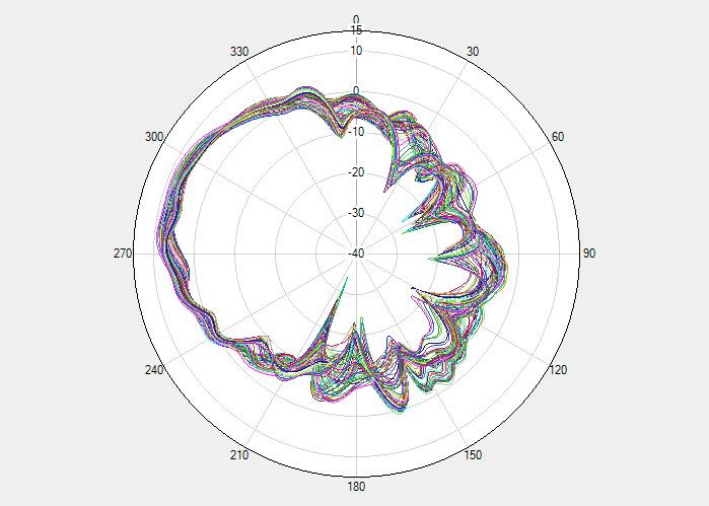
Phi 90 Etotal dB
