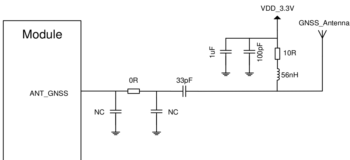
Figure 4-4 GNSS active antenna reference design
