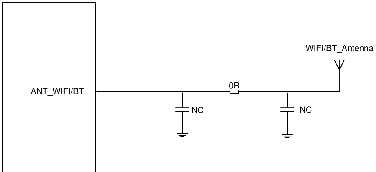
Figure 4-2 WIFI/BT antenna reference design
