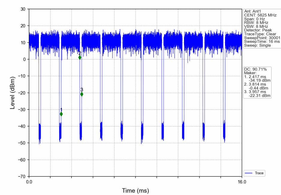
802.11a_HCH_5825MHz_Ant1_NTNV
