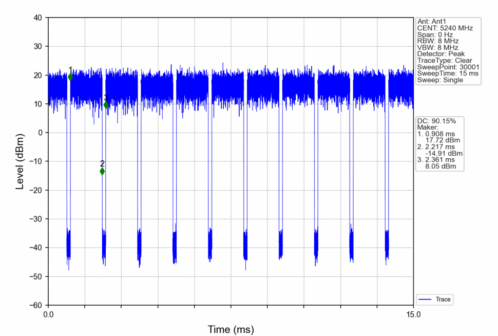
802.11n(HT20)_HCH_5240MHz_Ant1_NTNV
