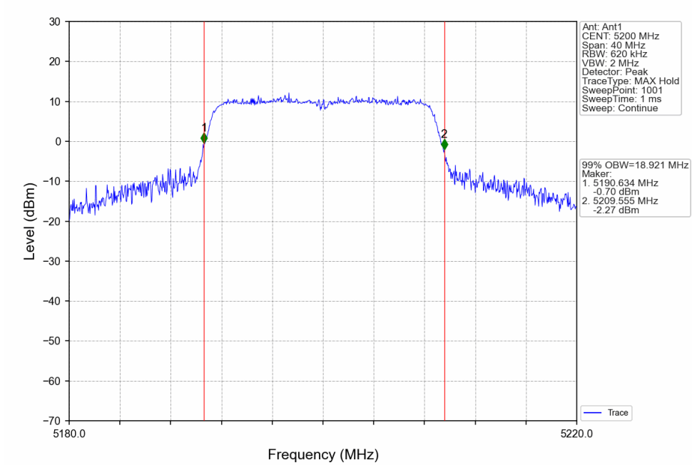
802.11n(HT20)_MCH_5200MHz_Ant1_NTNV
