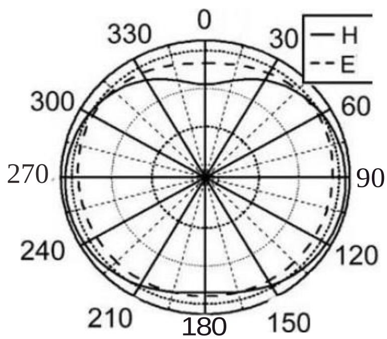
49.86 MHz radiation pattern
