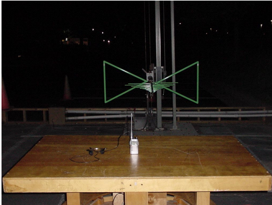
PHOTOGRAPH 6: RADIATED TEST CONFIGURATION TEST PICTURES (FRONT VIEW)
