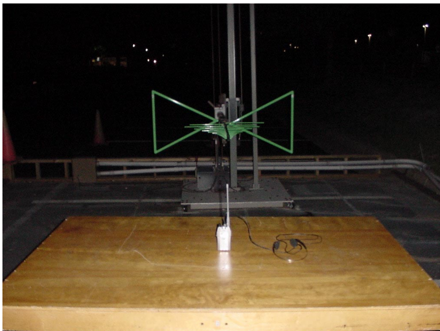
PHOTOGRAPH 7: RADIATED TEST CONFIGURATION TEST PICTURES (REAR VIEW)
