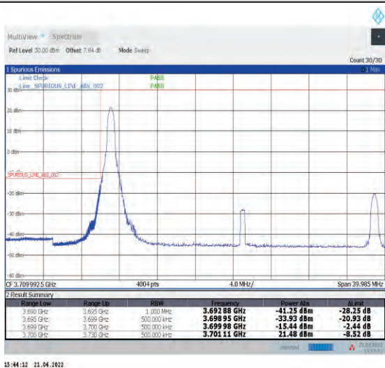
1-N77-3700-3980--30-30-L-4-CP-QPSK-Edge_1RB_L_eff-1@0-Ant1-PASS-see graph
