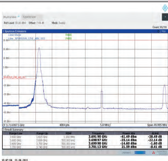
1-N77-3700-3980--30-40-L-4-CP-QPSK-Edge_1RB_L_eff-1@0-Ant1-PASS-see graph
