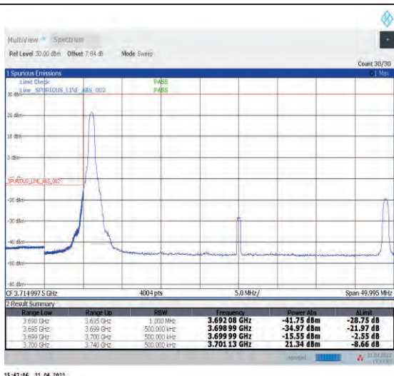
1-N77-3700-3980--30-40-L-1-DFT-PI2BPSK-Edge_1R_B_Left-1@0-Ant1-PASS-see graph
