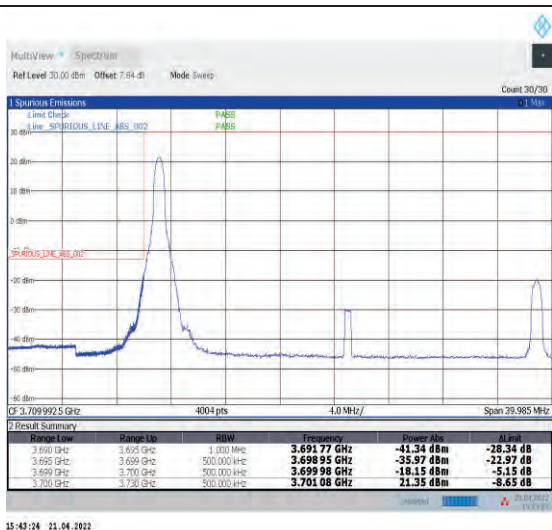
1-N77-3700-3980--30-30-L-1-DFT-PI2BPSK-Edge_1R_B_Left-1@0-Ant1-PASS-see graph
