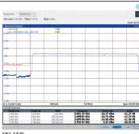
1-N77-3700-3980--30-40-L-6-CP-QPSK-Outer_Ful_I-106@0-Ant1-PASS-see graph
