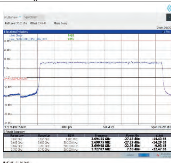
1-N77-3700-3980--30-40-L-3-DFT-PI2BPSK-Outer_Full-100@0-Ant1-PASS-see graph
