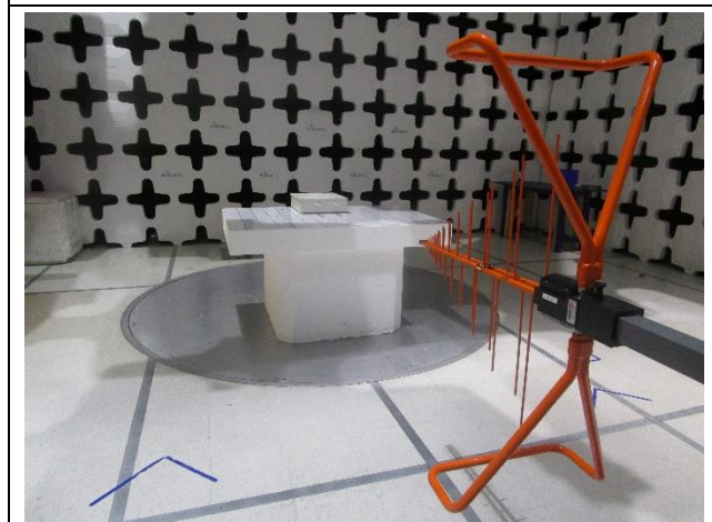
Spurious Emission Below 1GHz-Front View
