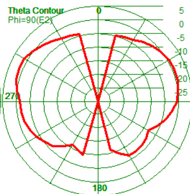
Efficiency: 63.49%
