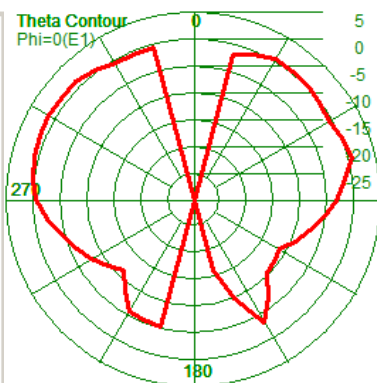
Peak Gain: 3.30dBi
