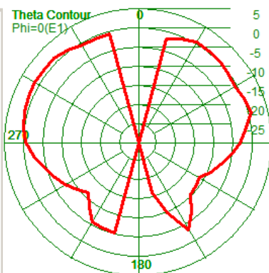
Peak Gain: 3.44dBi
