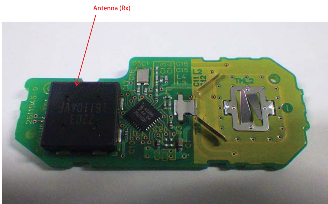
Figure 8.2 GHR-H014-T PCB assy (bottom view)
