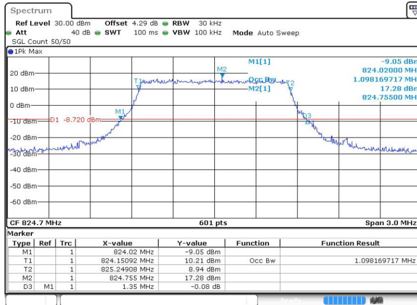
Band26-1.4MHz-QPSK-26797-6RB#0
