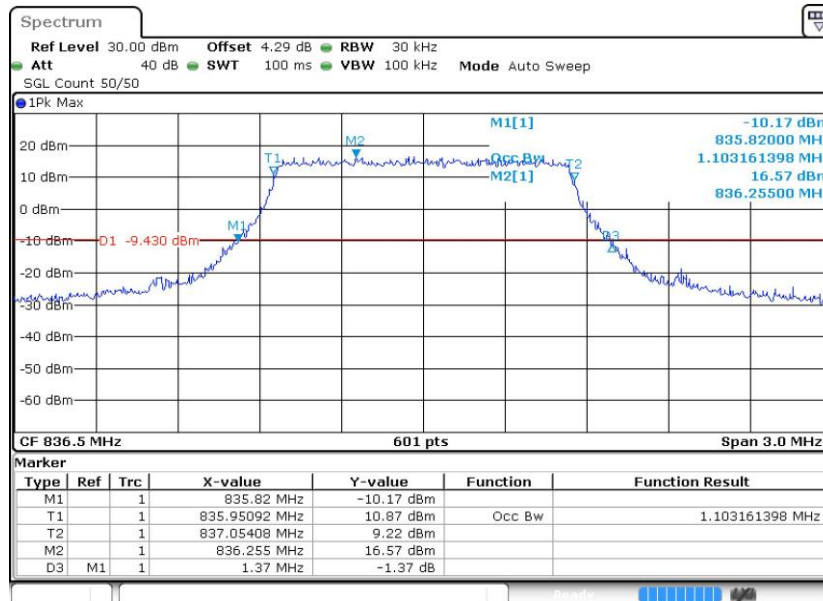
Band26-1.4MHz-QPSK-26915-6RB#0
