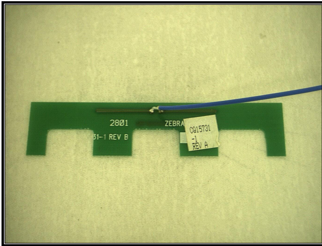
PHOTOGRAPH 33: CAMEO 2 ANTENNA FRONT VIEW
