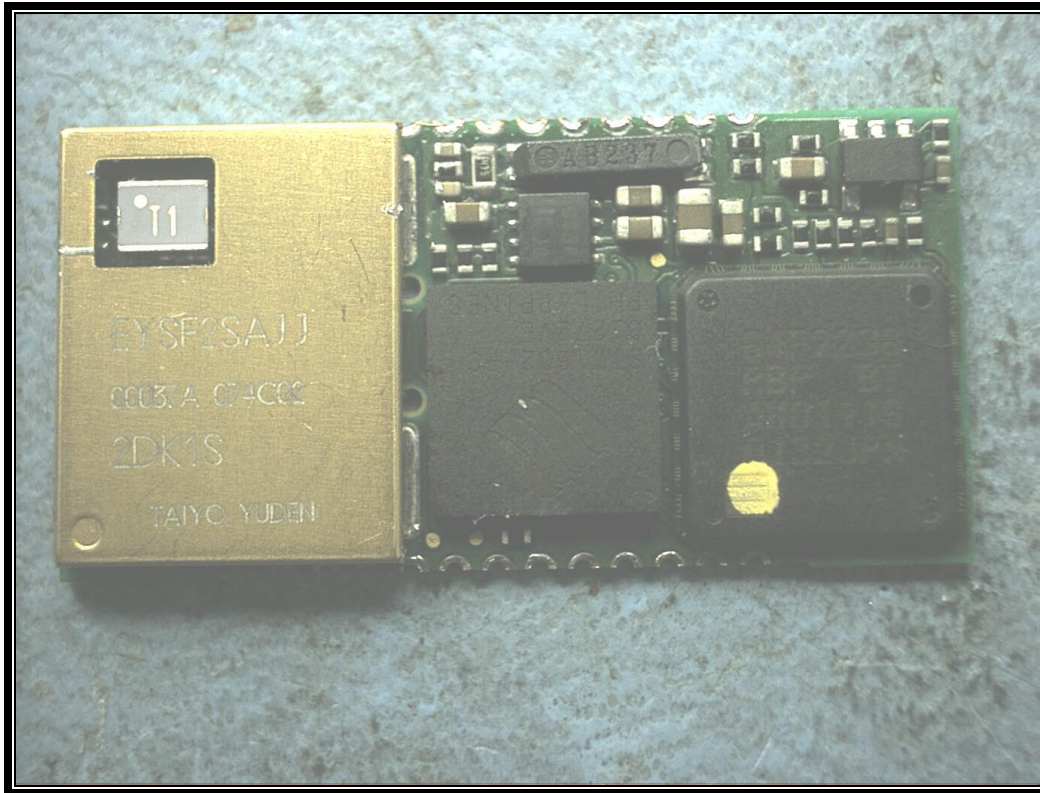
PHOTOGRAPH 28: EUT MAIN BOARD WITH SHIELD TOP VIEW
