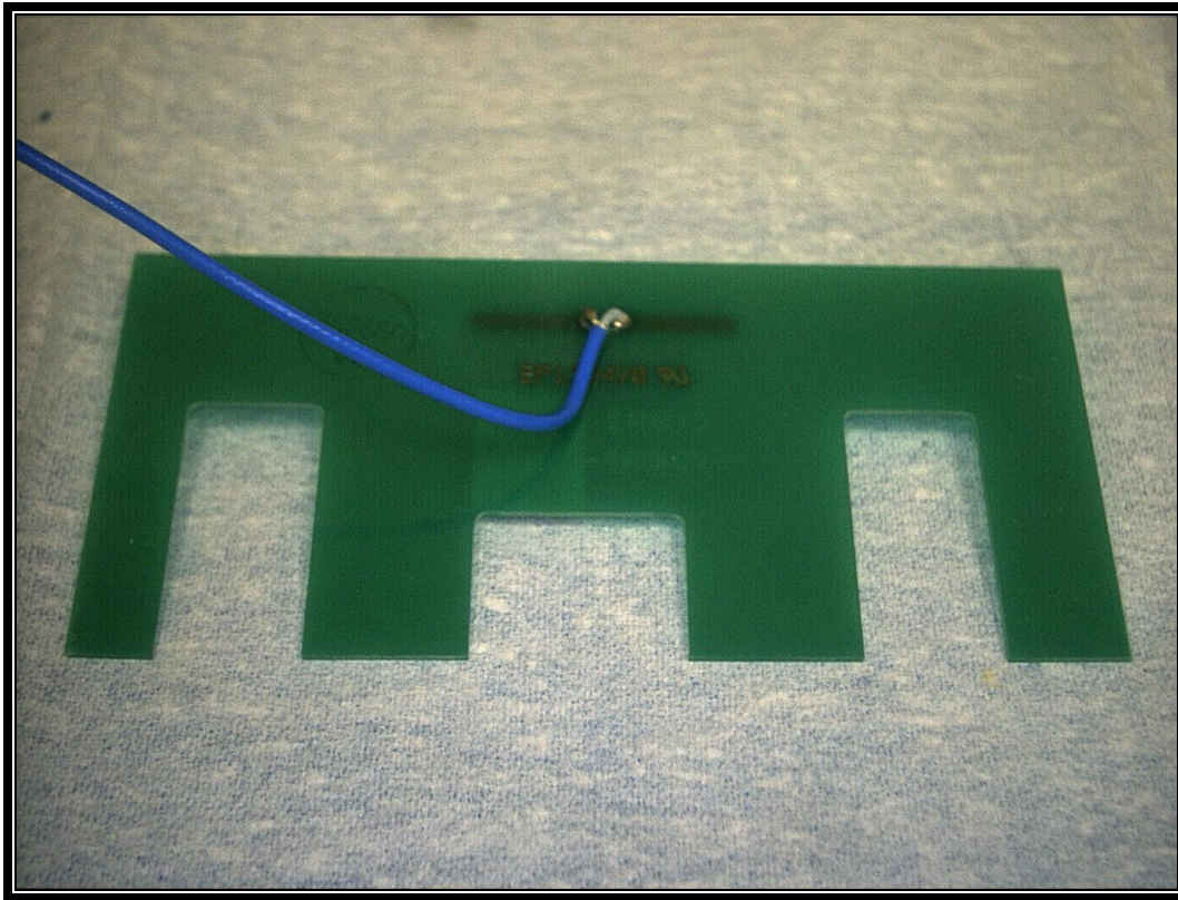
PHOTOGRAPH 38: CAMEO 3 SC ANTENNA BACK VIEW
