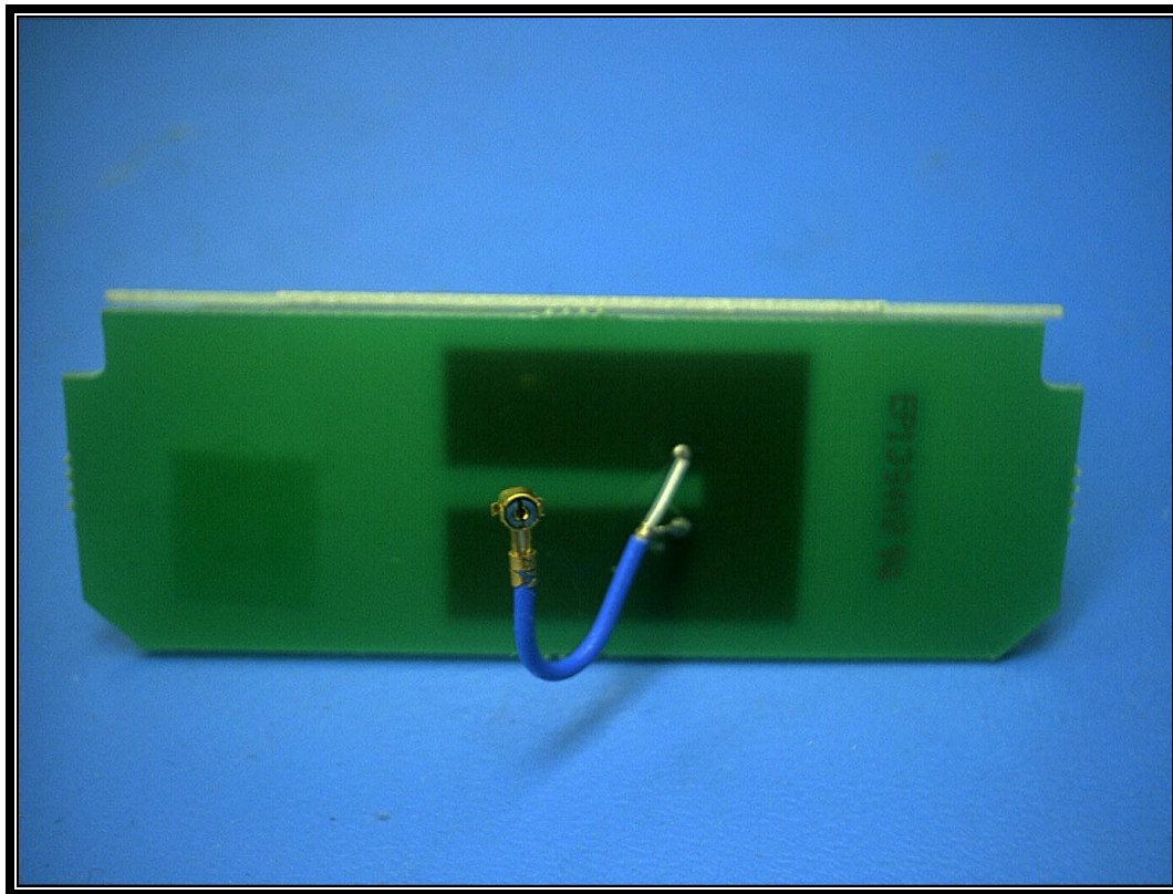
PHOTOGRAPH 40: ZPR POD ANTENNA BACK VIEW
