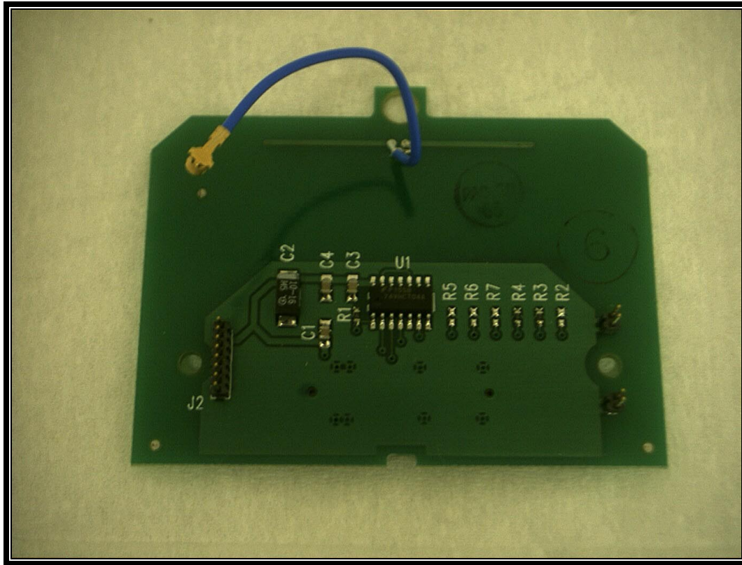
PHOTOGRAPH 35: QL-220/QL-320 ANTENNA FRONT VIEW
