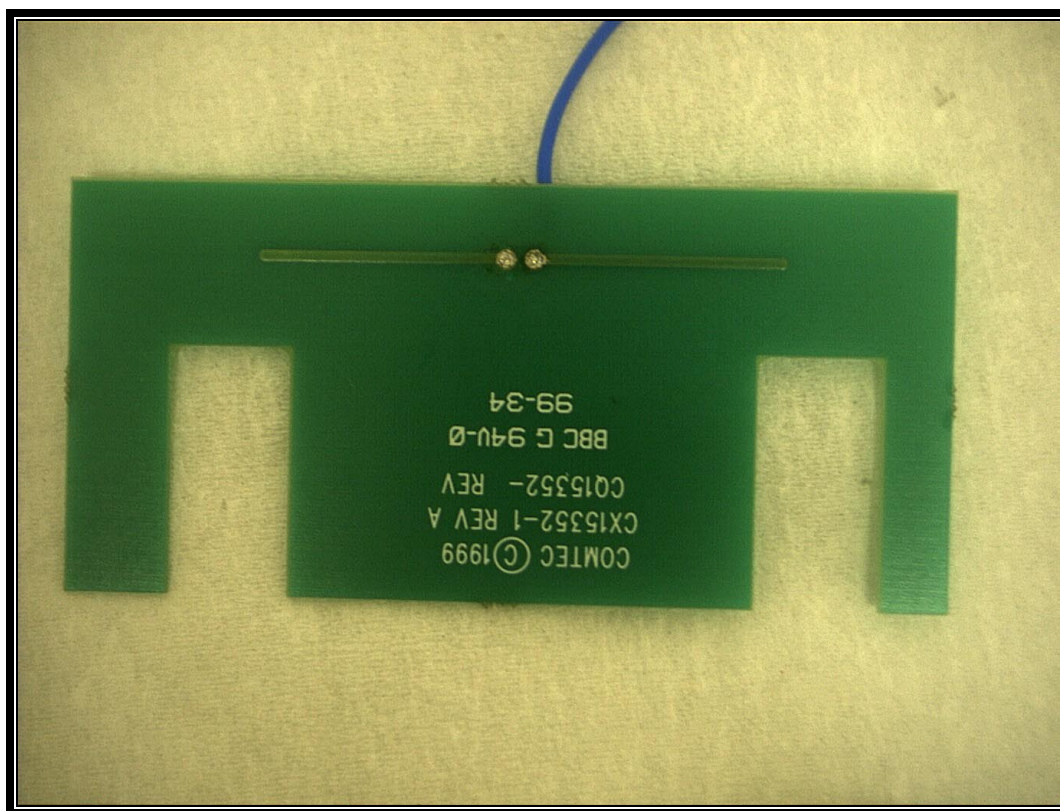
PHOTOGRAPH 31: CAMEO 3 ANTENNA FRONT VIEW
