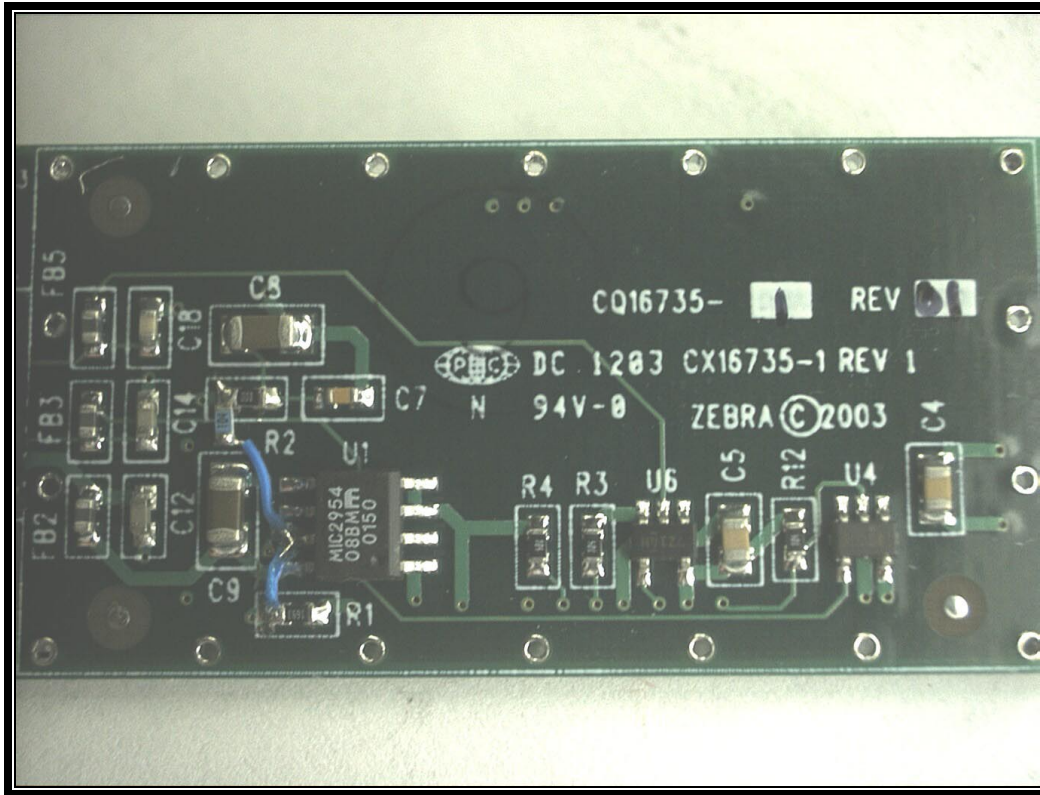
PHOTOGRAPH 30: EUT MAIN BOARD REAR VIEW
