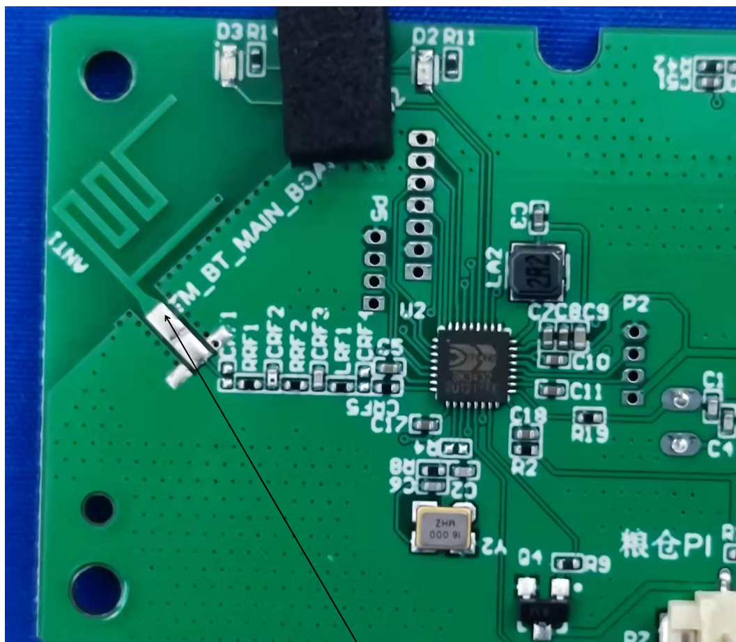
PCB ANTENNA
