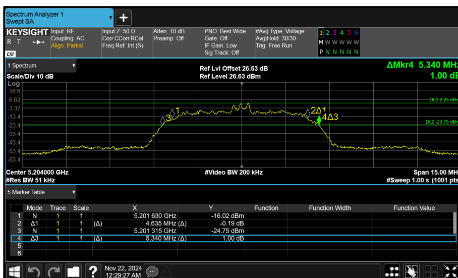
Figure 38 - Core 0 (A) 5204 MHz (CH54) 26 dB and 99% Bandwidth
