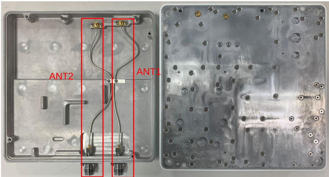
[Antenna Photo]
