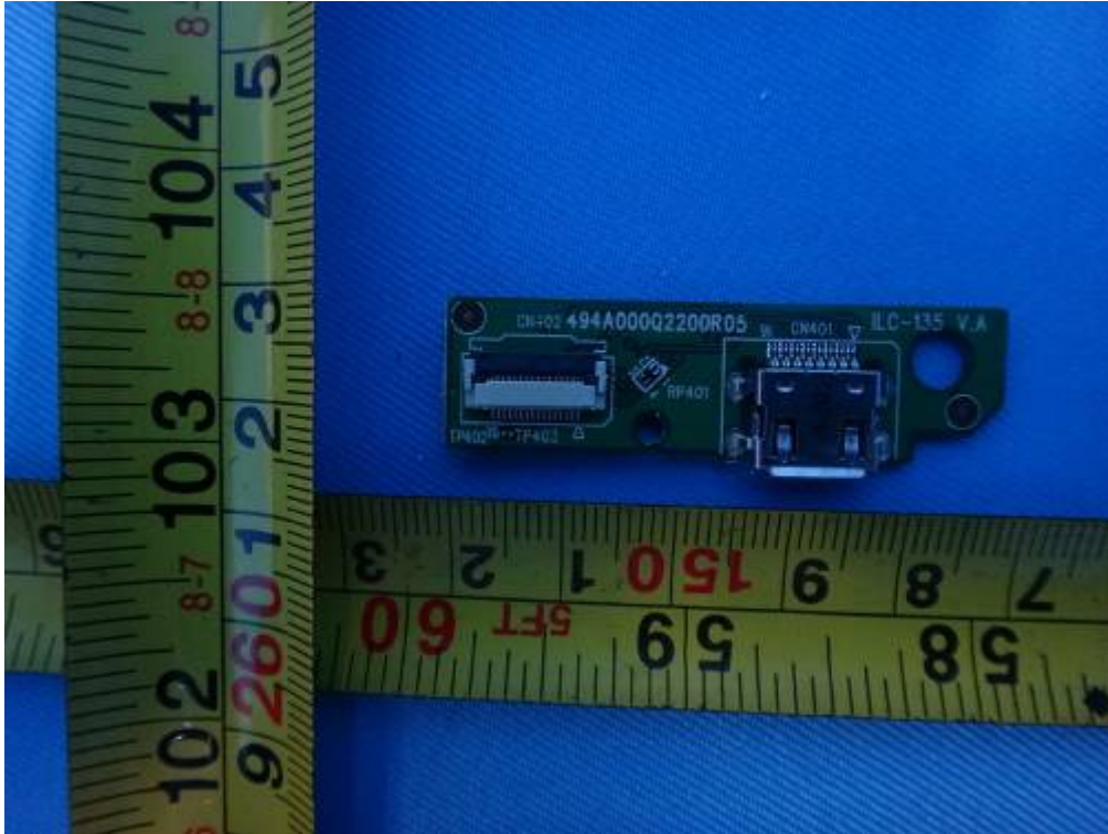
Accessory board
