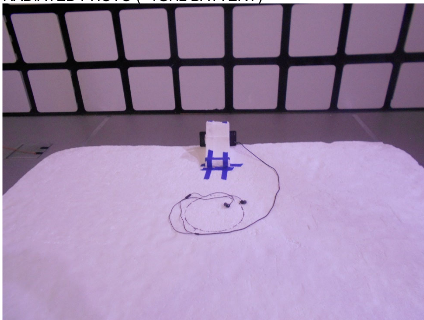
RADIATED PHOTO (>1GHz BATTERY)
