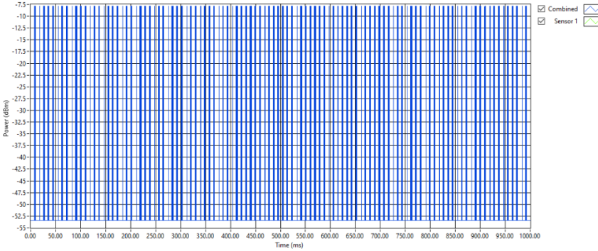
BLE/GFSK 2 Mbps Low Channel, 2402 MHz
