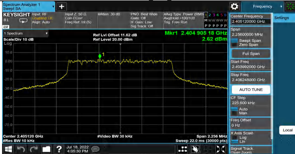
1.4MCA-MIMO Ant2 2405.12
