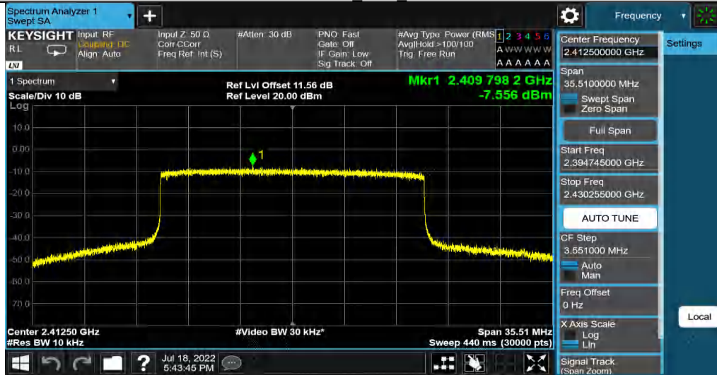
20M-MIMO Ant2 2412.5
