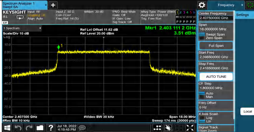
10M-MIMO Ant2 2407.5
