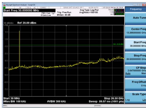
DQPSK-CH39 30MHz to 26.5GHz
