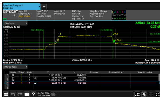
Figure 336 - 802.11ax HE80 SU Minimum 99% OBW
