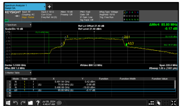
Figure 329 - 802.11ac VHT80 Maximum 99% OBW
