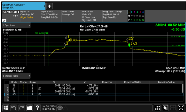
Figure 351 - 802.11ac VHT80 Maximum 99% OBW
