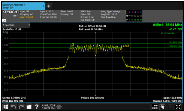
Figure 342 - 802.11ac VHT40 Minimum 6 dB EBW
