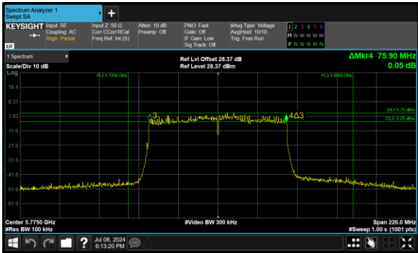
Figure 345 - 802.11ac VHT80 Maximum 6 dB EBW
