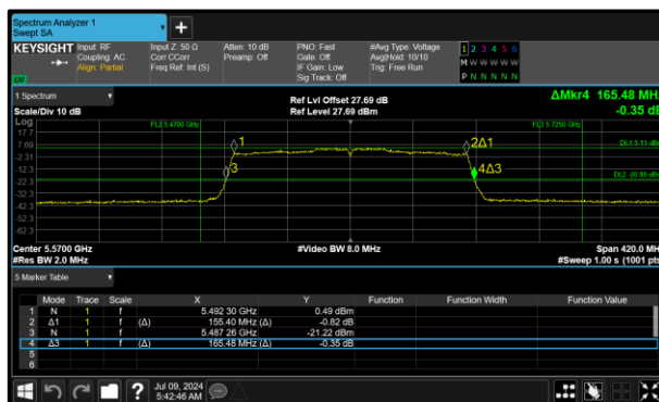
Figure 338 - 802.11ax HE160 SU Minimum 99% OBW
