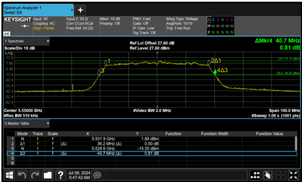
Figure 348 - 802.11ac VHT40 Minimum 99% OBW
