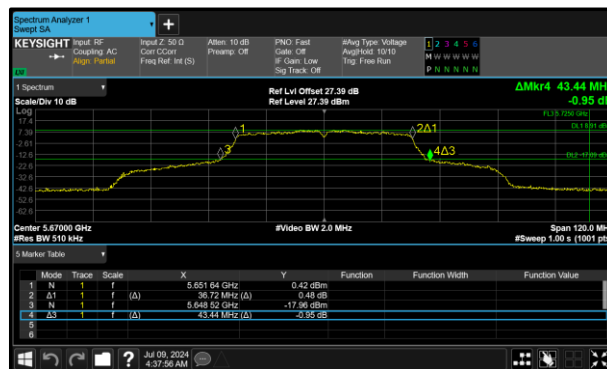
Figure 327 - 802.11n HT40 Maximum 99% OBW
