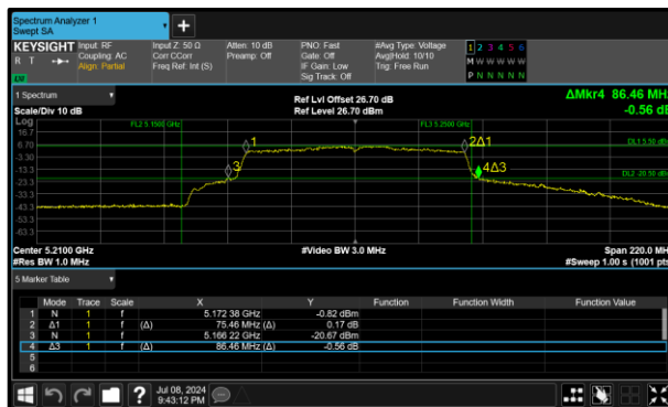
Figure 328 - 802.11ac VHT80 Minimum 99% OBW
