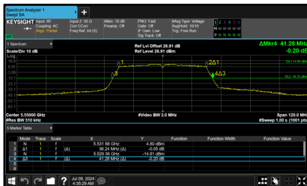
Figure 326 - 802.11n HT40 Minimum 99% OBW
