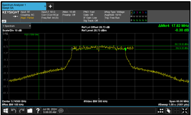
Figure 341 - 802.11ac VHT20 Maximum 6 dB EBW
