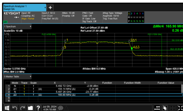
Figure 330 - 802.11ac VHT160 Minimum 99% OBW
