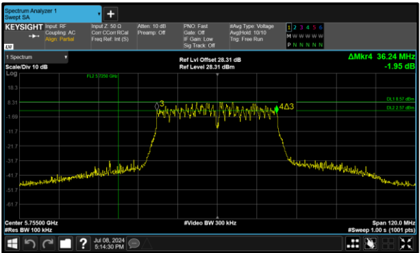
Figure 343 - 802.11ac VHT40 Maximum 6 dB EBW
