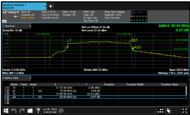
Figure 350 - 802.11ac VHT80 Minimum 99% OBW
