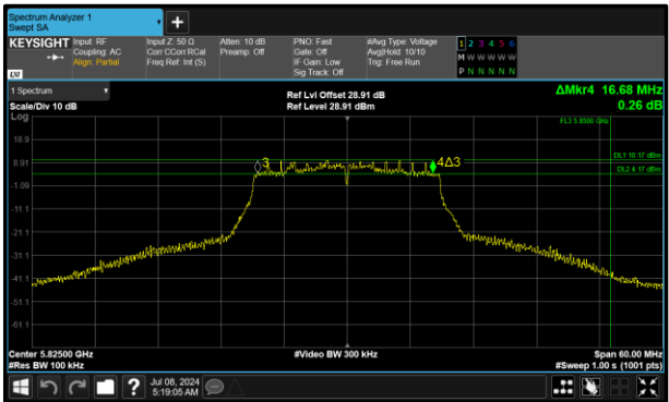
Figure 340 - 802.11ac VHT20 Minimum 6 dB EBW
