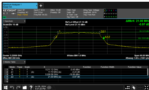
Figure 324 - 802.11n HT20 Minimum 99% OBW
