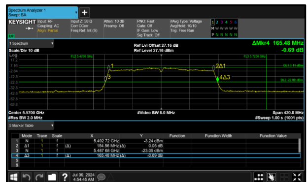
Figure 331 - 802.11ac VHT160 Maximum 99% OBW
