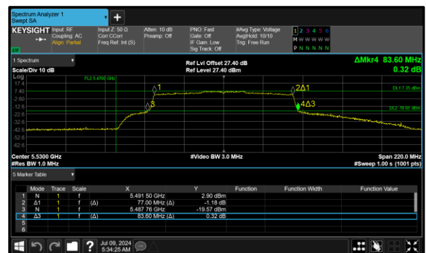
Figure 337 - 802.11ax HE80 SU Maximum 99% OBW
