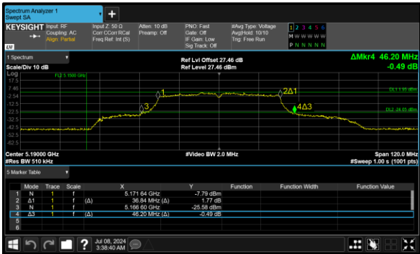
Figure 349 - 802.11ac VHT40 Maximum 99% OBW
