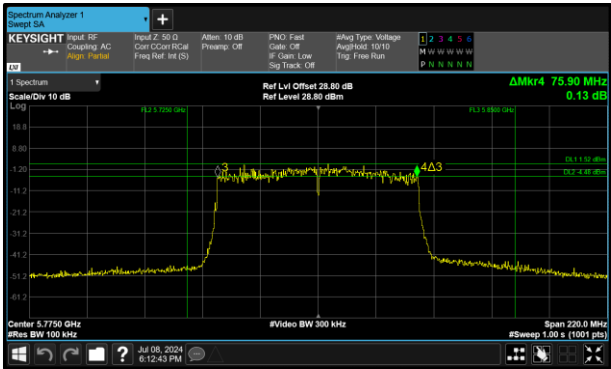
Figure 344 - 802.11ac VHT80 Minimum 6 dB EBW
