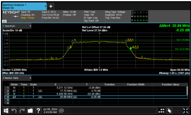
Figure 346 - 802.11ac VHT20 Minimum 99% OBW
