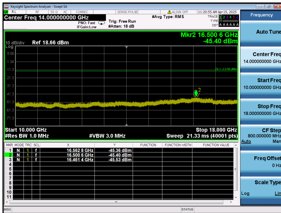
LTE Band 66 / 10MHz / 16QAM - RB Size/Offset (50/0) - Low Channel
