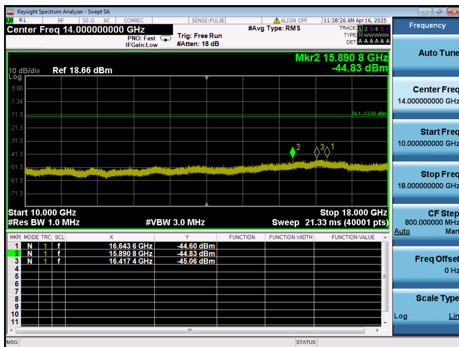
LTE Band 66 / 20MHz / QPSK - RB Size/Offset (100/0) - Mid Channel
