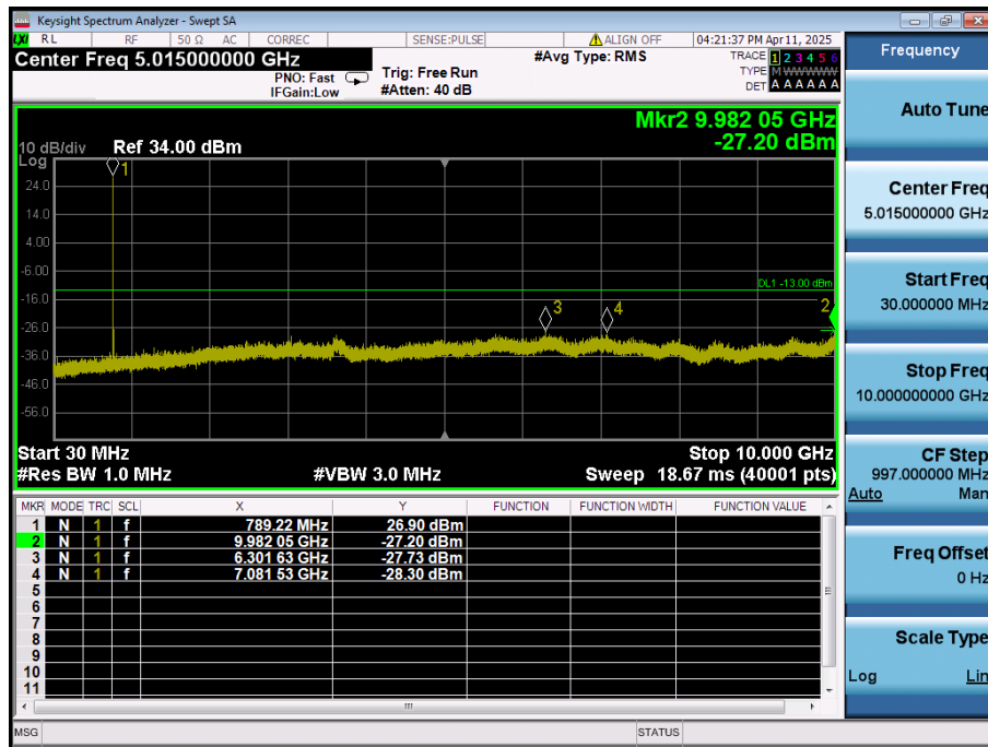
LTE Band 14 / 10MHz / 16QAM - RB Size/Offset (1/0) - Low Channel
