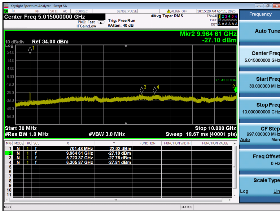
LTE Band 12 / 5MHz / QPSK - RB Size/Offset (25/0) - Low Channel
