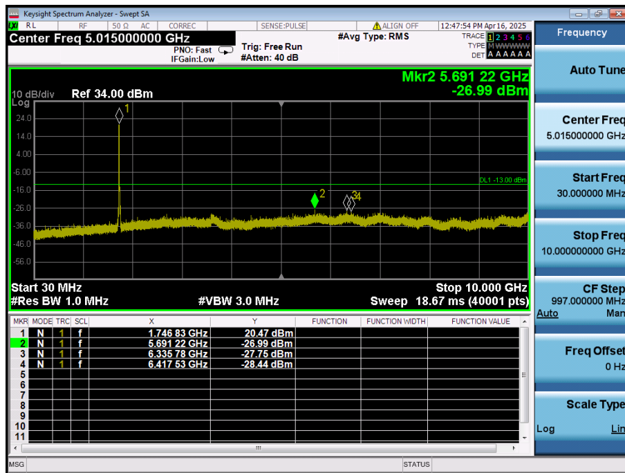
LTE Band 66 / 10MHz / 16QAM - RB Size/Offset (50/0) - Mid Channel
