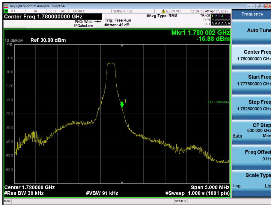
LTE Band 66 / 1.4MHz / 16QAM - RB Size/Offset (1/5)
