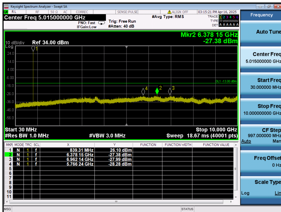
LTE Band 5 / 5MHz / QPSK - RB Size/Offset (1/24) - Mid Channel
