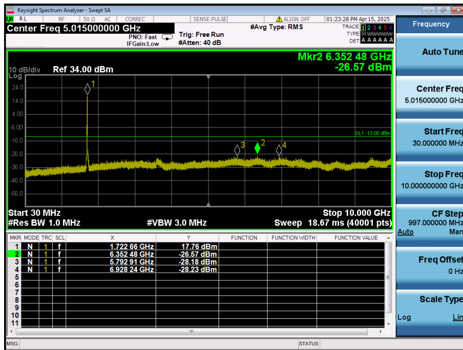
LTE Band 66 / 15MHz / 64QAM - RB Size/Offset (75/0) - Low Channel
