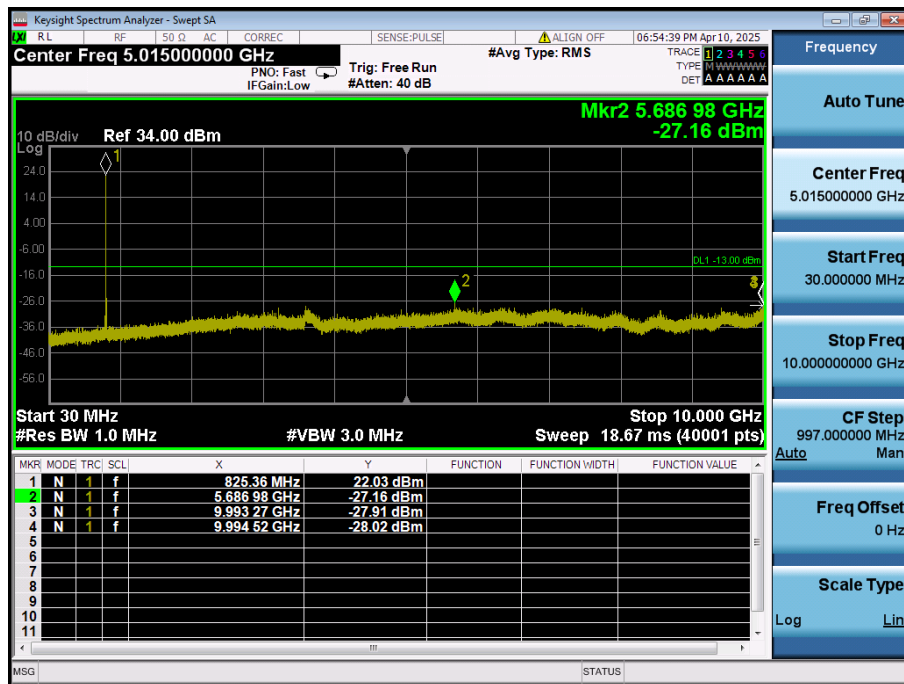
LTE Band 5 / 3MHz / 64QAM - RB Size/Offset (1/7) - Low Channel
