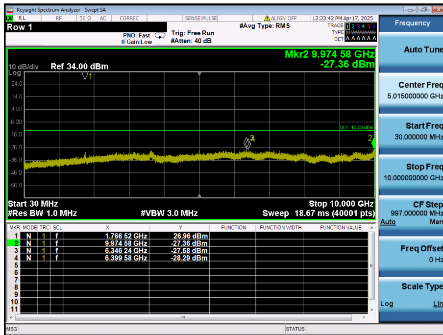
LTE Band 66 / 15MHz / QPSK - RB Size/Offset (1/0) - High Channel
