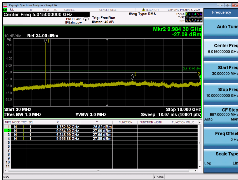
LTE Band 66 / 5MHz / 64QAM - RB Size/Offset (1/24) - Mid Channel
