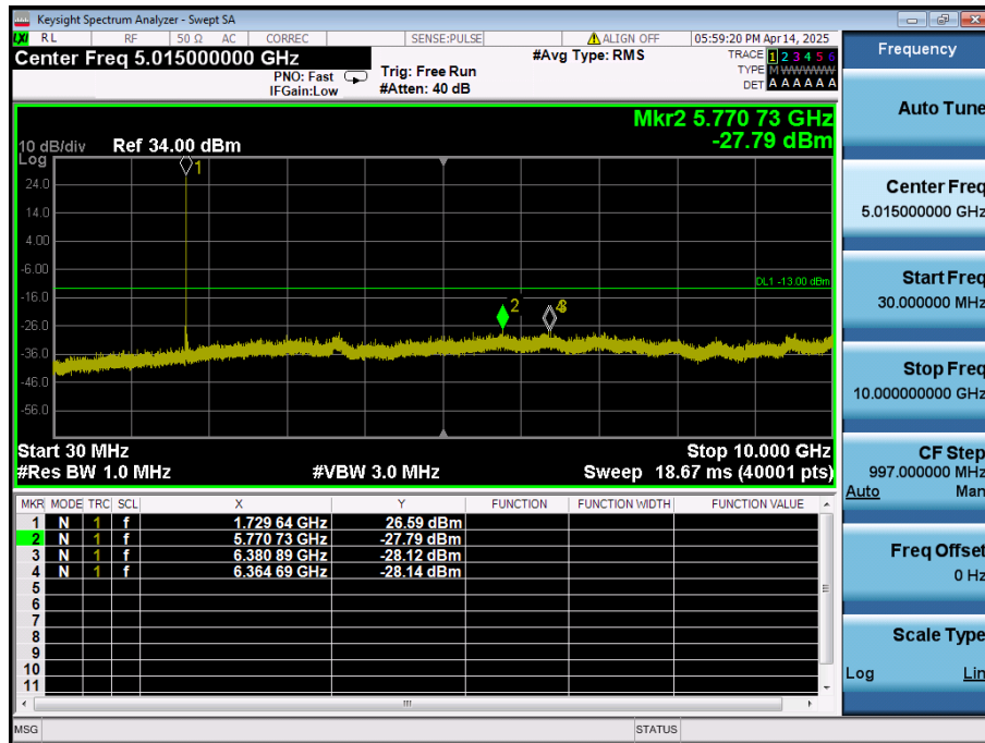
LTE Band 66 / 20MHz / QPSK - RB Size/Offset (1/99) - Low Channel
