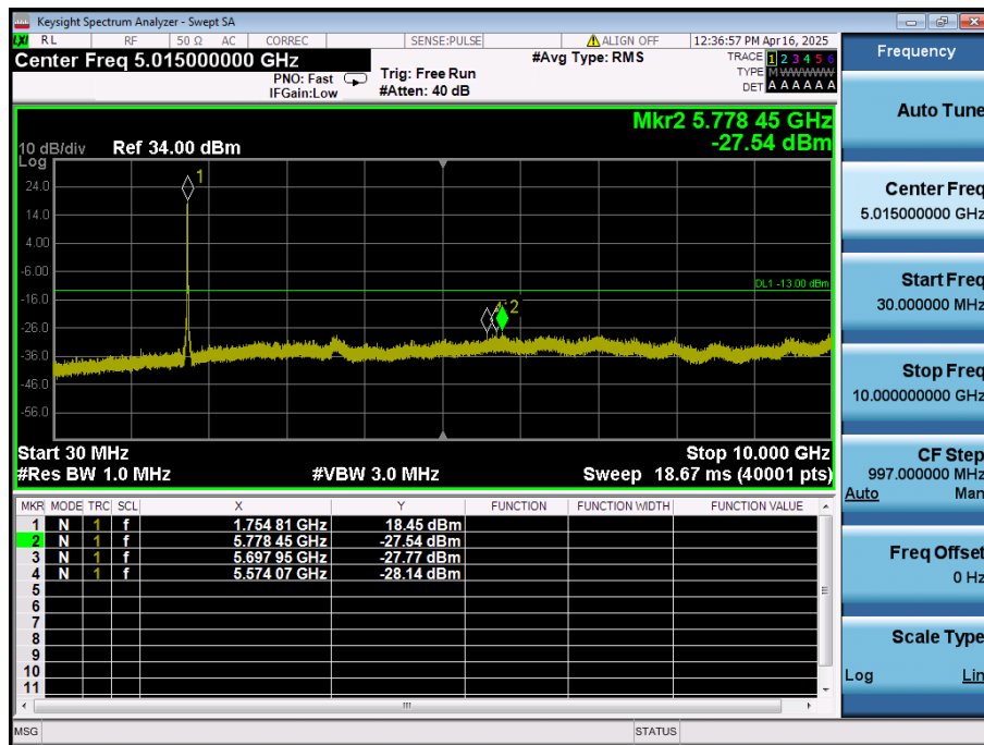
LTE Band 66 / 15MHz / 16QAM - RB Size/Offset (75/0) - Mid Channel
