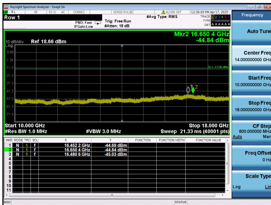
LTE Band 66 / 10MHz / QPSK - RB Size/Offset (1/12) - High Channel
