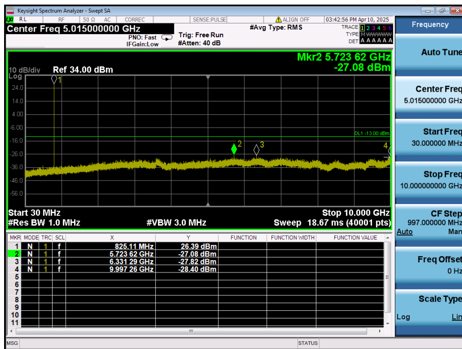
LTE Band 5 / 5MHz / QPSK - RB Size/Offset (1/0) - Low Channel
