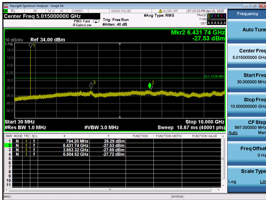
LTE Band 14 / 5MHz / 16QAM - RB Size/Offset (12/6) - Mid Channel
