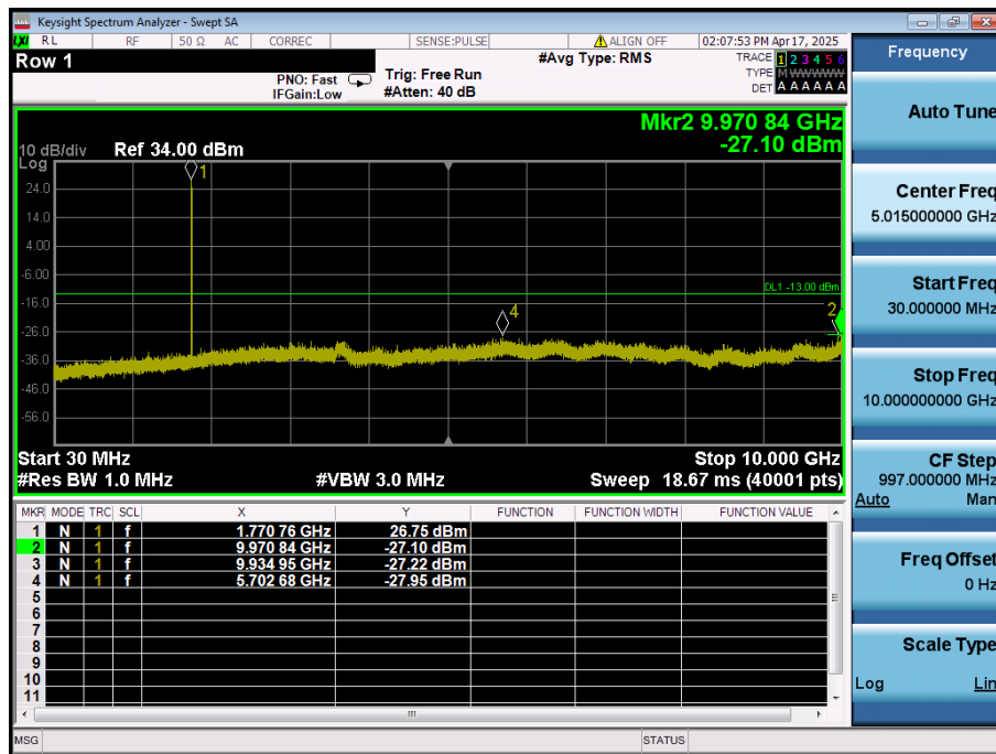
LTE Band 66 / 20MHz / 16QAM - RB Size/Offset (1/50) - High Channel
