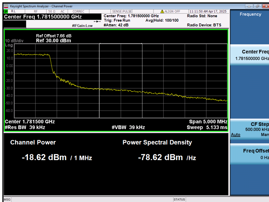
LTE Band 66 / 1.4MHz / 16QAM - RB Size/Offset (6/0)
