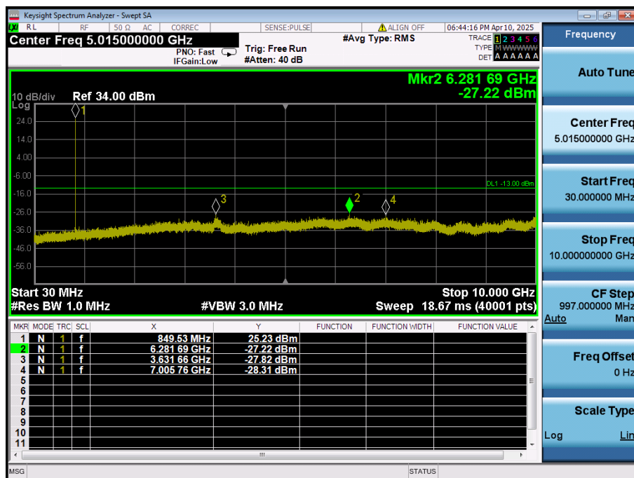
LTE Band 5 / 5MHz / 64QAM - RB Size/Offset (1/24) - High Channel
