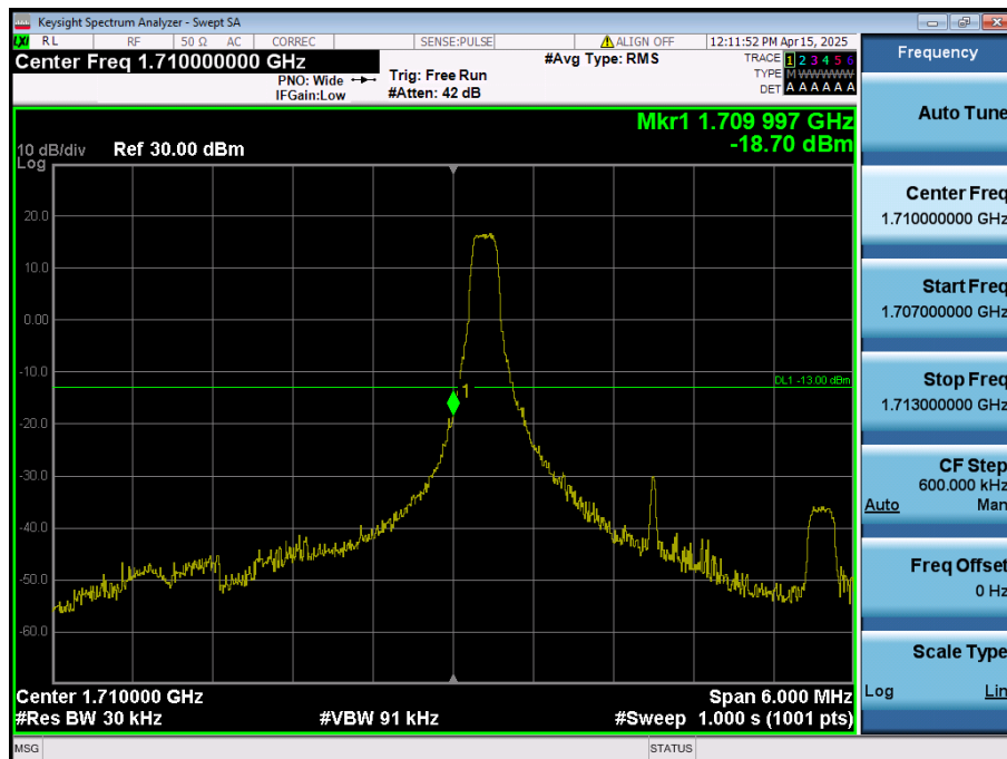
LTE Band 66 / 3MHz / 16QAM - RB Size/Offset (1/0)
