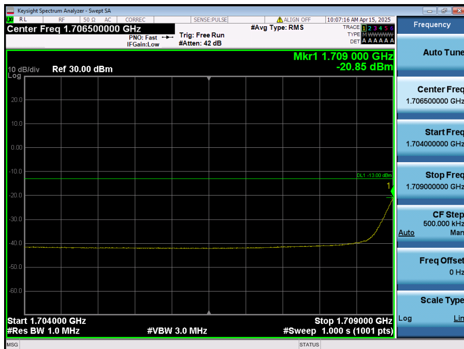
LTE Band 66 / 1.4MHz / QPSK - RB Size/Offset (1/2)
