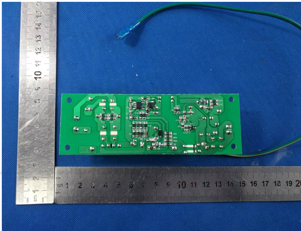
(Built-in Power Board: BI67-160410-O3)
