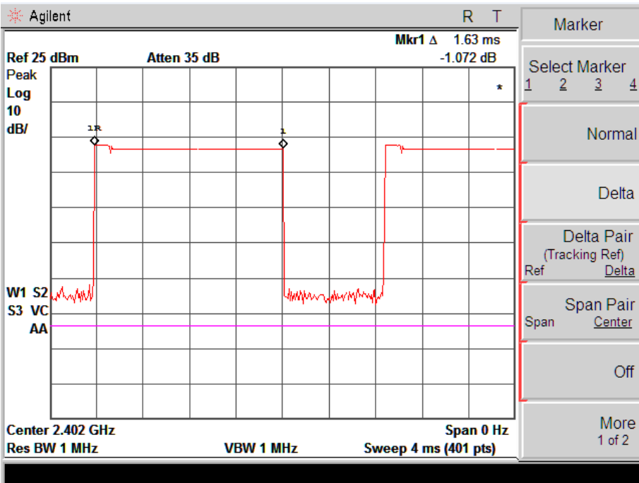
Pi/4 DQPSK 2DH3 time slot (Low, Middle, High Channels)
