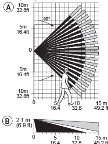
Figure 4. Coverage Pattern & Walk-test Up to 40 kg (90 lb)
