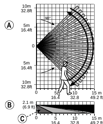
Fig. 5. Coverage Pattern & Walk-test
