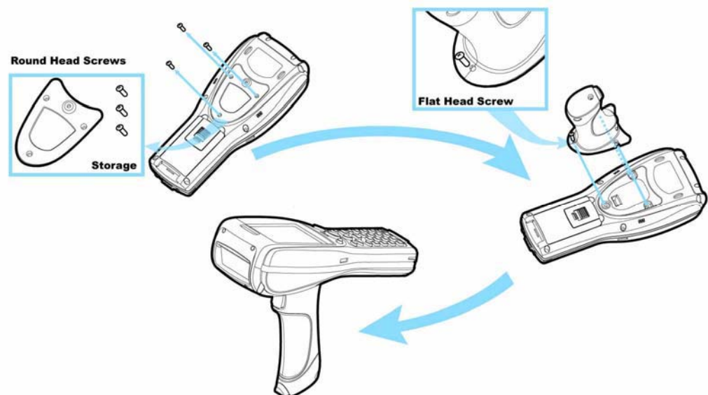
Figure 6: Installing pistol grip
