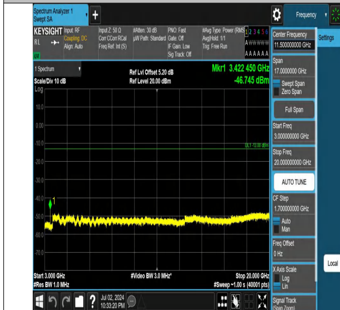
Band4-20MHz-QPSK-20050-1RB#0-3000~20000-PASS
