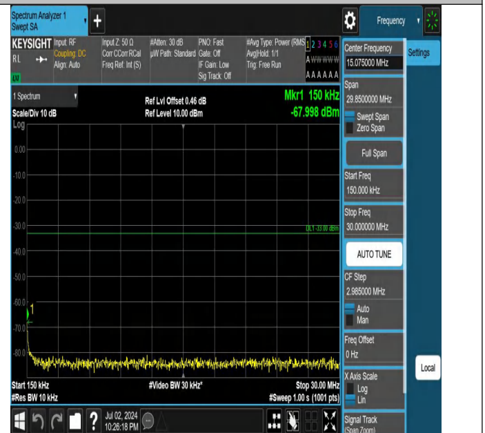
Band4-10MHz-QPSK-20000-1RB#0-0.15~30-PASS
