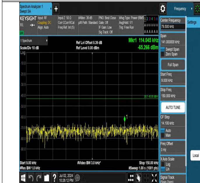
Band4-10MHz-QPSK-20000-1RB#0-0.009~0.15-PASS
