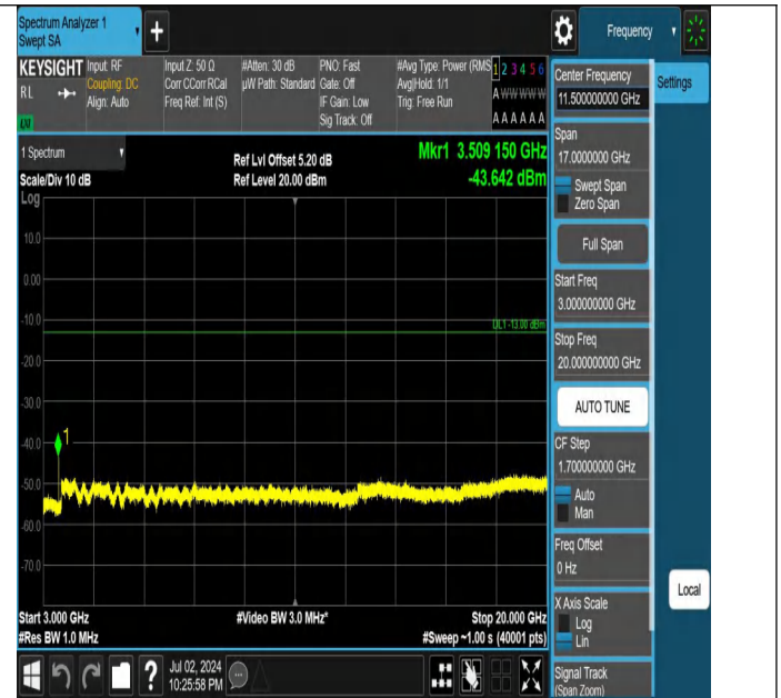
Band4-5MHz-QPSK-20375-1RB#24-3000~20000-PASS
