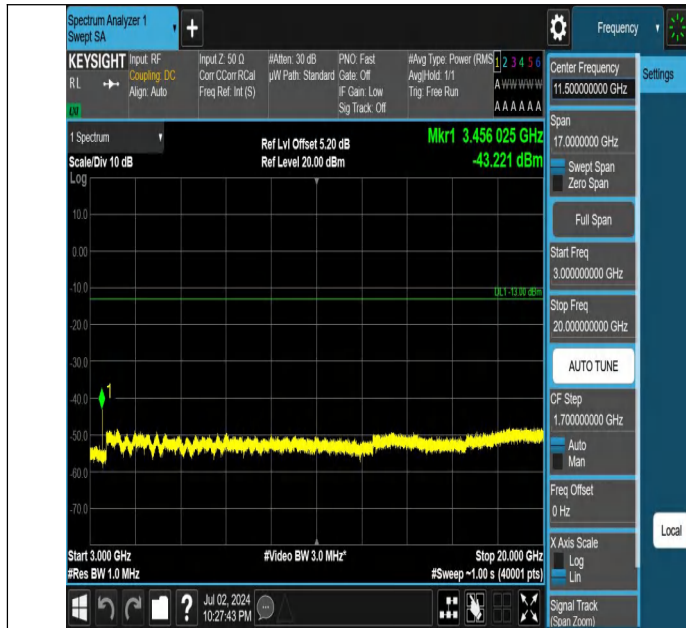
Band4-10MHz-QPSK-20175-1RB#0-3000~20000-PASS
