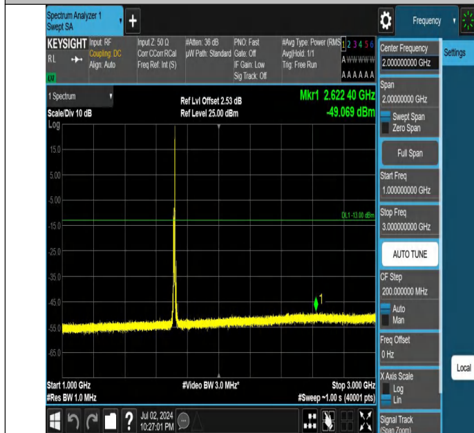
Band4-10MHz-QPSK-20000-1RB#49-1000~3000-PASS
