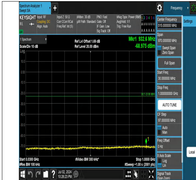
Band4-10MHz-QPSK-20000-1RB#0-30~1000-PASS
