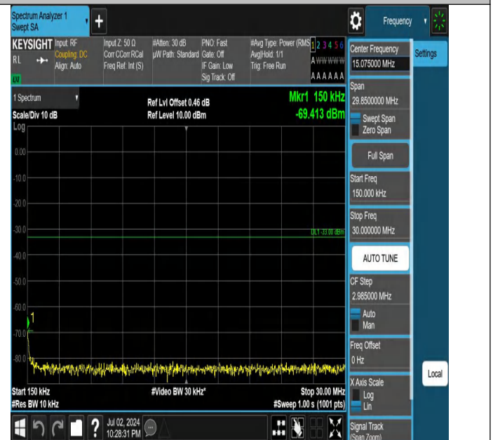
Band4-10MHz-QPSK-20350-1RB#0-0.15~30-PASS
