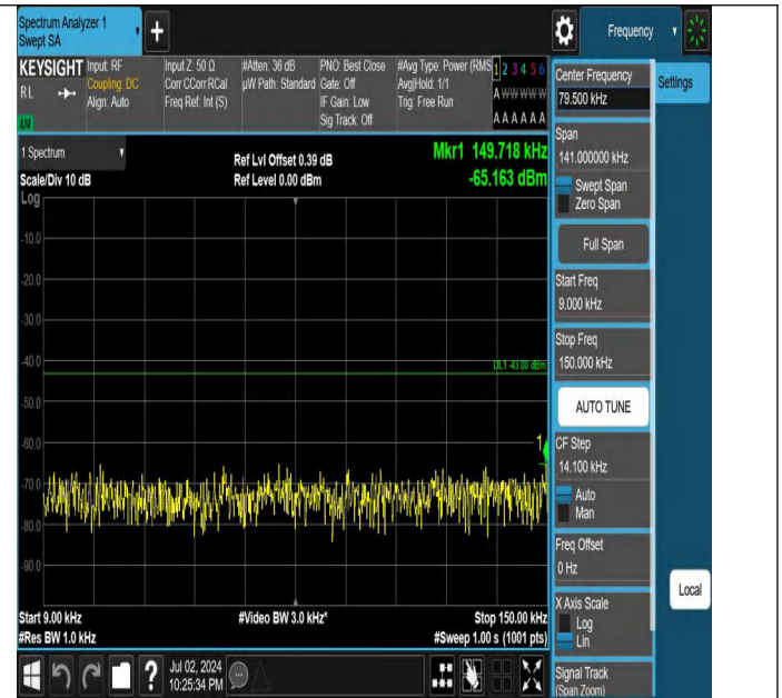
Band4-5MHz-QPSK-20375-1RB#24-0.009~0.15-PASS
