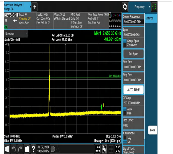
Band4-10MHz-QPSK-20000-1RB#0-1000~3000-PASS
