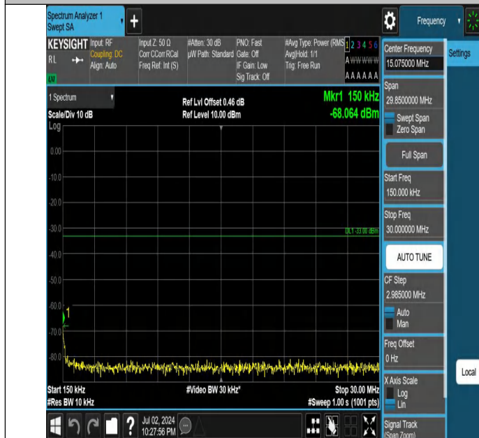
Band4-10MHz-QPSK-20175-1RB#49-0.15~30-PASS
