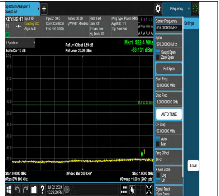
Band4-10MHz-QPSK-20350-1RB#49-30~1000-PASS
