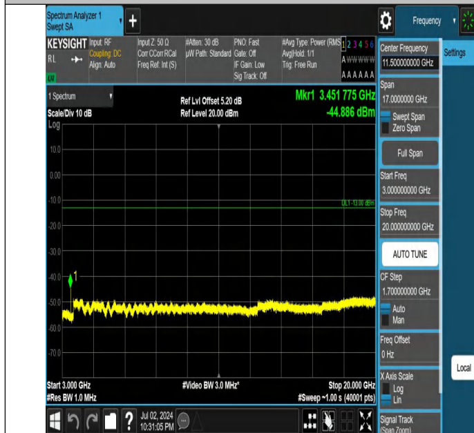
Band4-15MHz-QPSK-20175-1RB#0-3000~20000-PASS
