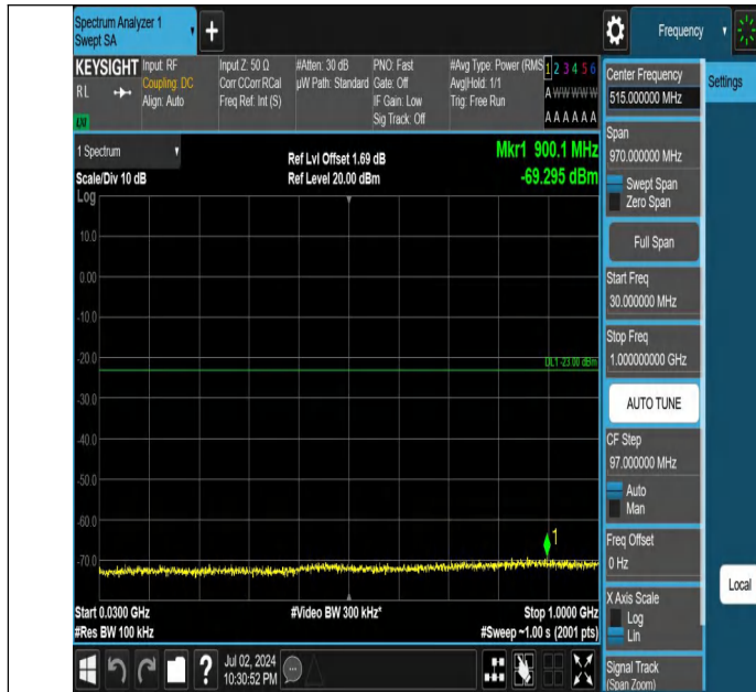
Band4-15MHz-QPSK-20175-1RB#0-30~1000-PASS
