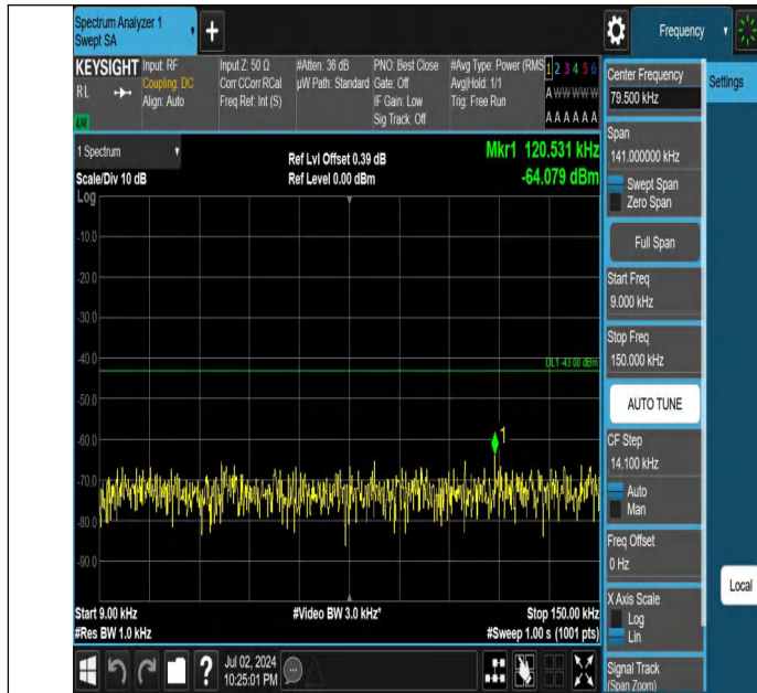
Band4-5MHz-QPSK-20375-1RB#0-0.009~0.15-PASS
