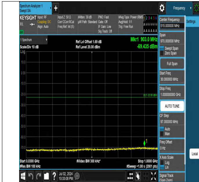
Band4-20MHz-QPSK-20050-1RB#0-30~1000-PASS
