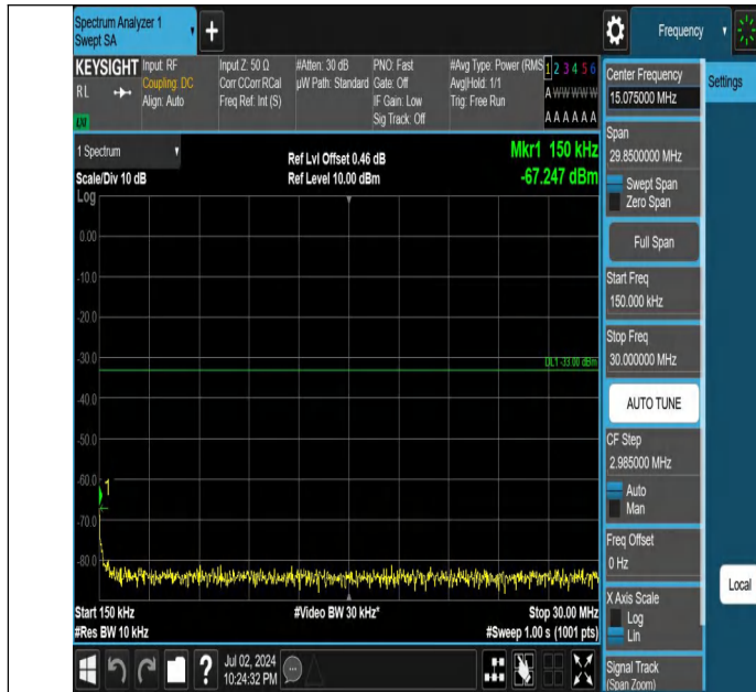
Band4-5MHz-QPSK-20175-1RB#24-0.15~30-PASS
