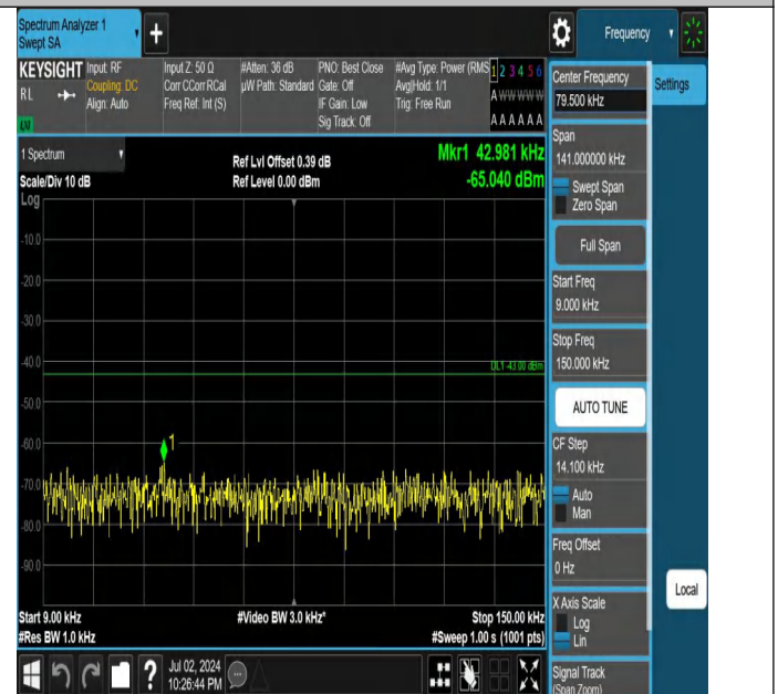
Band4-10MHz-QPSK-20000-1RB#49-0.009~0.15-PASS
