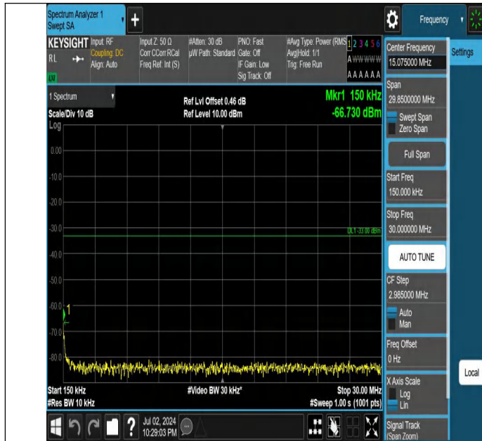
Band4-10MHz-QPSK-20350-1RB#49-0.15~30-PASS
