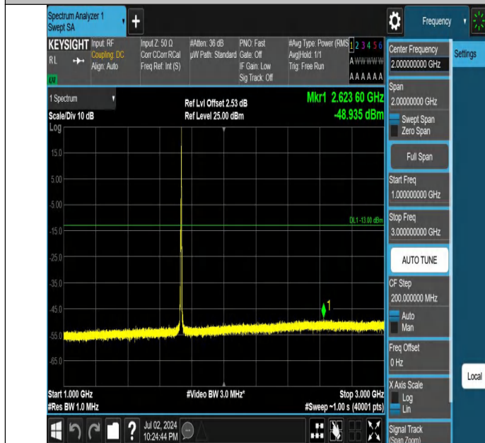
Band4-5MHz-QPSK-20175-1RB#24-1000~3000-PASS
