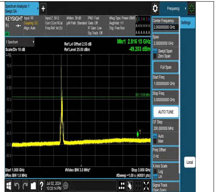
Band4-20MHz-QPSK-20050-1RB#0-1000~3000-PASS
