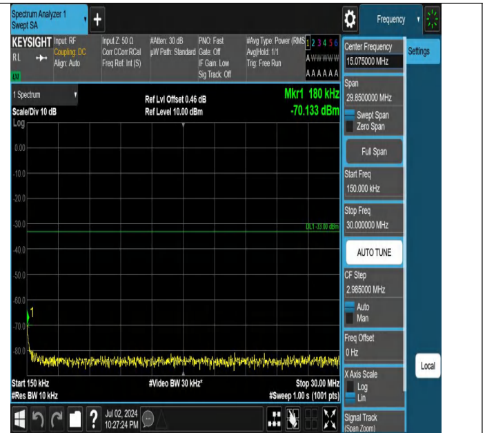
Band4-10MHz-QPSK-20175-1RB#0-0.15~30-PASS
