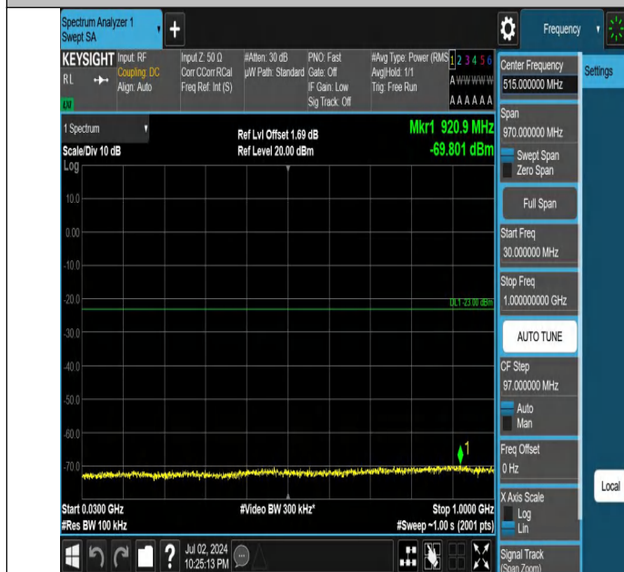
Band4-5MHz-QPSK-20375-1RB#0-30~1000-PASS
