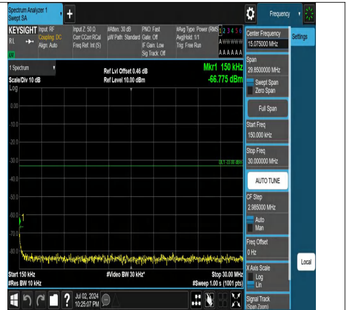
Band4-5MHz-QPSK-20375-1RB#0-0.15~30-PASS
