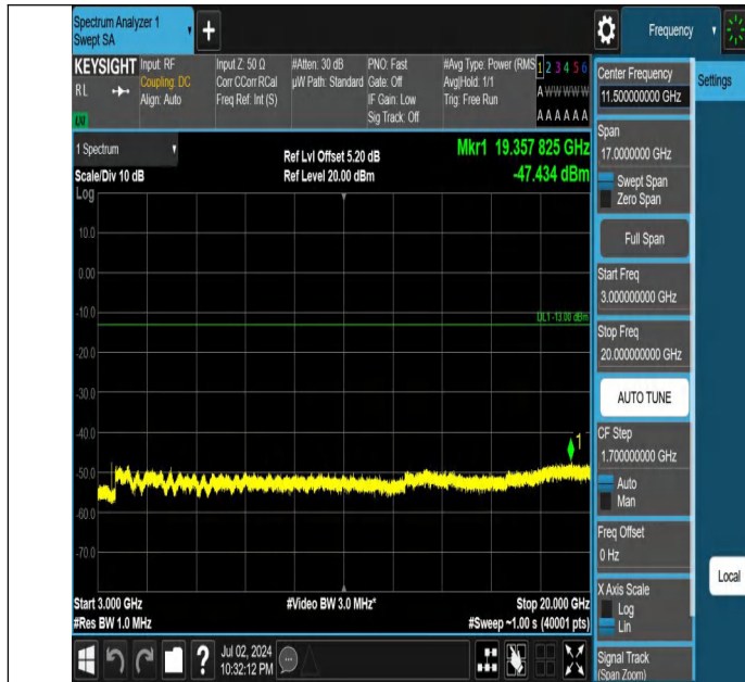
Band4-15MHz-QPSK-20325-1RB#0-3000~20000-PASS
