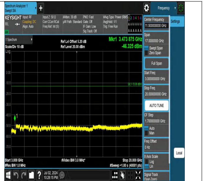
Band4-10MHz-QPSK-20175-1RB#49-3000~20000-PASS
