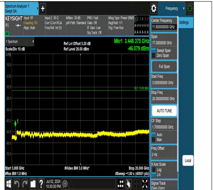
Band4-15MHz-QPSK-20025-1RB#74-3000~20000-PASS
