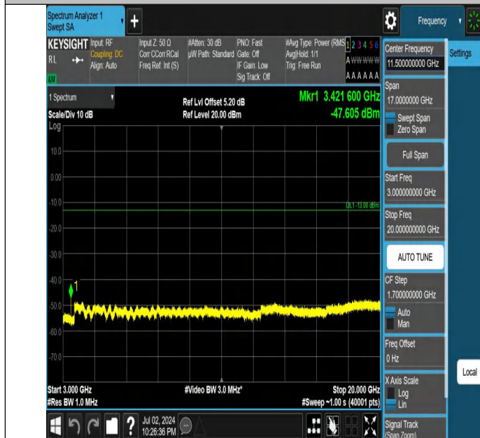
Band4-10MHz-QPSK-20000-1RB#0-3000~20000-PASS
