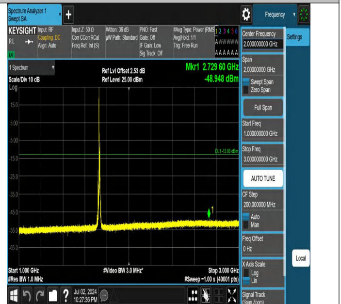
Band4-10MHz-QPSK-20175-1RB#0-1000~3000-PASS
