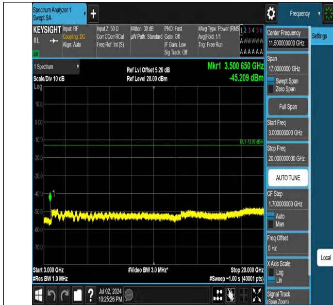
Band4-5MHz-QPSK-20375-1RB#0-3000~20000-PASS
