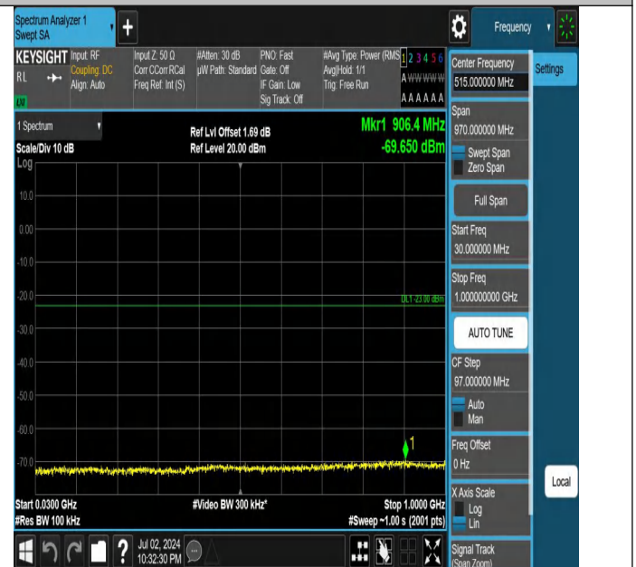
Band4-15MHz-QPSK-20325-1RB#74-30~1000-PASS
