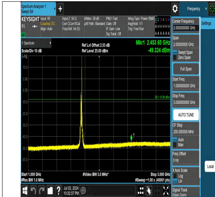
Band4-15MHz-QPSK-20325-1RB#74-1000~3000-PASS
