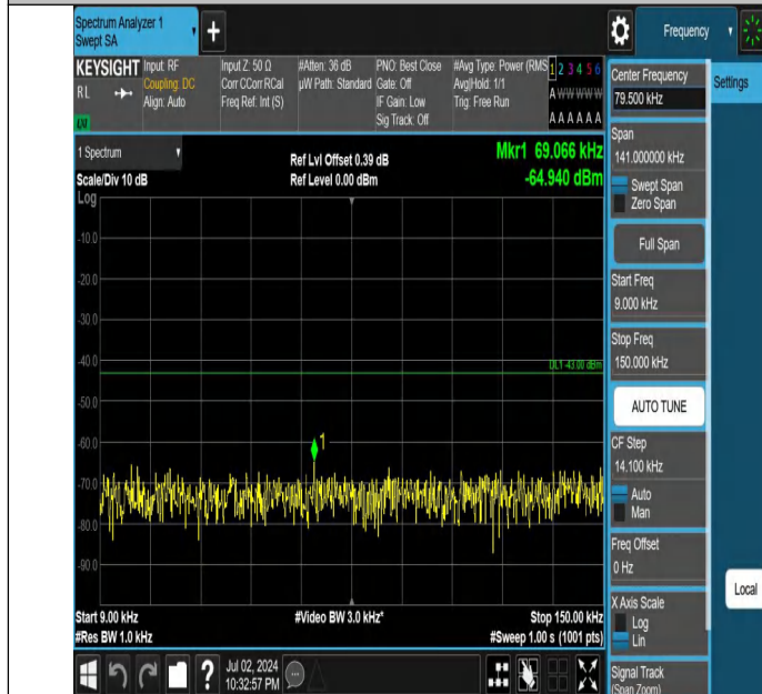
Band4-20MHz-QPSK-20050-1RB#0-0.009~0.15-PASS
