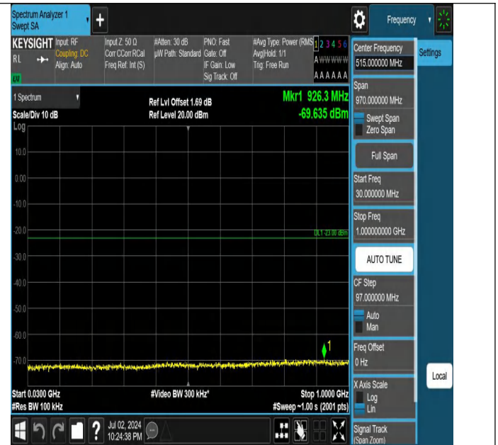
Band4-5MHz-QPSK-20175-1RB#24-30~1000-PASS
