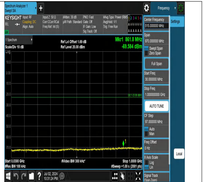
Band4-15MHz-QPSK-20175-1RB#74-30~1000-PASS
