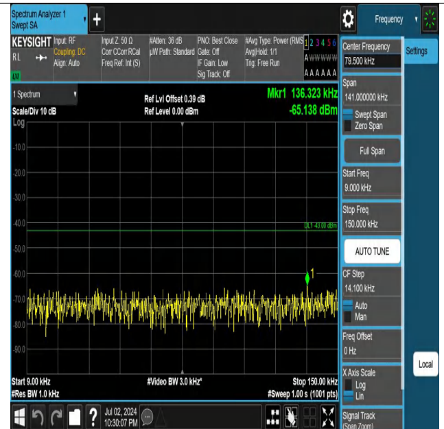
Band4-15MHz-QPSK-20025-1RB#74-0.009~0.15-PASS
