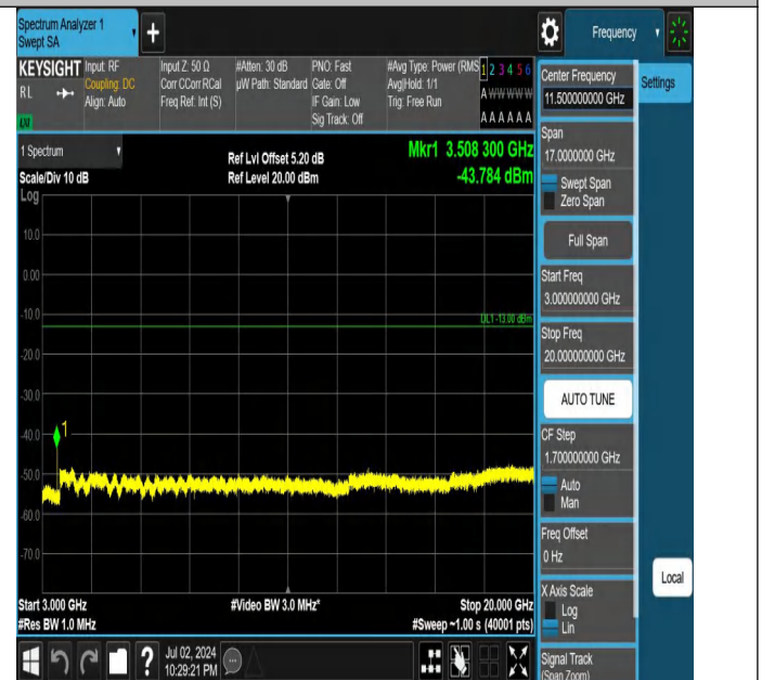
Band4-10MHz-QPSK-20350-1RB#49-3000~20000-PASS
