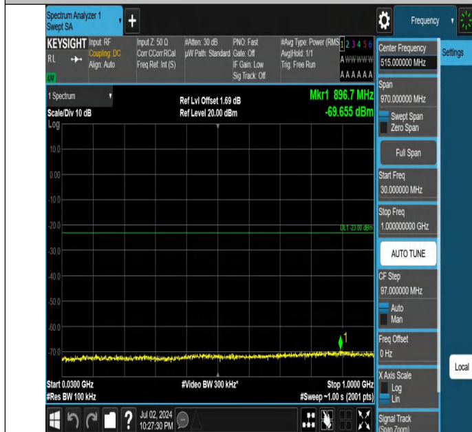
Band4-10MHz-QPSK-20175-1RB#0-30~1000-PASS
