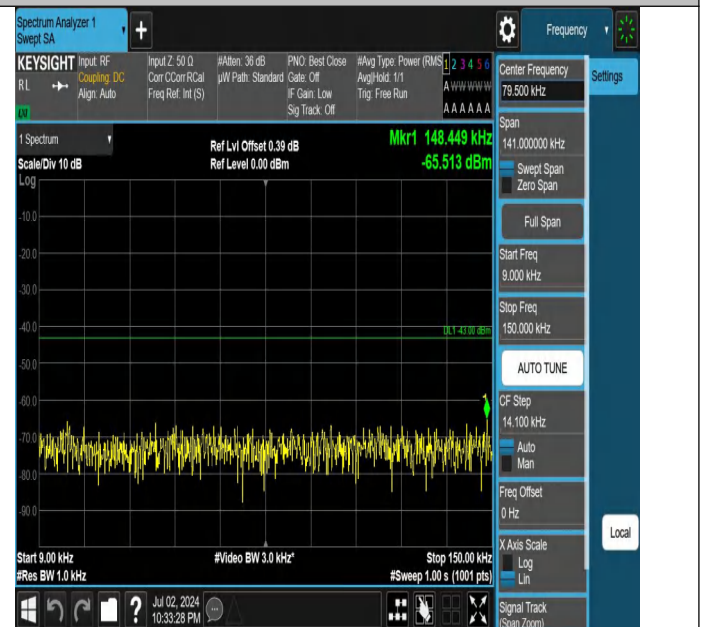
Band4-20MHz-QPSK-20050-1RB#99-0.009~0.15-PASS
