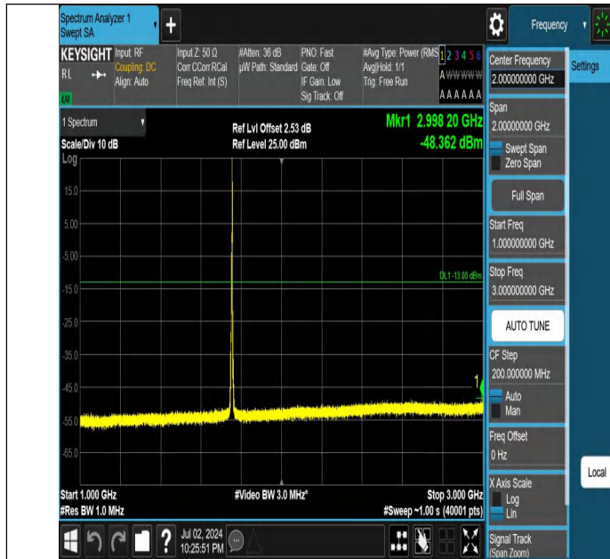
Band4-5MHz-QPSK-20375-1RB#24-1000~3000-PASS
