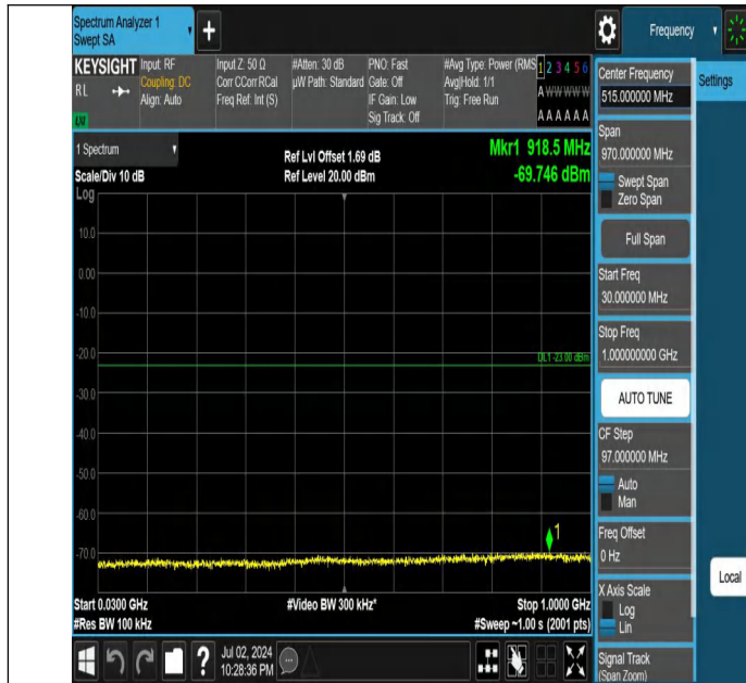
Band4-10MHz-QPSK-20350-1RB#0-30~1000-PASS
