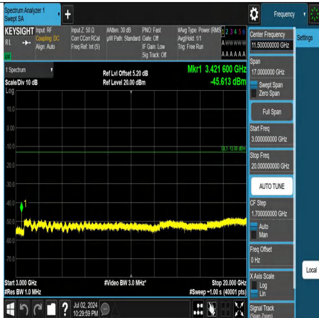
Band4-15MHz-QPSK-20025-1RB#0-3000~20000-PASS
