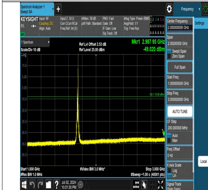
Band4-15MHz-QPSK-20175-1RB#74-1000~3000-PASS
