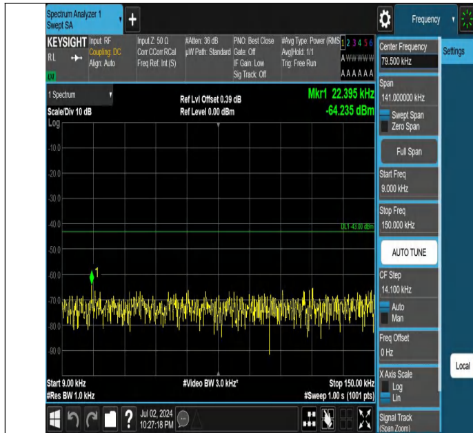
Band4-10MHz-QPSK-20175-1RB#0-0.009~0.15-PASS
