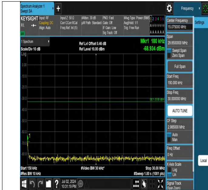
Band4-15MHz-QPSK-20175-1RB#74-0.15~30-PASS
