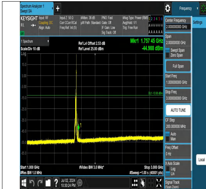
Band4-15MHz-QPSK-20025-1RB#74-1000~3000-PASS
