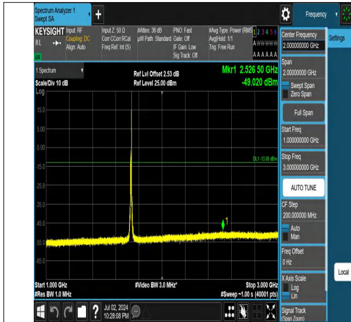
Band4-10MHz-QPSK-20175-1RB#49-1000~3000-PASS
