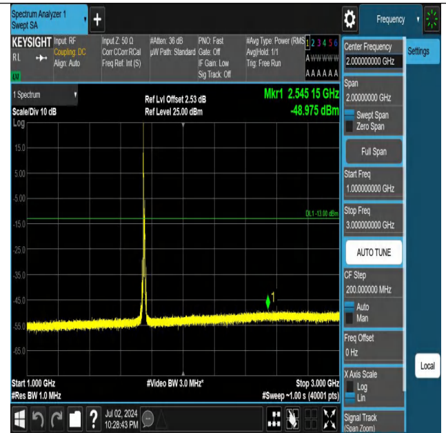
Band4-10MHz-QPSK-20350-1RB#0-1000~3000-PASS
