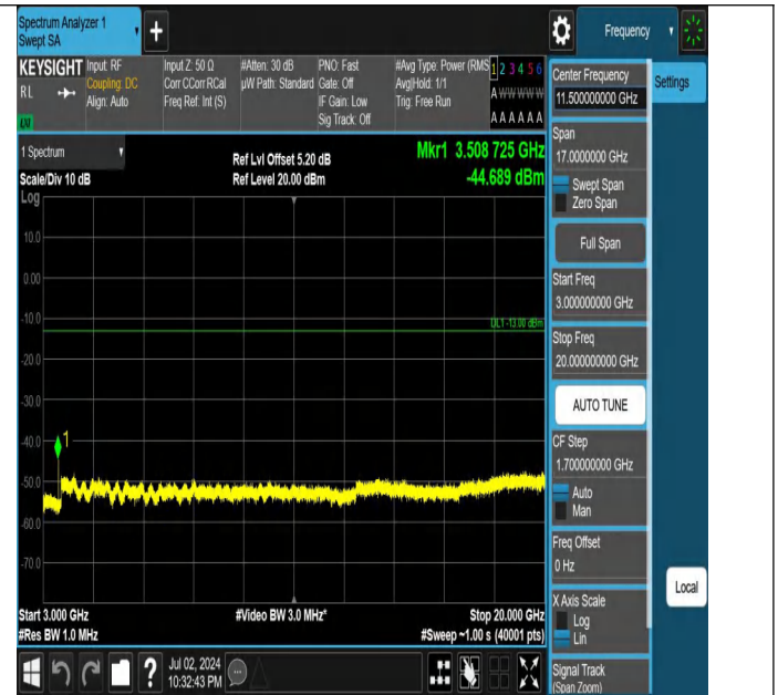
Band4-15MHz-QPSK-20325-1RB#74-3000~20000-PASS
