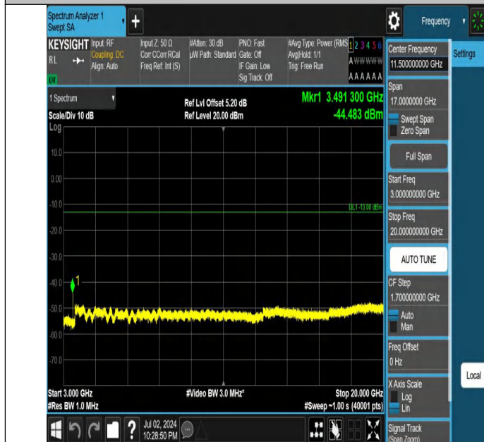
Band4-10MHz-QPSK-20350-1RB#0-3000~20000-PASS
