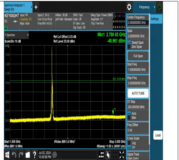
Band4-15MHz-QPSK-20175-1RB#0-1000~3000-PASS
