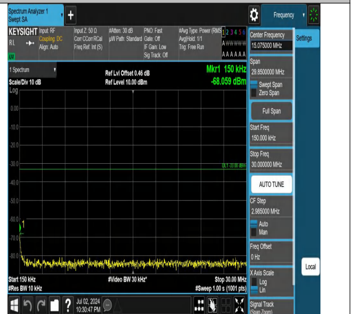
Band4-15MHz-QPSK-20175-1RB#0-0.15~30-PASS
