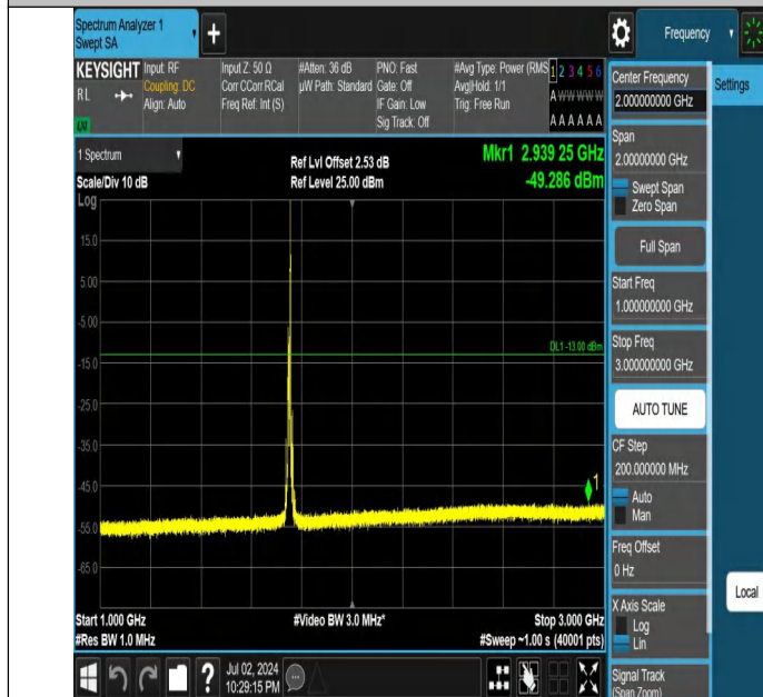
Band4-10MHz-QPSK-20350-1RB#49-1000~3000-PASS
