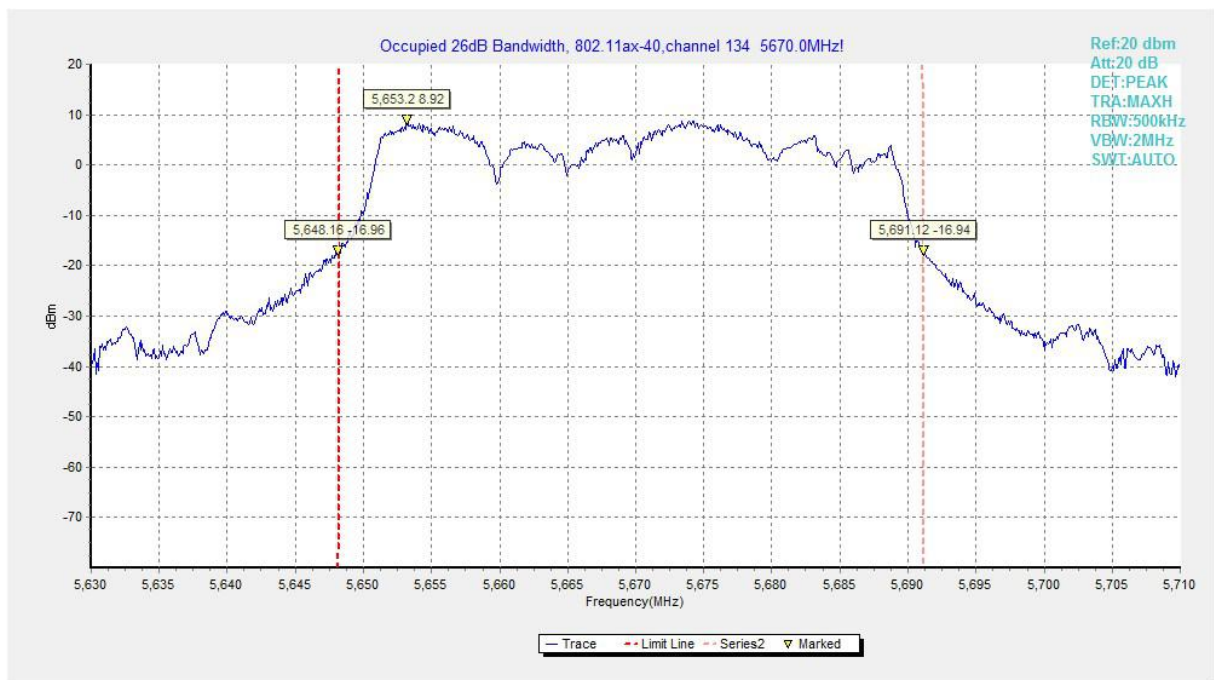
Fig.143 Occupied 26dB Bandwidth (802.11ax-HE40, 5670MHz)
