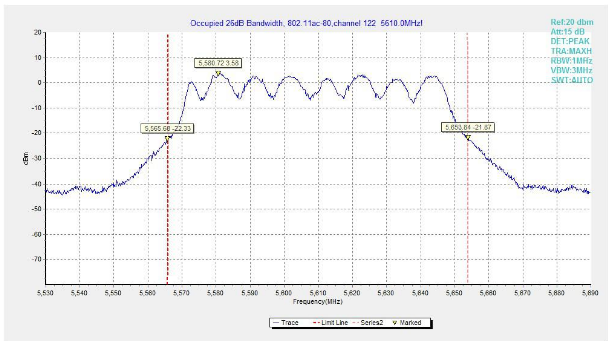
Fig.127 Occupied 26dB Bandwidth (802.11ac-HT80, 5610MHz)
