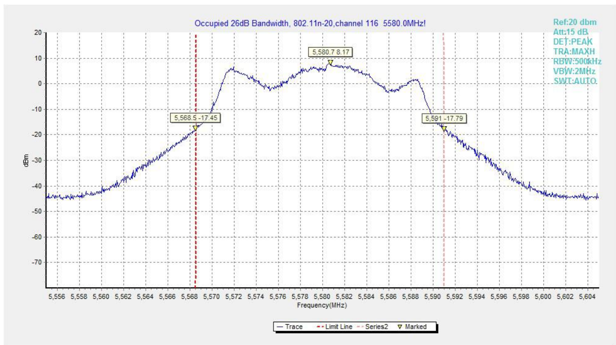
Fig.115 Occupied 26dB Bandwidth (802. 11n-HT20, 5580MHz)
