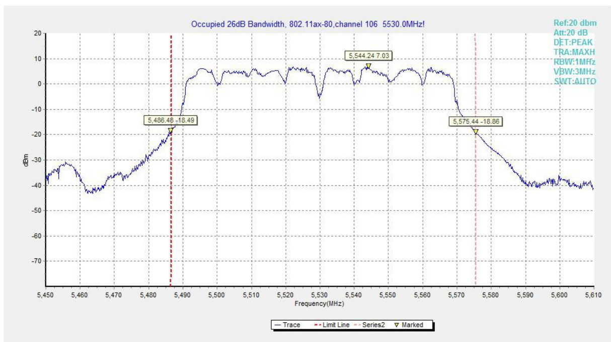
Fig.146 Occupied 26dB Bandwidth (802.11ax-HE80,5530MHz)
