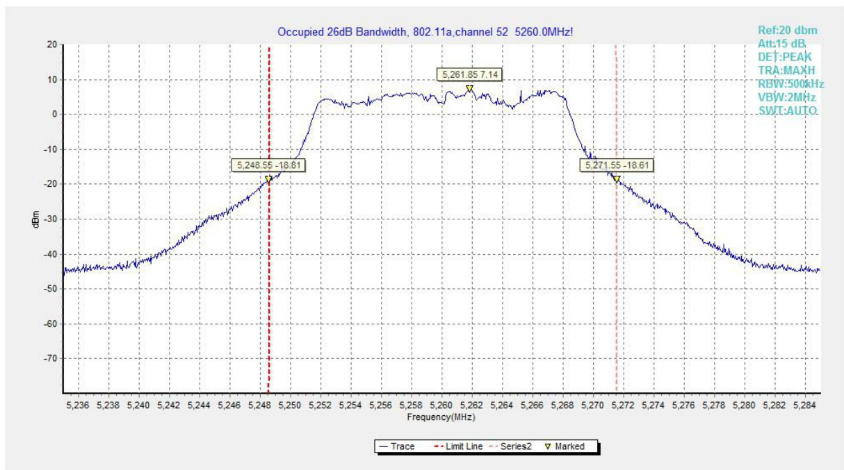
Fig.102 Occupied 26dB Bandwidth (802.11a, 5260MHz)
