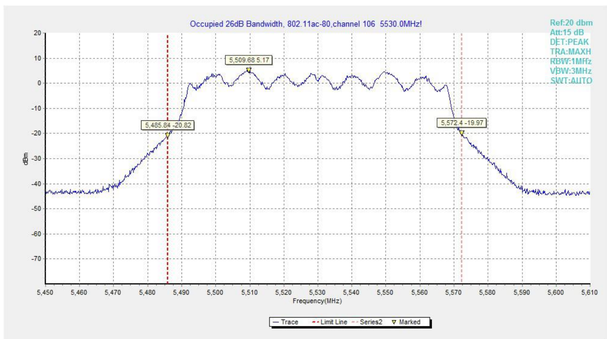
Fig.126 Occupied 26dB Bandwidth (802. 11ac-HT80, 5530MHz)
