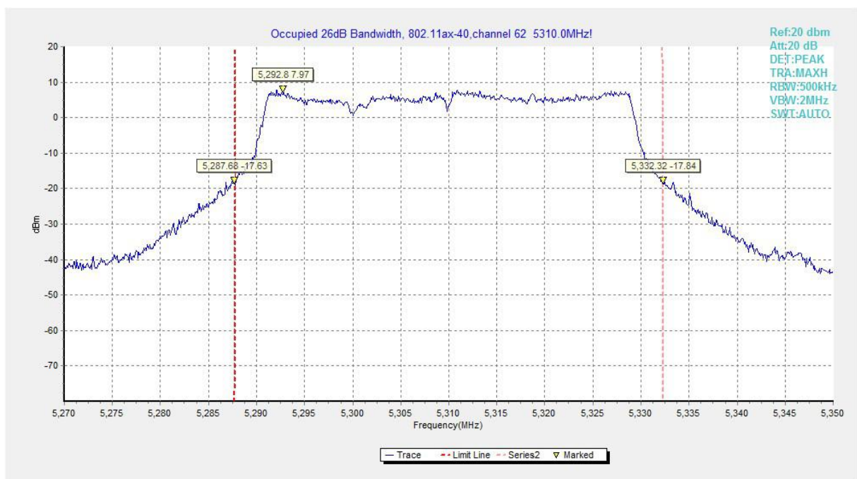
Fig.140 Occupied 26dB Bandwidth (802.11ax-HE40,5310MHz)
