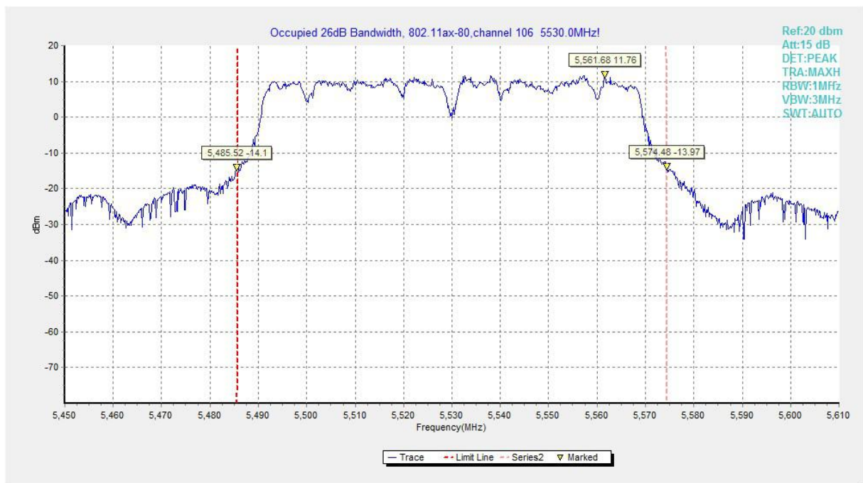
Fig.97 Occupied 26dB Bandwidth (802.11ax-HE80,5530MHz)
