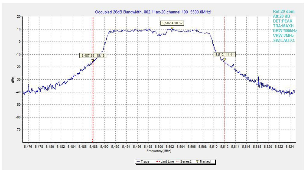
Fig.134 Occupied 26dB Bandwidth (802.11ax-HE20, 5500MHz)
