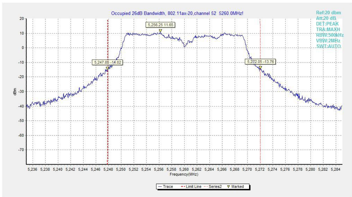
Fig.131 Occupied 26dB Bandwidth (802.11ax-HE20, 5260MHz)
