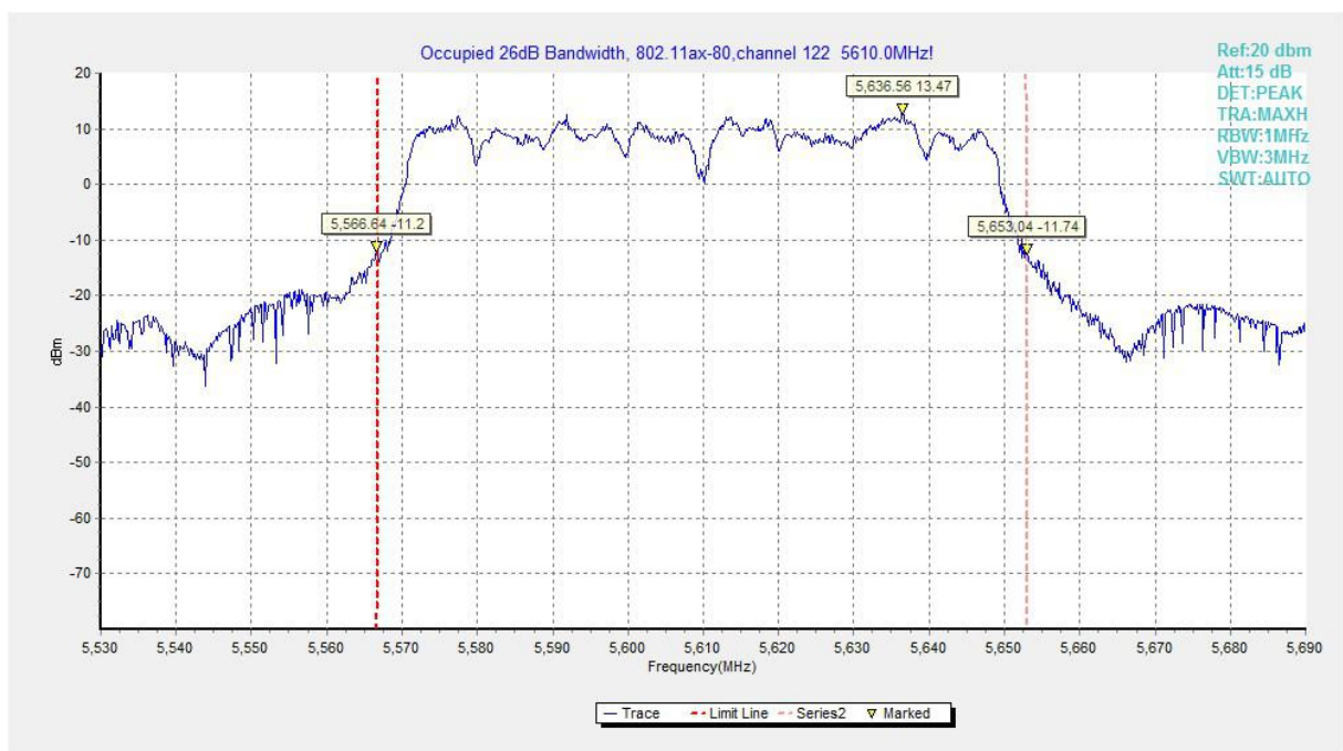
Fig.98 Occupied 26dB Bandwidth (802.11ax-HE80, 5610MHz)
