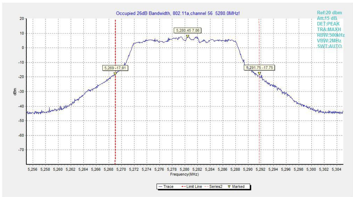
Fig.103 Occupied 26dB Bandwidth (802.11a, 5280MHz)
