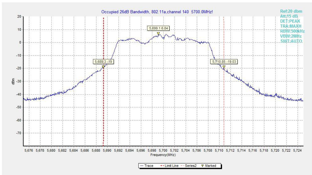
Fig.107 Occupied 26dB Bandwidth (802.11a, 5700MHz)
