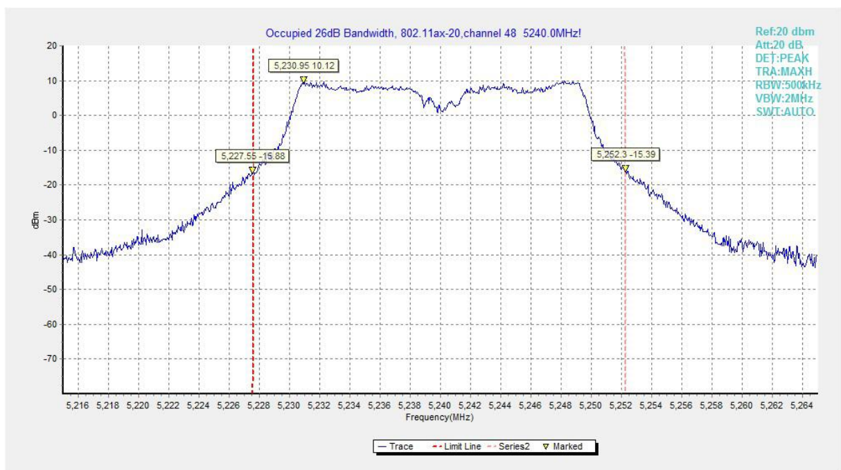
Fig.130 Occupied 26dB Bandwidth (802.11ax-HE20, 5240MHz)
