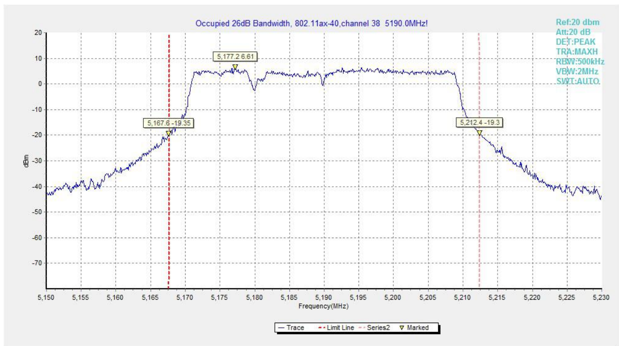
Fig.137 Occupied 26dB Bandwidth (802.11ax-HE40, 5190MHz)
