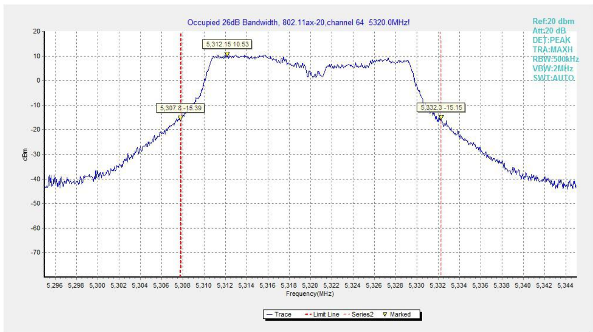
Fig.133 Occupied 26dB Bandwidth (802.11ax-HE20, 5320MHz)
