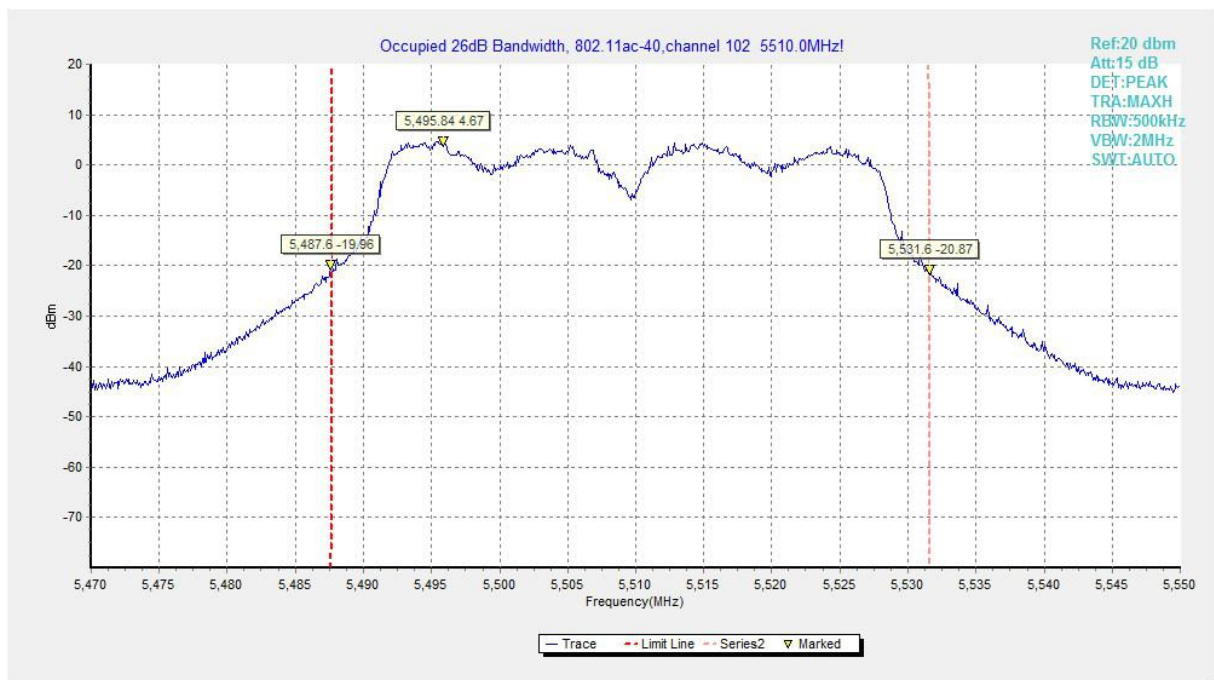
Fig.121 Occupied 26dB Bandwidth (802.11ac-HT40, 5510MHz)
