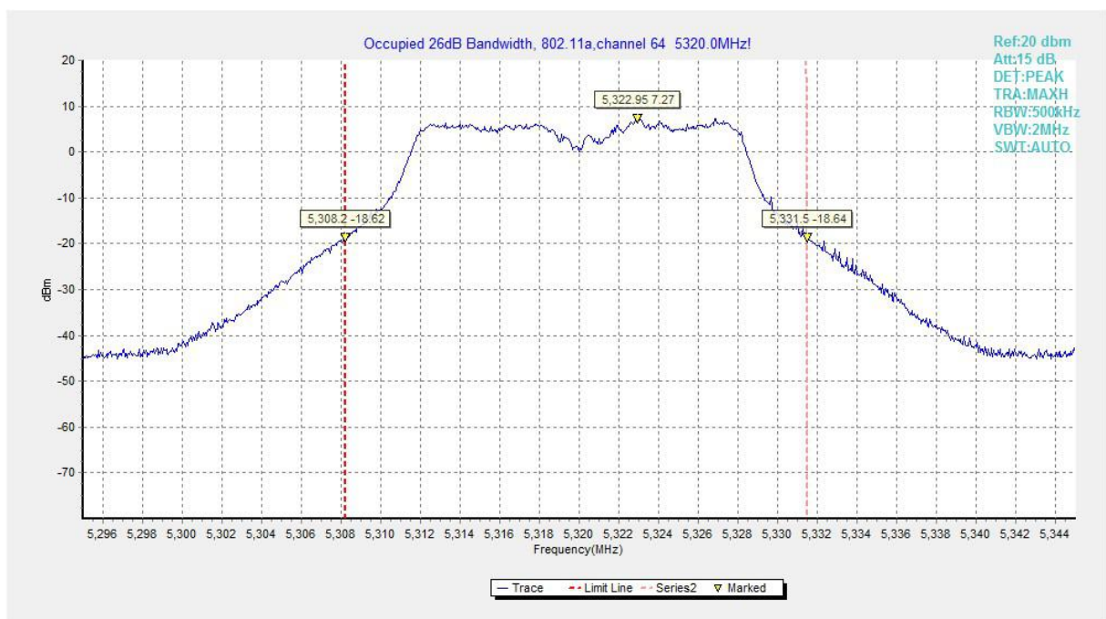
Fig.104 Occupied 26dB Bandwidth (802.11a, 5320MHz)
