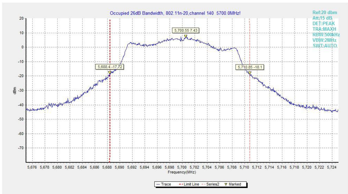
Fig.116 Occupied 26dB Bandwidth (802. 11n-HT20, 5700MHz)
