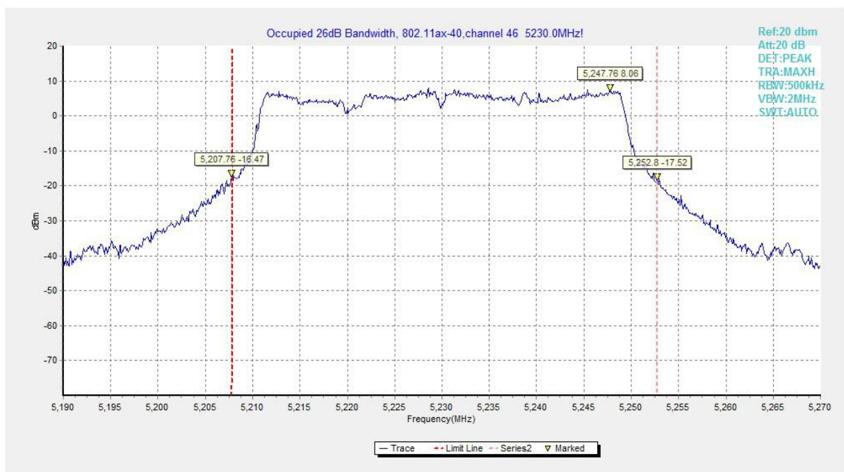
Fig.138 Occupied 26dB Bandwidth (802.11ax-HE40, 5230MHz)
