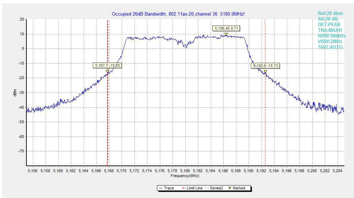
Fig.128 Occupied 26dB Bandwidth (802.11ax-HE20, 5180MHz)
