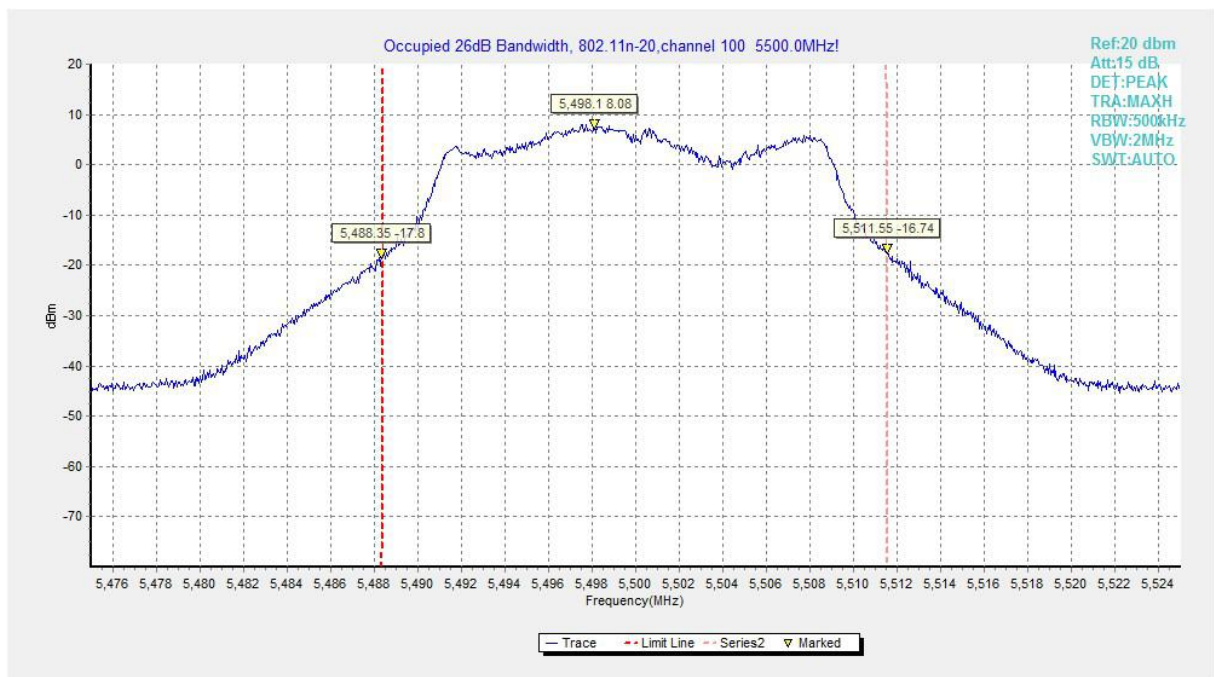
Fig.114 Occupied 26dB Bandwidth (802. 11n-HT20, 5500MHz)
