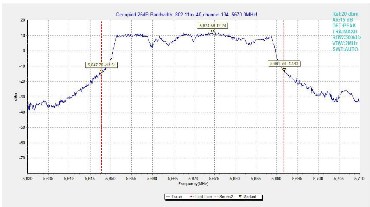
Fig.94 Occupied 26dB Bandwidth (802.11ax-HE40, 5670MHz)
