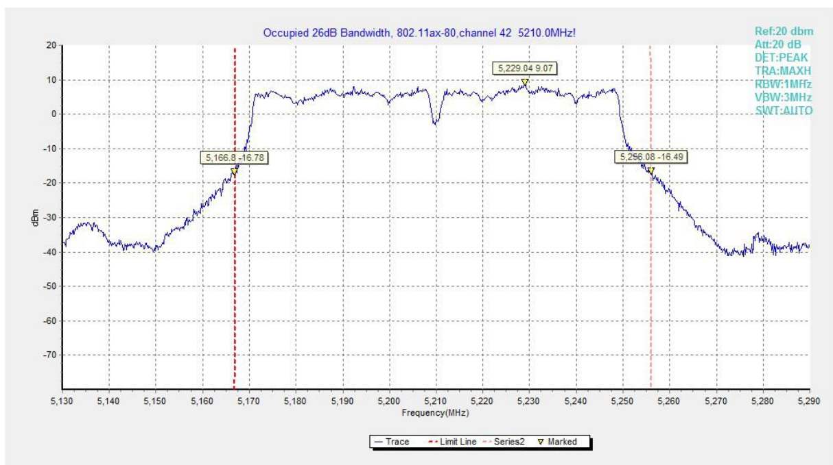
Fig.144 Occupied 26dB Bandwidth (802.11ax-HE80,5210MHz)
