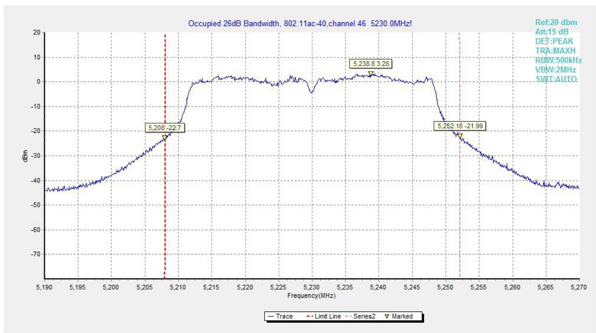
Fig.118 Occupied 26dB Bandwidth (802.11ac-HT40, 5230MHz)
