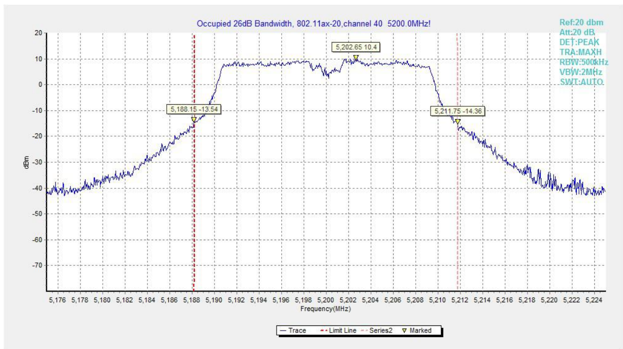
Fig.129 Occupied 26dB Bandwidth (802.11ax-HE20, 5200MHz)
