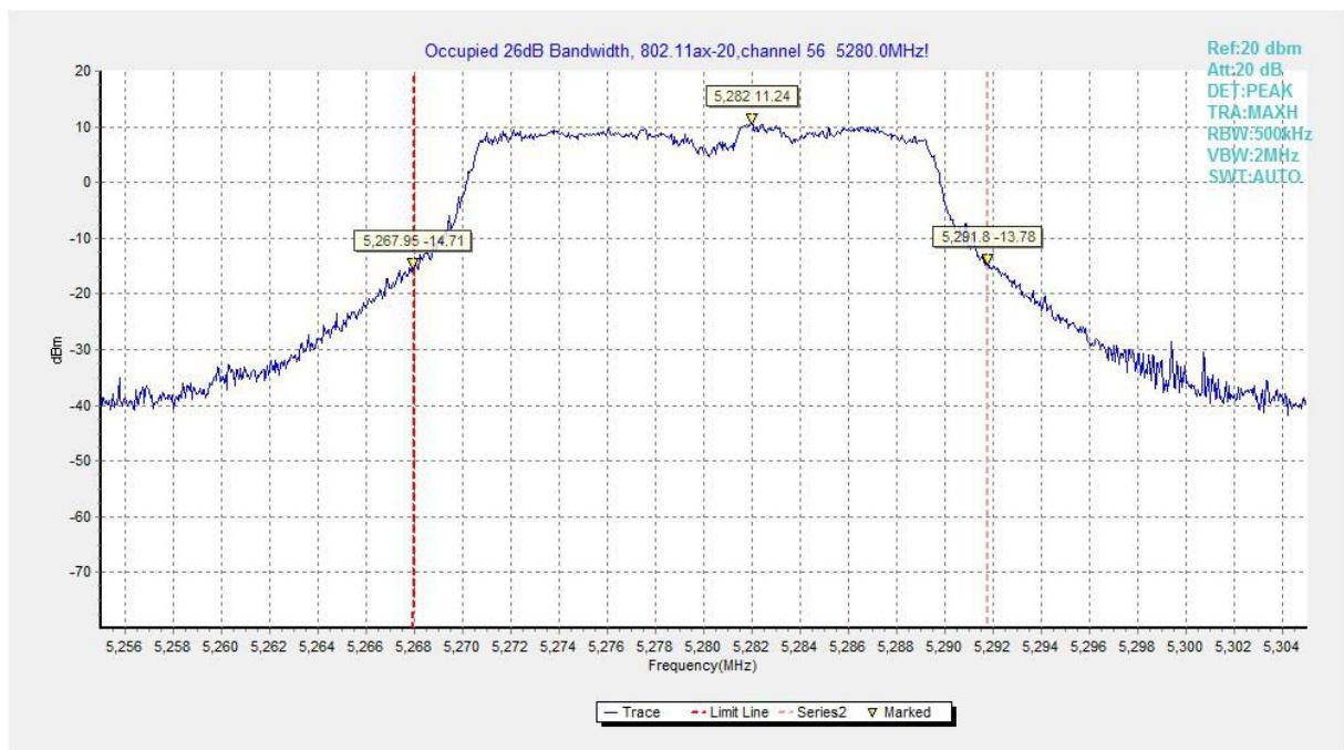
Fig.132 Occupied 26dB Bandwidth (802.11ax-HE20, 5280MHz)
