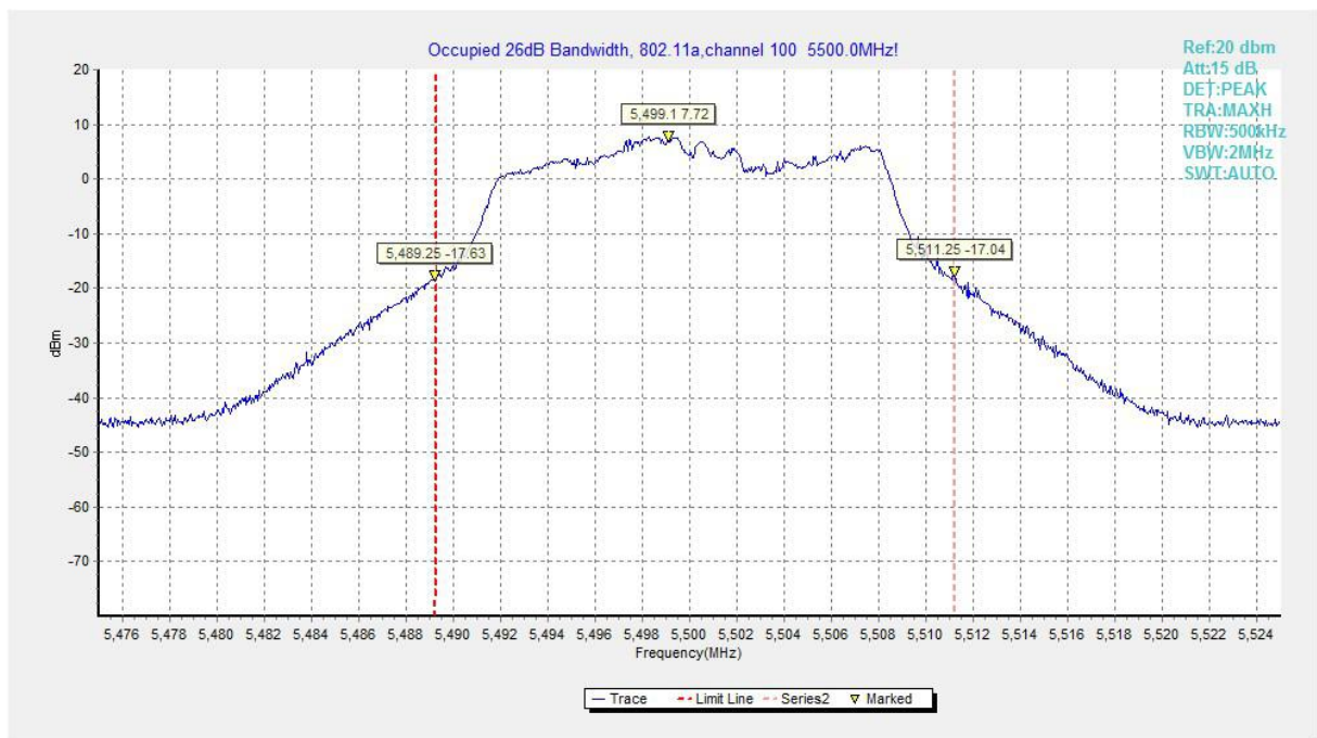
Fig.105 Occupied 26dB Bandwidth (802.11a, 5500MHz)
