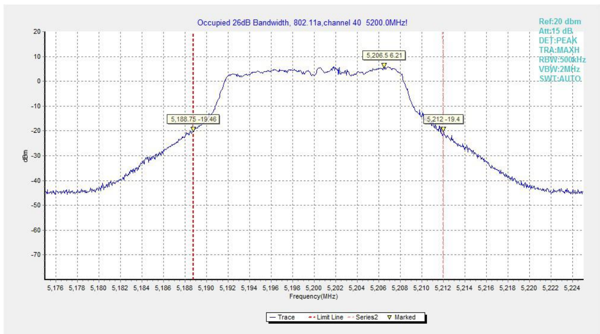
Fig.100 Occupied 26dB Bandwidth (802.11a, 5200MHz)
