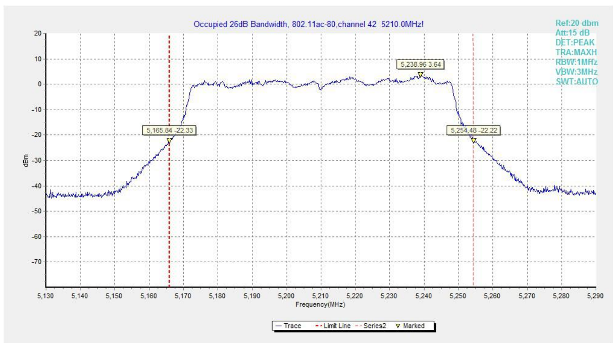
Fig.124 Occupied 26dB Bandwidth (802. 11ac-HT80, 5210MHz)
