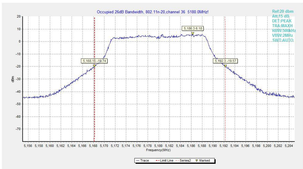
Fig.108 Occupied 26dB Bandwidth (802.11n-HT20, 5180MHz)
