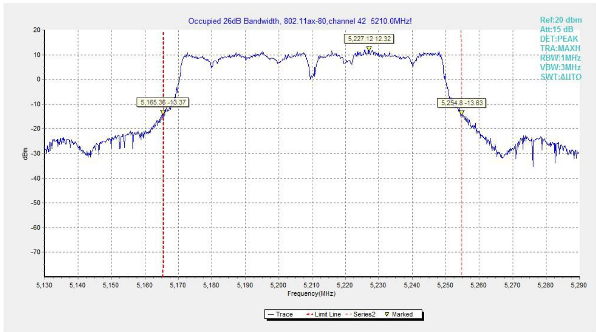
Fig.95 Occupied 26dB Bandwidth (802.11ax-HE80,5210MHz)
