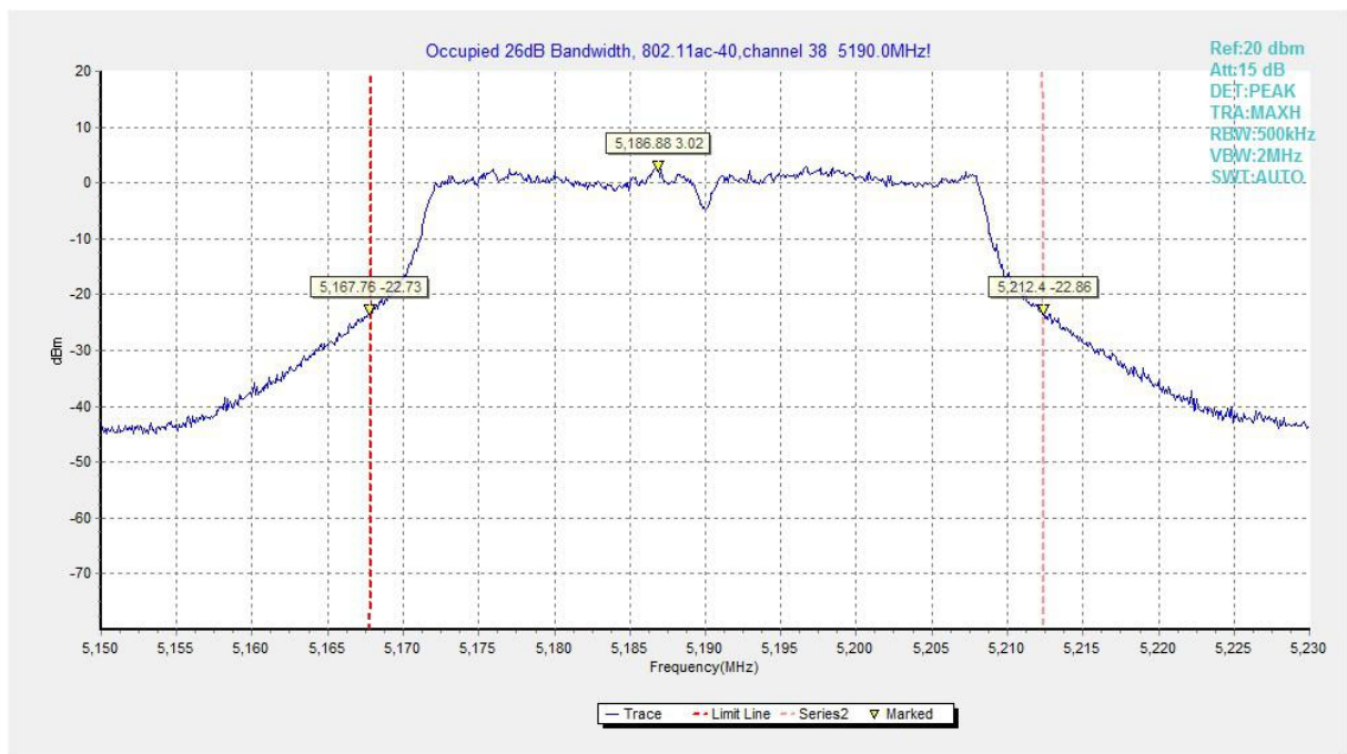
Fig.117 Occupied 26dB Bandwidth (802.11ac-HT40, 5190MHz)
