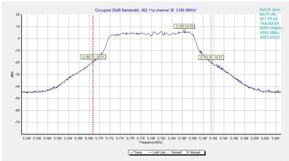
Fig.99 Occupied 26dB Bandwidth (802.11a, 5180MHz)
