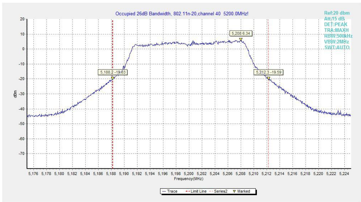
Fig.109 Occupied 26dB Bandwidth (802.11n-HT20, 5200MHz)
