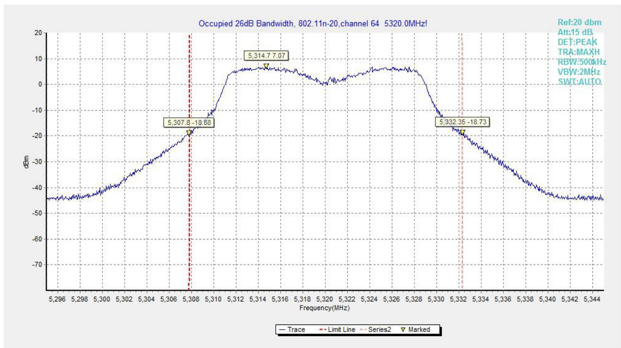
Fig.113 Occupied 26dB Bandwidth (802.11n-HT20, 5320MHz)
