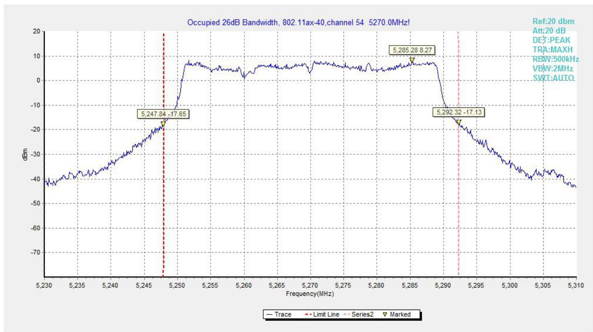
Fig.139 Occupied 26dB Bandwidth (802.11ax-HE40, 5270MHz)
