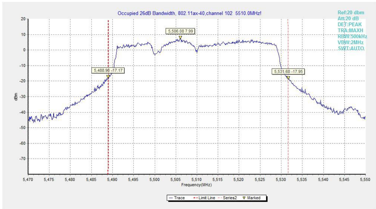
Fig.141 Occupied 26dB Bandwidth (802.11ax-HE40, 5510MHz)
