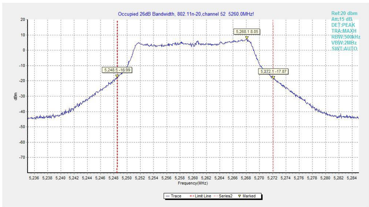
Fig.111 Occupied 26dB Bandwidth (802.11n-HT20, 5260MHz)
