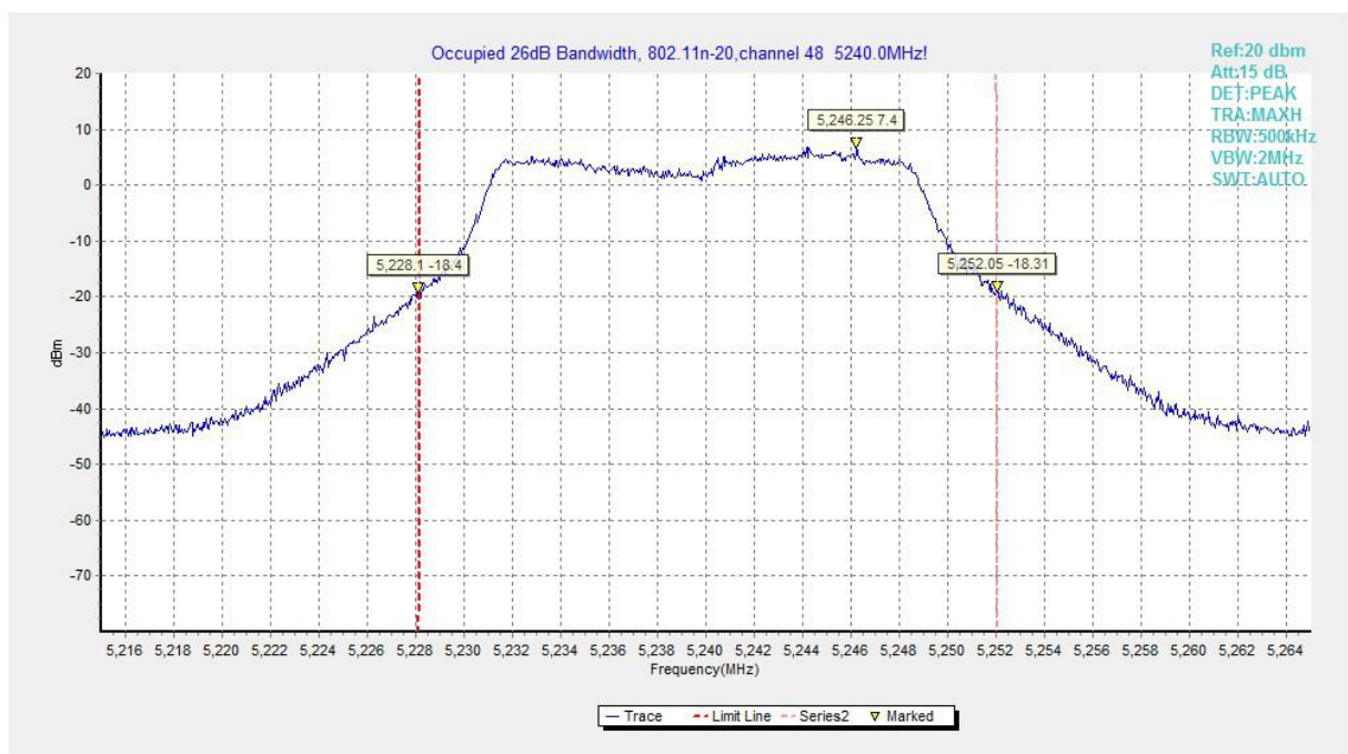
Fig.110 Occupied 26dB Bandwidth (802.11n-HT20, 5240MHz)
