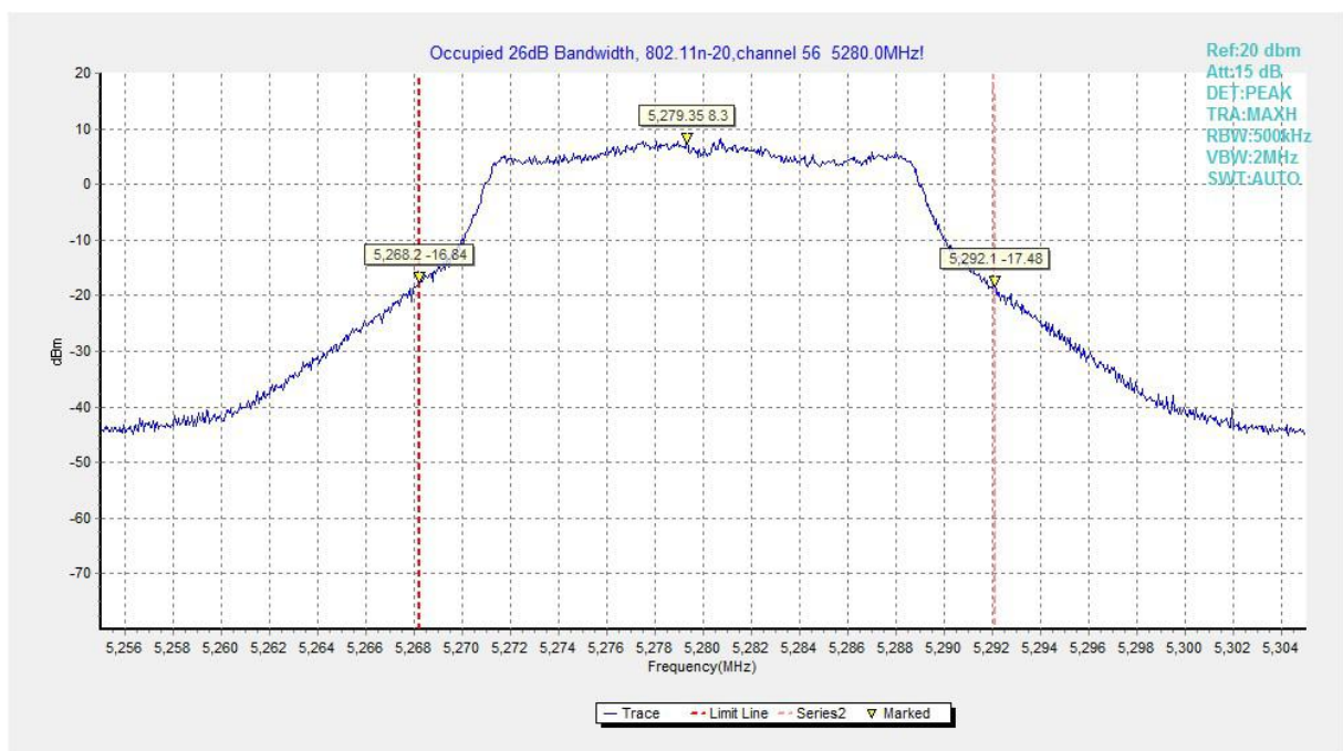
Fig.112 Occupied 26dB Bandwidth (802.11n-HT20, 5280MHz)
