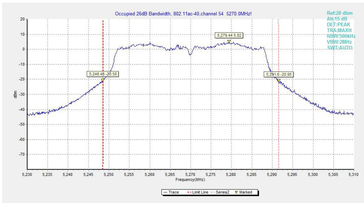
Fig.119 Occupied 26dB Bandwidth (802.11ac-HT40, 5270MHz)
