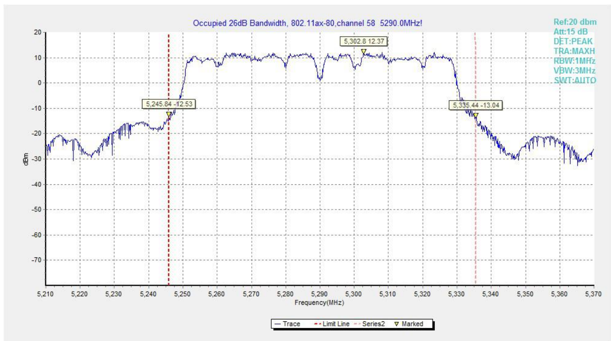
Fig.96 Occupied 26dB Bandwidth (802.11ax-HE80, 5290MHz)
