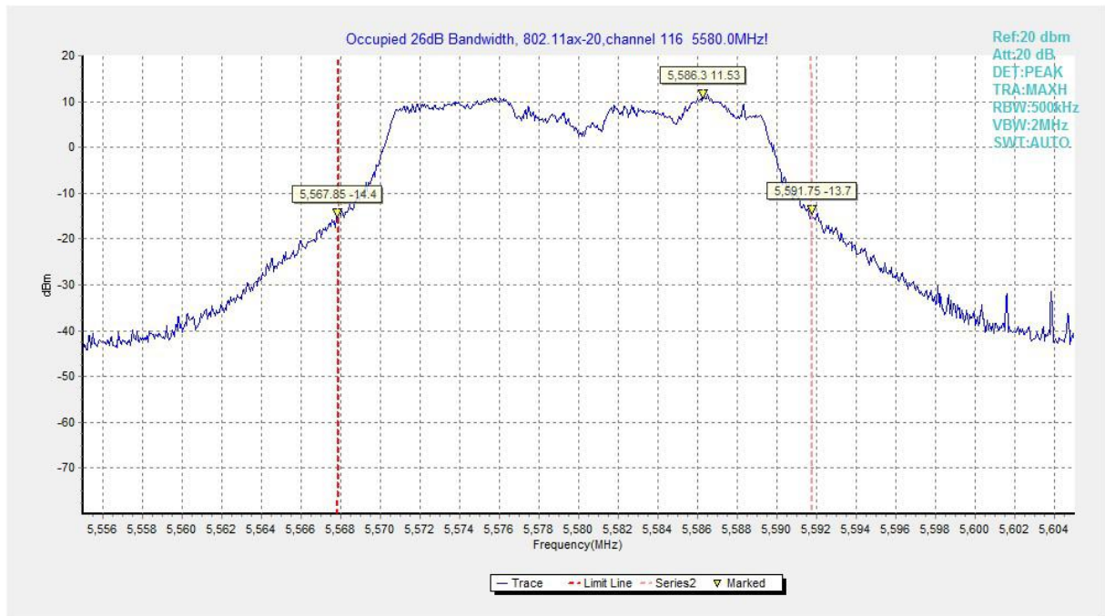
Fig.135 Occupied 26dB Bandwidth (802.11ax-HE20, 5580MHz)
