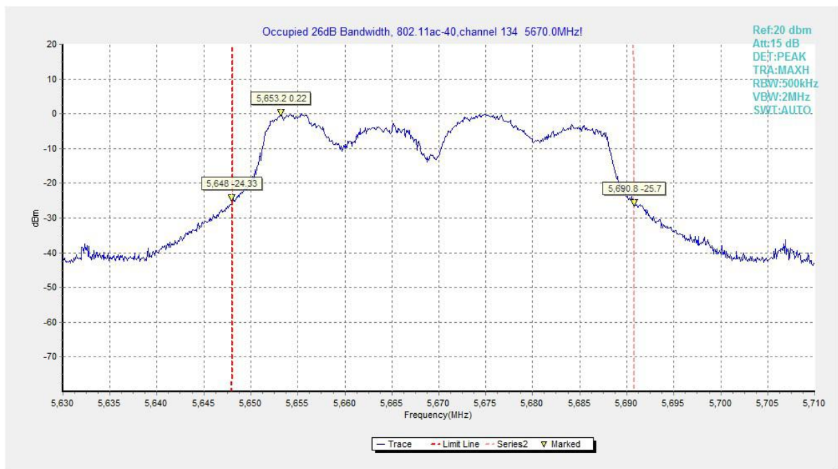
Fig.123 Occupied 26dB Bandwidth (802.11ac-HT40, 5670MHz)
