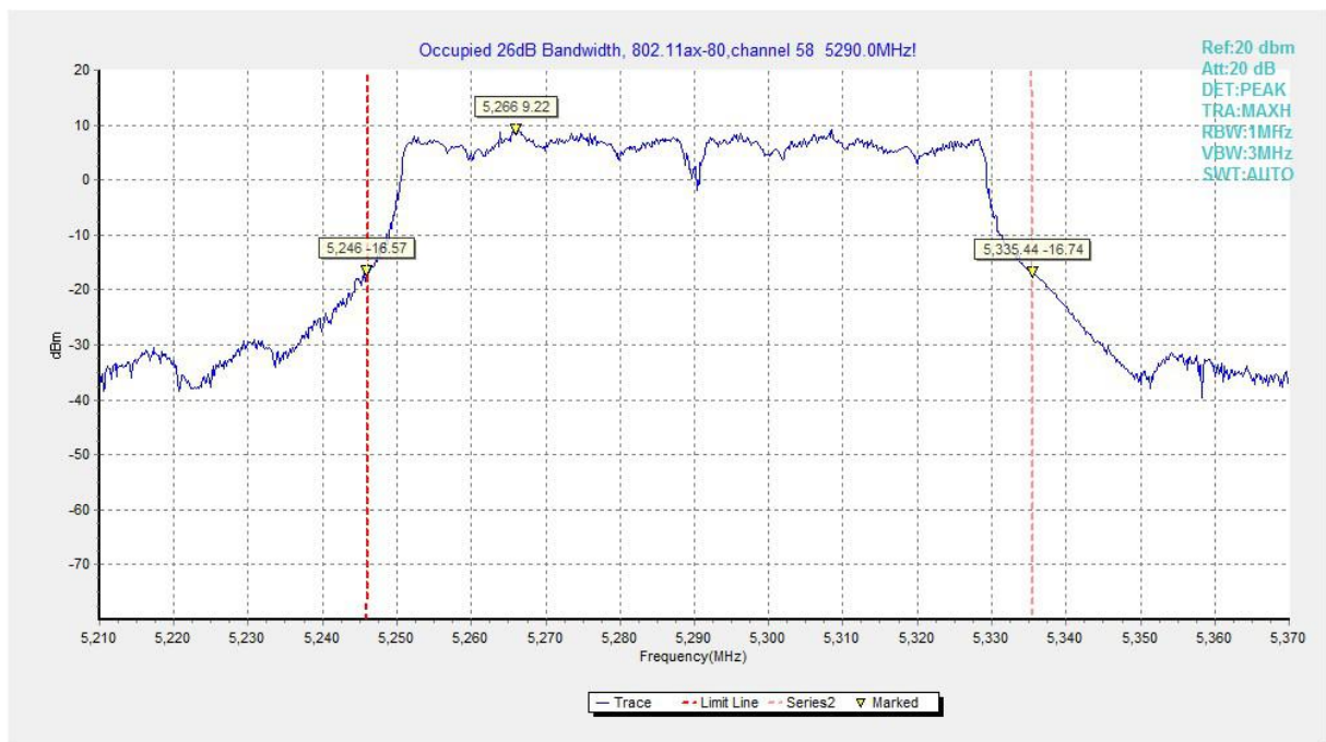
Fig.145 Occupied 26dB Bandwidth (802.11ax-HE80, 5290MHz)
