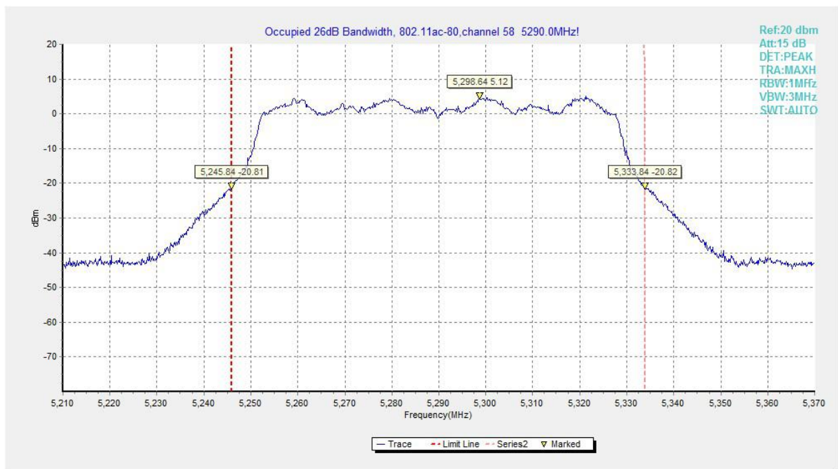
Fig.125 Occupied 26dB Bandwidth (802. 11ac-HT80, 5290MHz)
