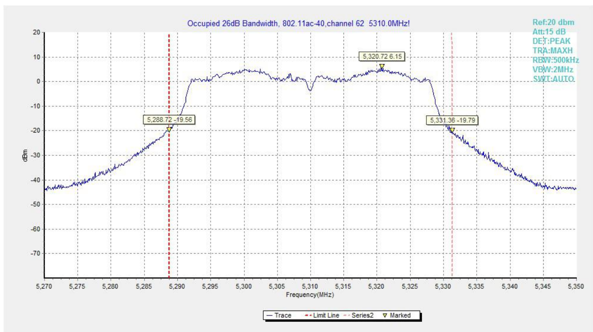
Fig.120 Occupied 26dB Bandwidth (802.11ac-HT40, 5310MHz)
