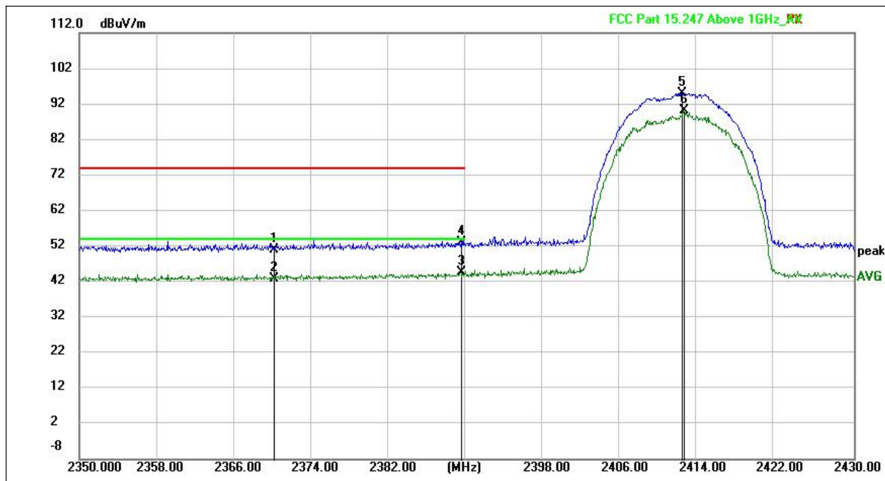
(802.11b _2412MHz, Antenna Horizontal)
