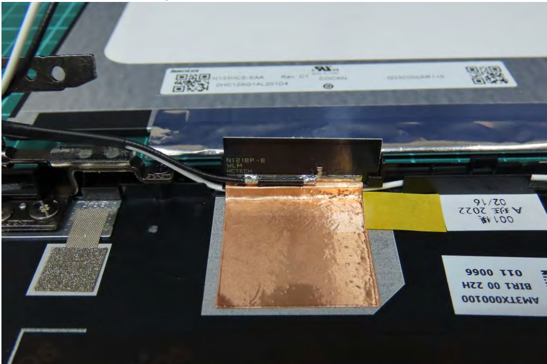
(30) EUT Photo - Antenna: High-Tek Electronics Co., Ltd.
