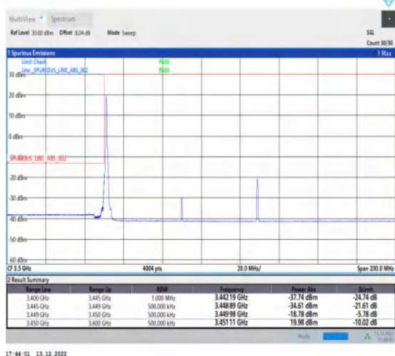
1-N77-3450-3550-30-80-L-4-CP-QPSK-Edge_1RB_Lef t-1@0-Ant1-1--PASS-see graph
