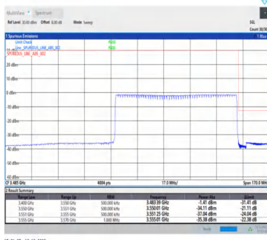
1-N77-3450-3550-30-80-H-6-CP-QPSK-Outer_Full -217@0-Ant1-1--PASS-see graph
