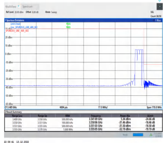
1-N77-3450-3550-30-10-H-6-CP-QPSK-Outer_Full -24@0-Ant1-1--PASS-see graph
