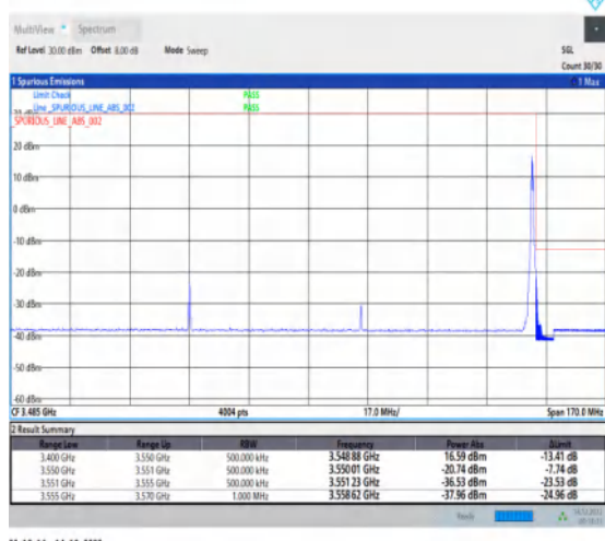
1-N77-3450-3550-30-100-H-5-CP-QPSK-Edge_1RB_R ight-1@272-Ant1-1--PASS-see graph
