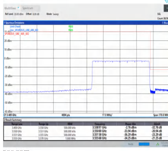
1-N77-3450-3550-30-60-H-6-CP-QPSK-Outer_Full -162@0-Ant1-1--PASS-see graph
