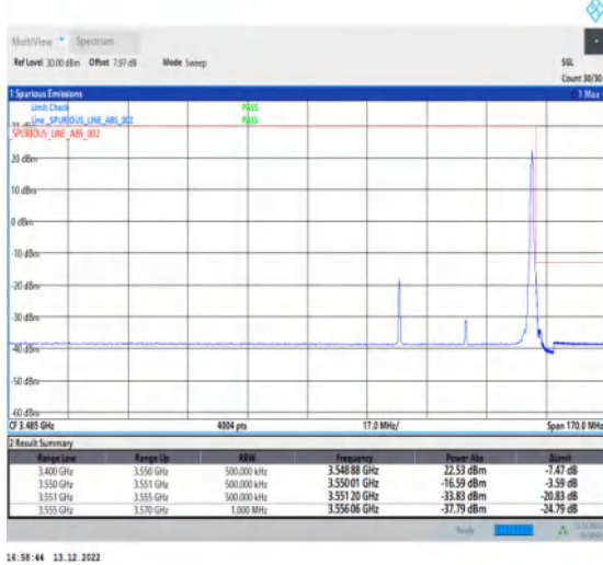
1-N77-3450-3550-30-40-H-2-DFT-PI2BPSK-Edge_1R B_Right-1@105-Ant1-1--PASS-see graph
