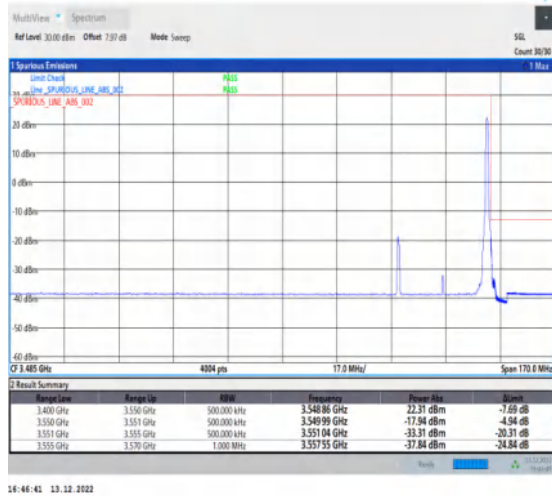
1-N77-3450-3550-30-30-H-2-DFT-PI2BPSK-Edge_1R B_Right-1@77-Ant1-1--PASS-see graph
