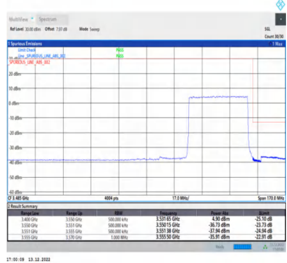
1-N77-3450-3550-30-40-H-3-DFT-PI2BPSK-Outer _Full-100@0-Ant1-1--PASS-see graph
