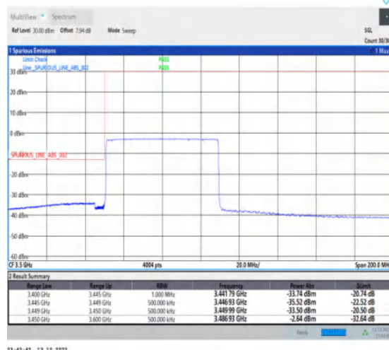
1-N77-3450-3550-30-60-L-6-CP-QPSK-Outer_Full -162@0-Ant1-1--PASS-see graph
