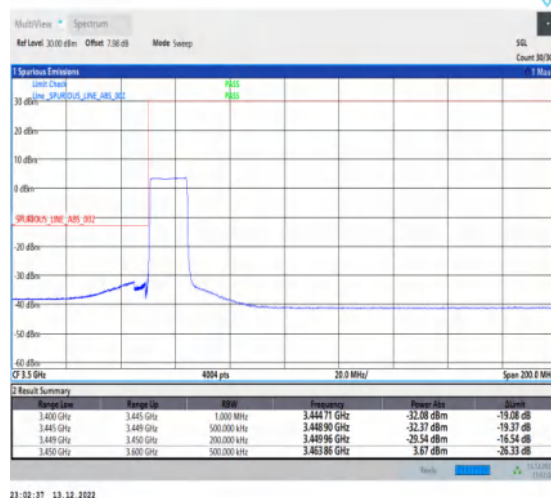
1-N77-3450-3550-30-15-L-6-CP-QPSK-Outer_Full -38@0-Ant1-1--PASS-see graph
