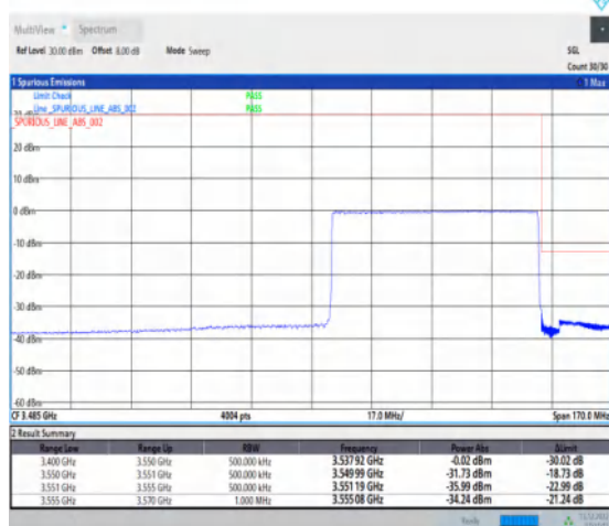
1-N77-3450-3550-30-60-H-6-CP-QPSK-Outer_Full -162@0-Ant1-1--PASS-see graph
