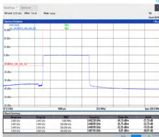
1-N77-3450-3550-30-60-L-6-CP-QPSK-Outer_Full -162@0-Ant1-1--PASS-see graph
