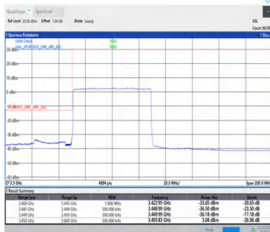
1-N77-3450-3550-30-60-L-3-DFT-PI2BPSK-Outer _Full-162@0-Ant1-1--PASS-see graph
