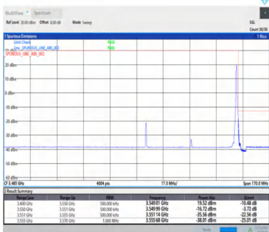
1-N77-3450-3550-30-60-H-5-CP-QPSK-Edge_1RB_Ri ght-1@161-Ant1-1--PASS-see graph
