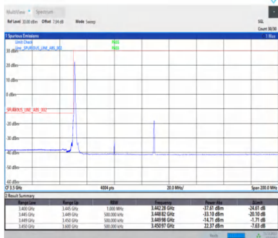
1-N77-3450-3550-30-60-L-1-DFT-PI2BPSK-Edge_1RB _Left-1@0-Ant1-1--PASS-see graph
