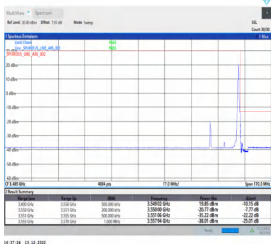
1-N77-3450-3550-30-20-H-5-CP-QPSK-Edge_1RB_Ri ght-1@50-Ant1-1--PASS-see graph
