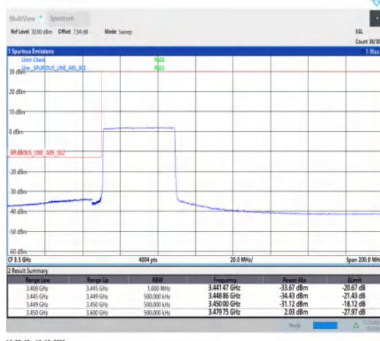
1-N77-3450-3550-30-40-L-6-CP-QPSK-Outer_Full -106@0-Ant1-1--PASS-see graph
