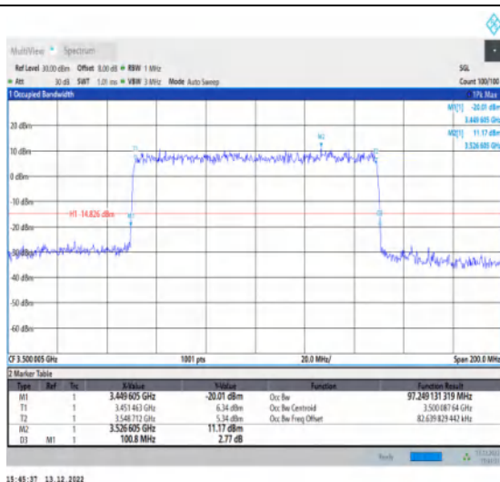
1-N77-3450-3550-30-100-L-7-CP-16QAM-Outer_Full -273@0-Ant1-97.249-100.800≤100-PASS
