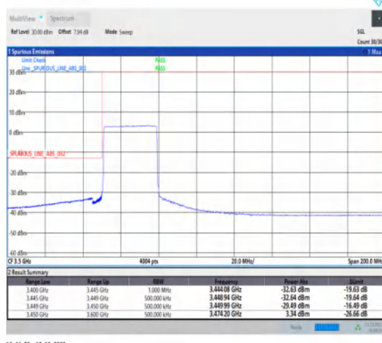
1-N77-3450-3550-30-30-L-6-CP-QPSK-Outer_Full -78@0-Ant1-1--PASS-see graph
