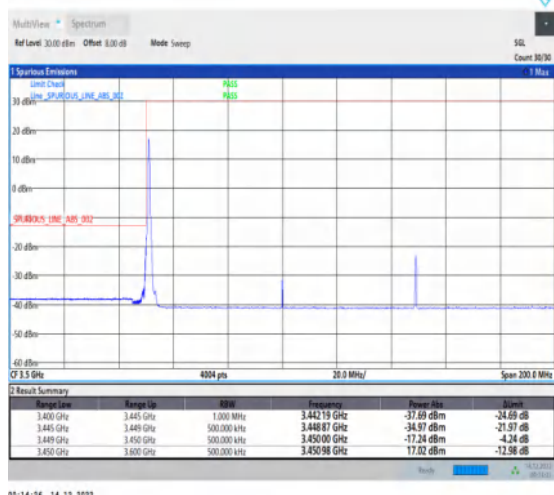
1-N77-3450-3550-30-100-L-4-CP-QPSK-Edge_1RB_L eft-1@0-Ant1-1--PASS-see graph
