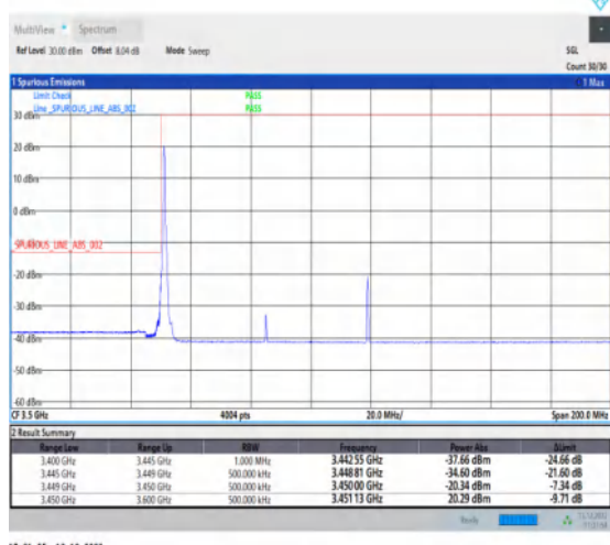
1-N77-3450-3550-30-70-L-4-CP-QPSK-Edge_1RB_Lef t-1@0-Ant1-1--PASS-see graph
