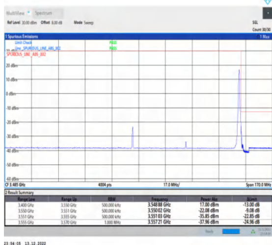
1-N77-3450-3550-30-70-H-5-CP-QPSK-Edge_1RB_Ri ght-1@188-Ant1-1--PASS-see graph
