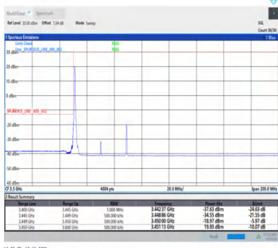
1-N77-3450-3550-30-40-L-4-CP-QPSK-Edge_1RB_Lef t-1@0-Ant1-1--PASS-see graph
