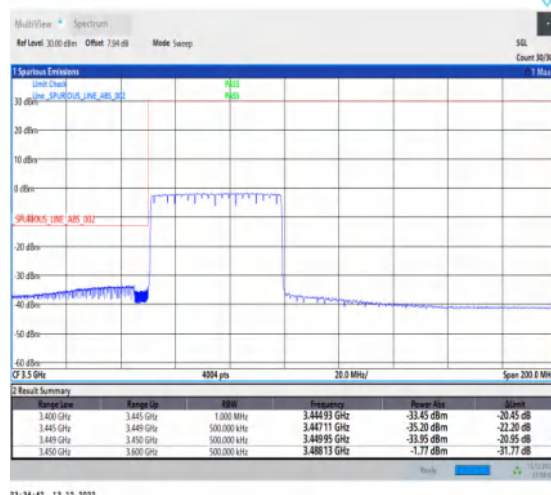
1-N77-3450-3550-30-50-L-6-CP-QPSK-Outer_Full -133@0-Ant1-1--PASS-see graph
