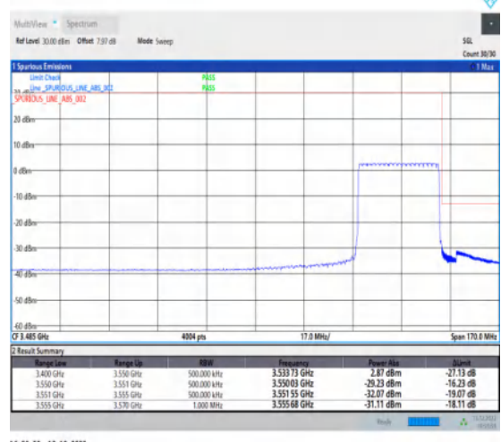
1-N77-3450-3550-30-30-H-6-CP-QPSK-Outer_Full -78@0-Ant1-1--PASS-see graph
