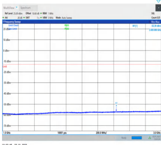
1-N77-3450-3550-30-100-M-1-DFT-QPSK-Edge_1R B_Left-1@0-1000-3000-Ant1-2925.40--52.39--13-PA SS
