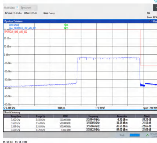
1-N77-3450-3550-30-70-H-6-CP-QPSK-Outer_Full -189@0-Ant1-1--PASS-see graph
