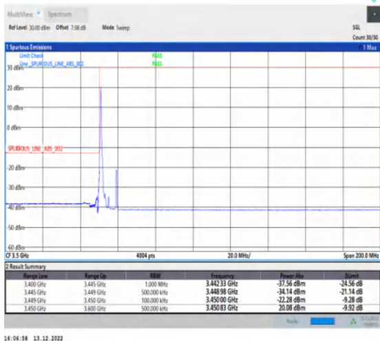
1-N77-3450-3550-30-10-L-4-CP-QPSK-Edge_1RB_Lef t-1@0-Ant1-1--PASS-see graph
