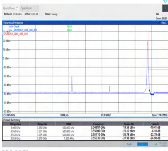
1-N77-3450-3550-30-80-H-5-CP-QPSK-Edge_1RB_Ri ght-1@216-Ant1-1--PASS-see graph
