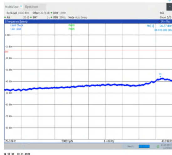
1-N77-3450-3550-30-100-M-1-DFT-QPSK-Edge_1R B_Left-1@0-26000-40000-Ant1-26000.00--42.55--13 -PASS
