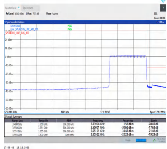
1-N77-3450-3550-30-40-H-6-CP-QPSK-Outer_Full -106@0-Ant1-1--PASS-see graph
