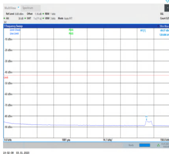
1-N77-3450-3550-30-100-M-1-DFT-QPSK-Edge_1R B_Left-1@0-0.009-0.15-Ant1-0.13--84.07--43-PASS
