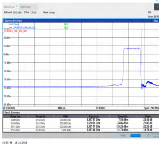
1-N77-3450-3550-30-20-H-3-DFT-PI2BPSK-Outer _Full-50@0-Ant1-1--PASS-see graph
