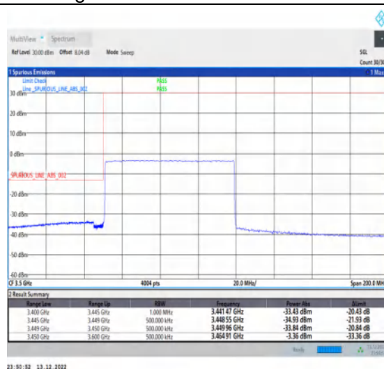
1-N77-3450-3550-30-70-L-6-CP-QPSK-Outer_Full -189@0-Ant1-1--PASS-see graph
