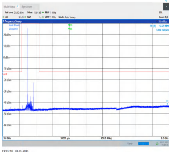
1-N77-3450-3550-30-100-L-1-DFT-QPSK-Edge_1R B_Left-1@0-3000-6000-Ant1-5914.65--42.24--13-PA SS
