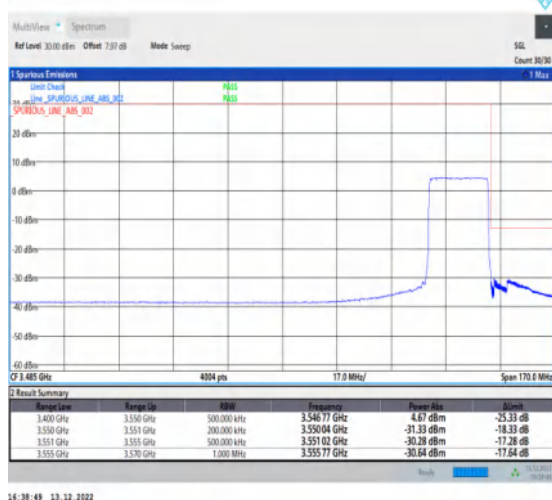
1-N77-3450-3550-30-20-H-6-CP-QPSK-Outer_Full -51@0-Ant1-1--PASS-see graph
