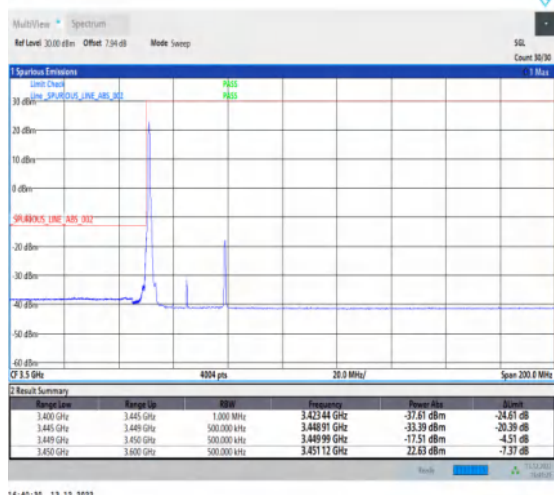
1-N77-3450-3550-30-30-L-1-DFT-PI2BPSK-Edge_1RB_Left-1@0-Ant1-1--PASS-see graph
